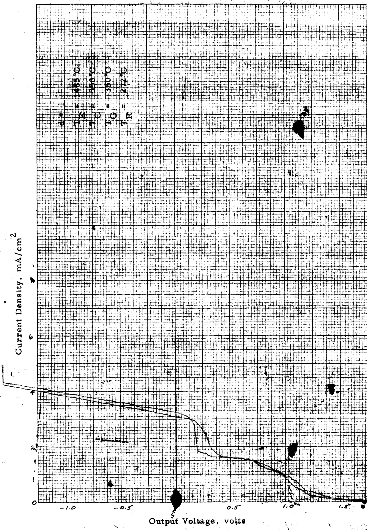
I-V Characteristics of RL6 Emitter
