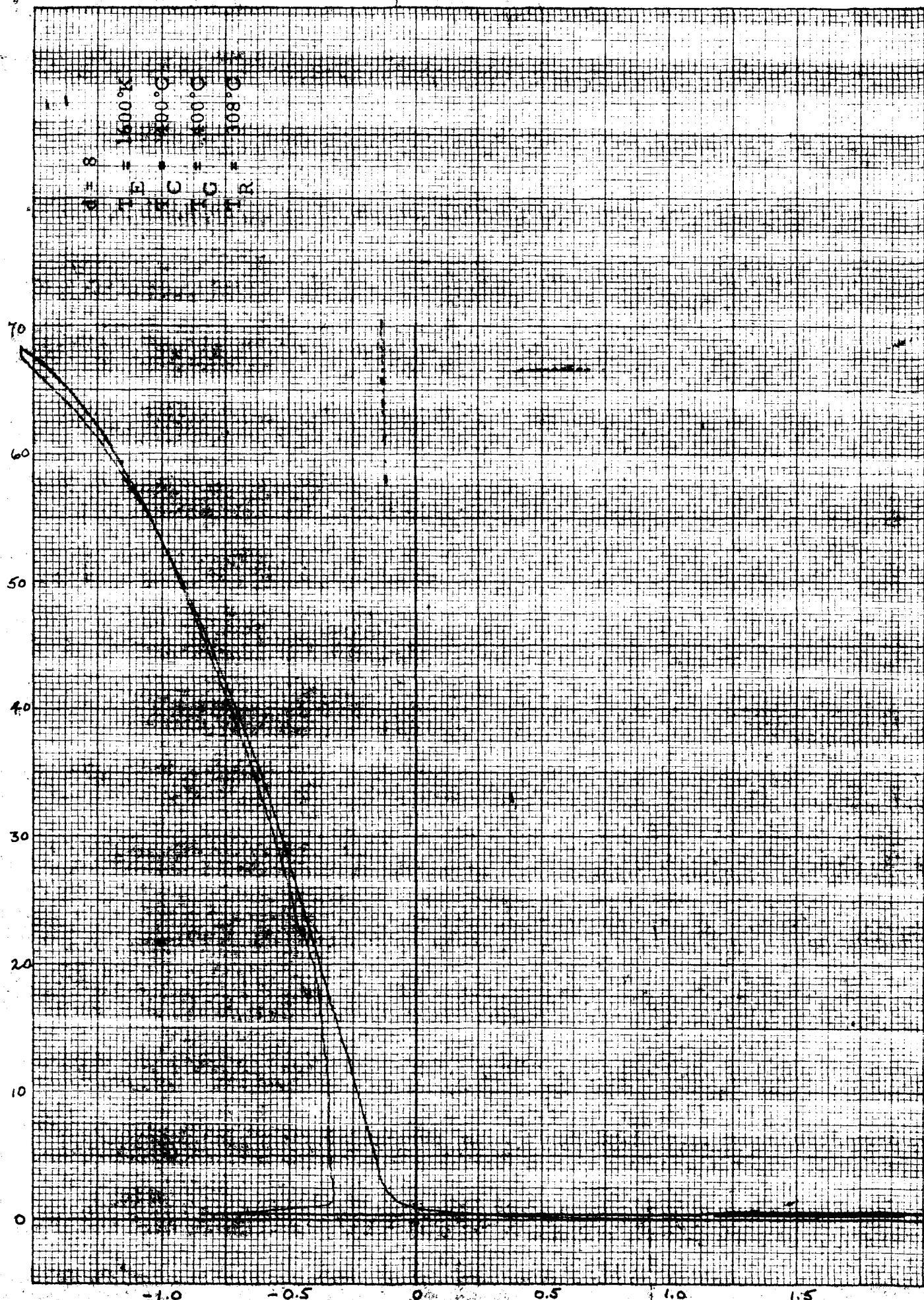
I-V Characteristics of RL6 Emitter
