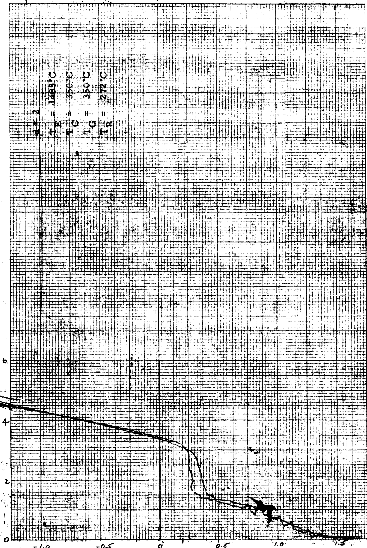
I-V Characteristics of R16 Emitter
