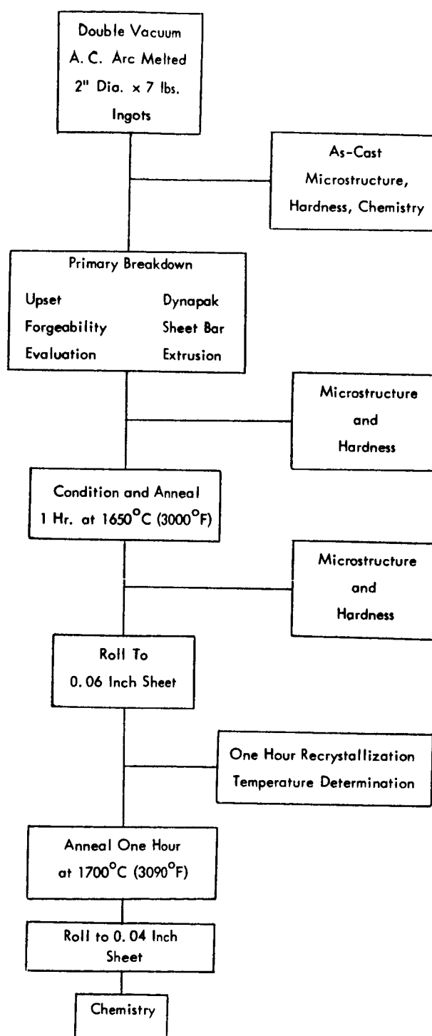
FIGURE 1 - Processing Schedule for Optimized Two Inch Diameter Ingot Compositions
