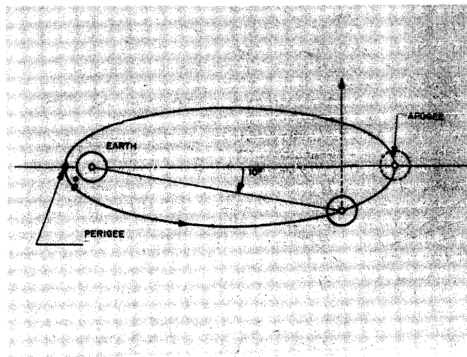
Fig. 4. Spacecraft trajectories
