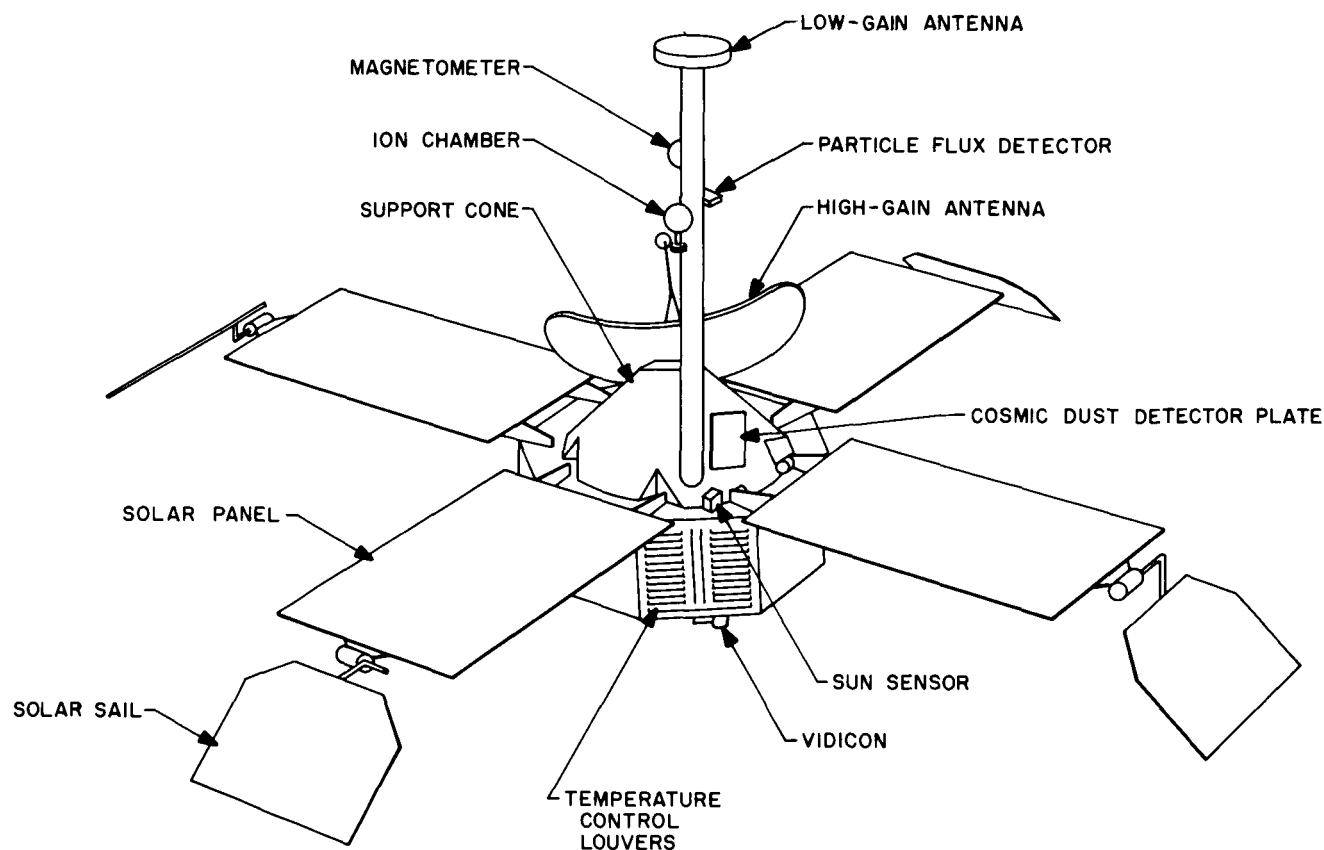
Fig. 3. Mariner spacecraft
