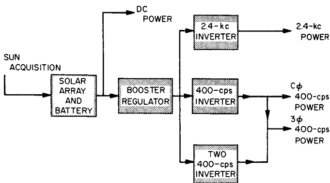
Fig. 8. Power supply
