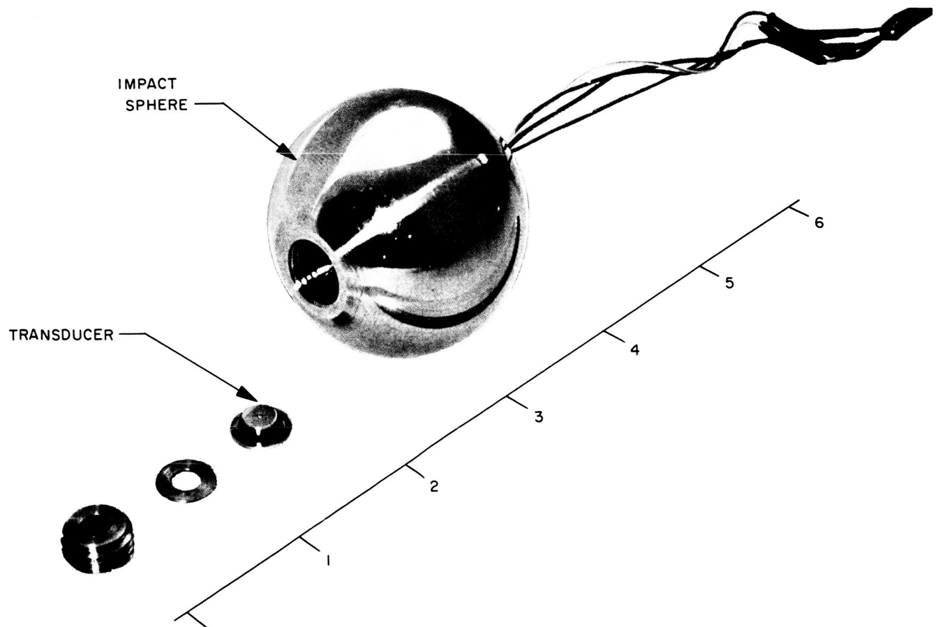
Fig. 9. Prototype accelerometer
