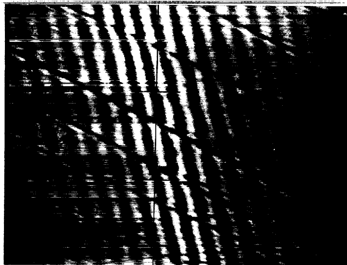
FIGURE 2.8 Interference Photo of Monomolecular Finish on 2024 Aluminum. Scale: 0.00194 inches between scale marks; 11.8 microinches between interference lines.
