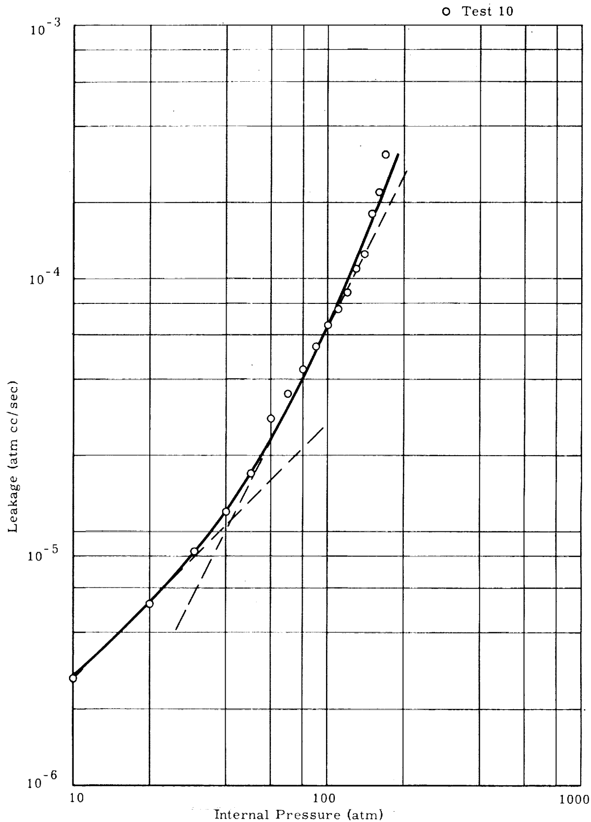
Figure 2. 73. Leakage as a Function of Internal Pressure, Phase II of Experiment - Jones Optical KANIGEN aluminum.
