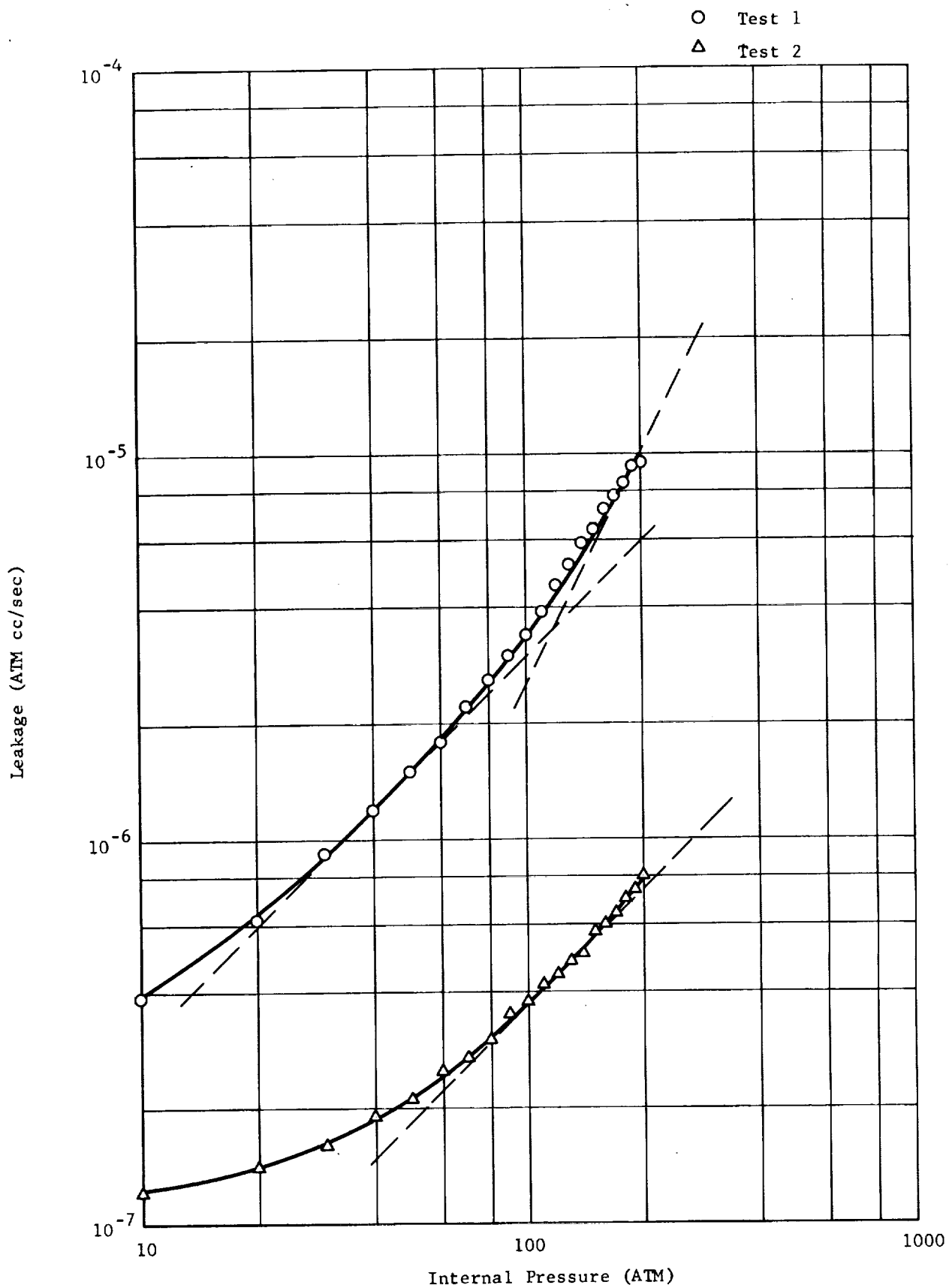
Figure 2. 74. Leakage as a Function of Internal Pressure, Phase II of Experiment - Stainless Steel-Silver Tests 2-83
