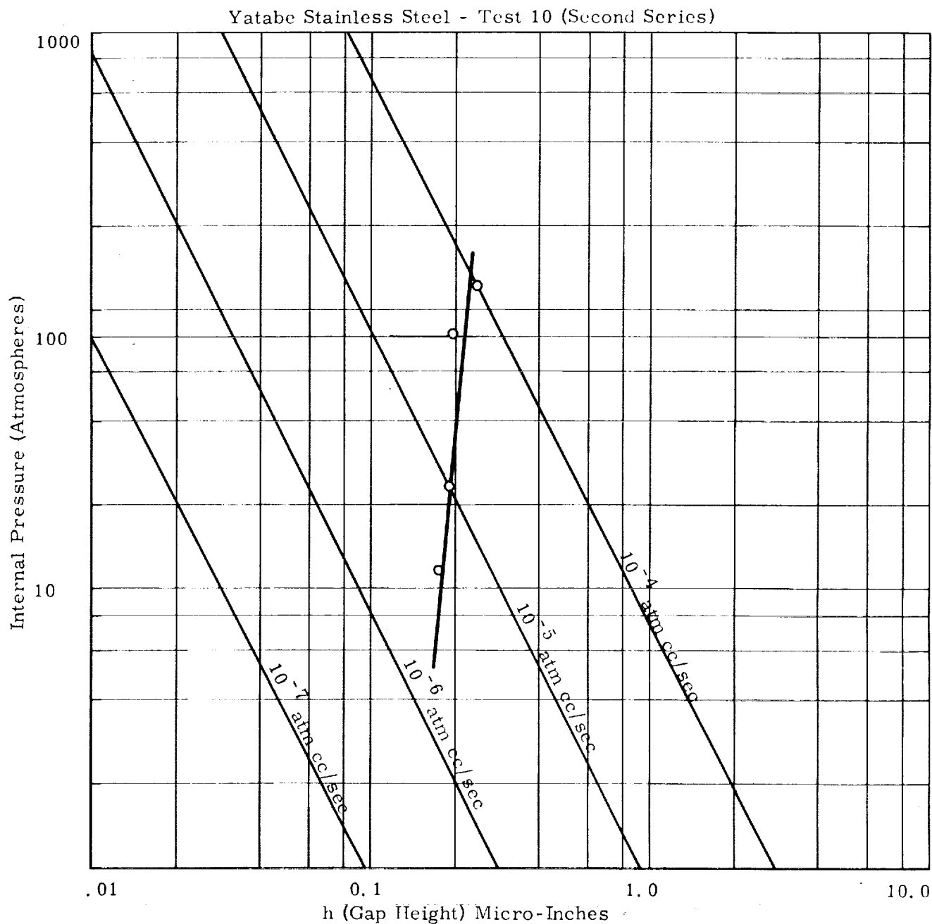
Figure 2.83. Leakage Rate for Helium at 20°C for an Annular Passage Equal to Experimental Nominal Dimensions, with 0 psi External Pressure. Comparison with Experimental Superfinished Surface Results.
