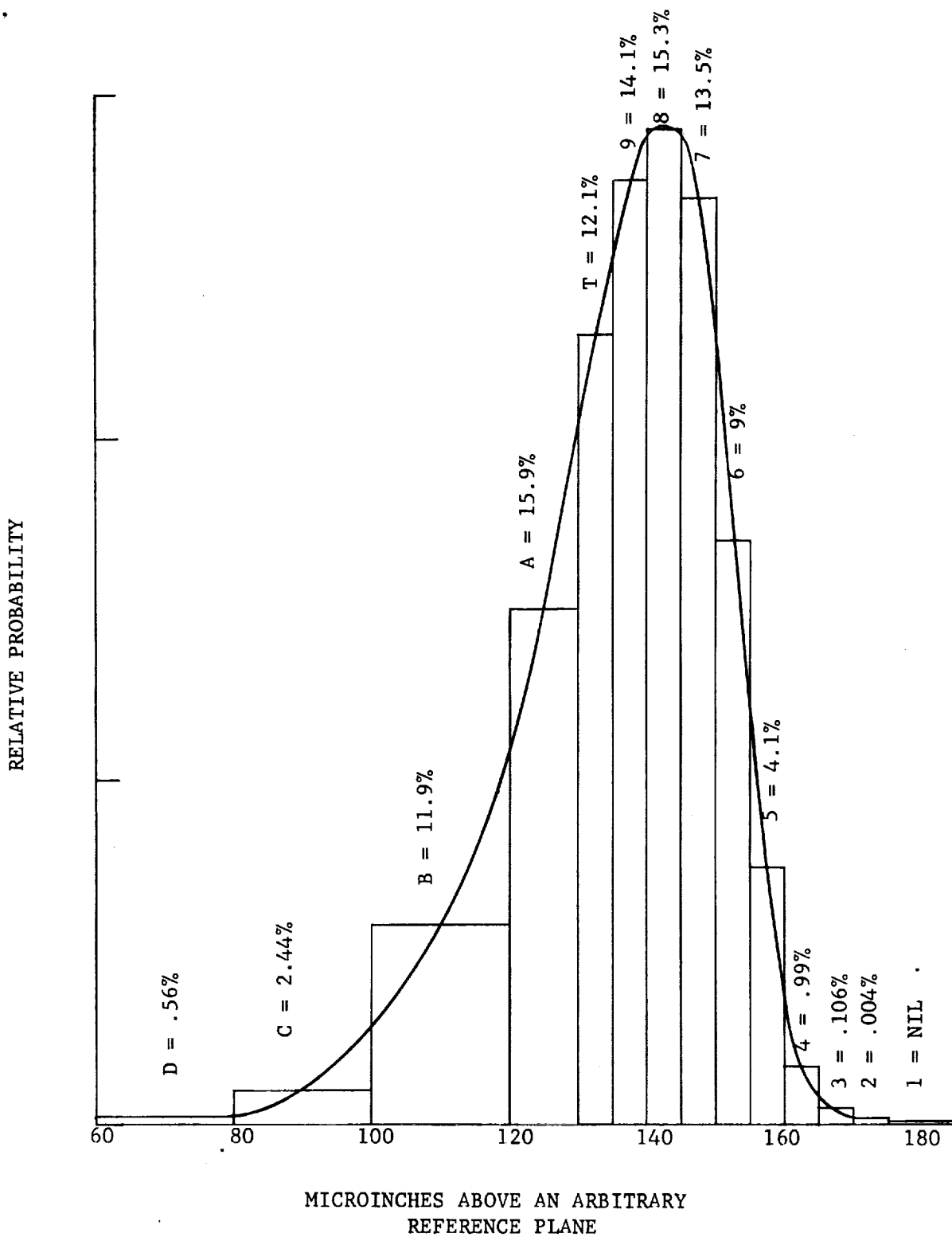
Figure 3.7. Distribution of Asperity Heights for a Lapped Surface
