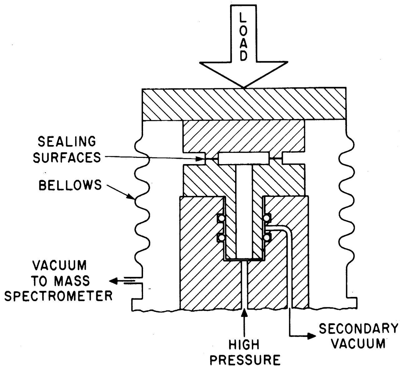
FIGURE 2.2 Schematic of Experimental Apparatus for Sealing Investigations.
