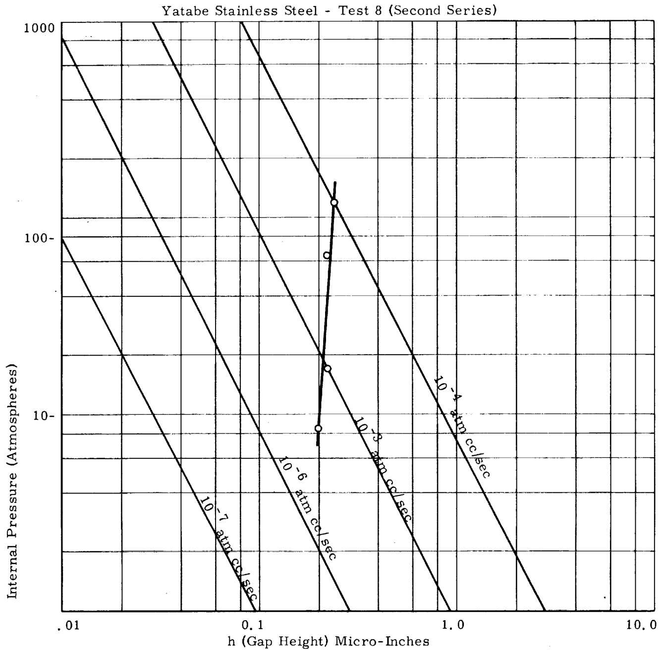
Figure 2.82. Leakage Rate for Helium at 20°C for an Annular Passage Equal to Experimental Nominal Dimensions, with 0 psi External Pressure. Comparison with Experimental Superfinished Surface Results.
