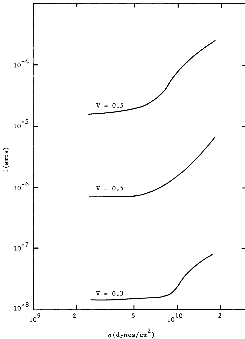
Fig. 28. Current vs Nominal Stress for a (111) Plane Planar Diode for Several Voltage Levels.
