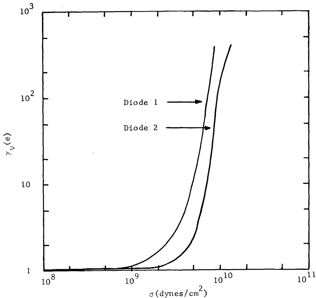
Fig. 22. \gamma_v(e) as a Function of Stress for Two Diodes Made on the Same (111) Wafer.
