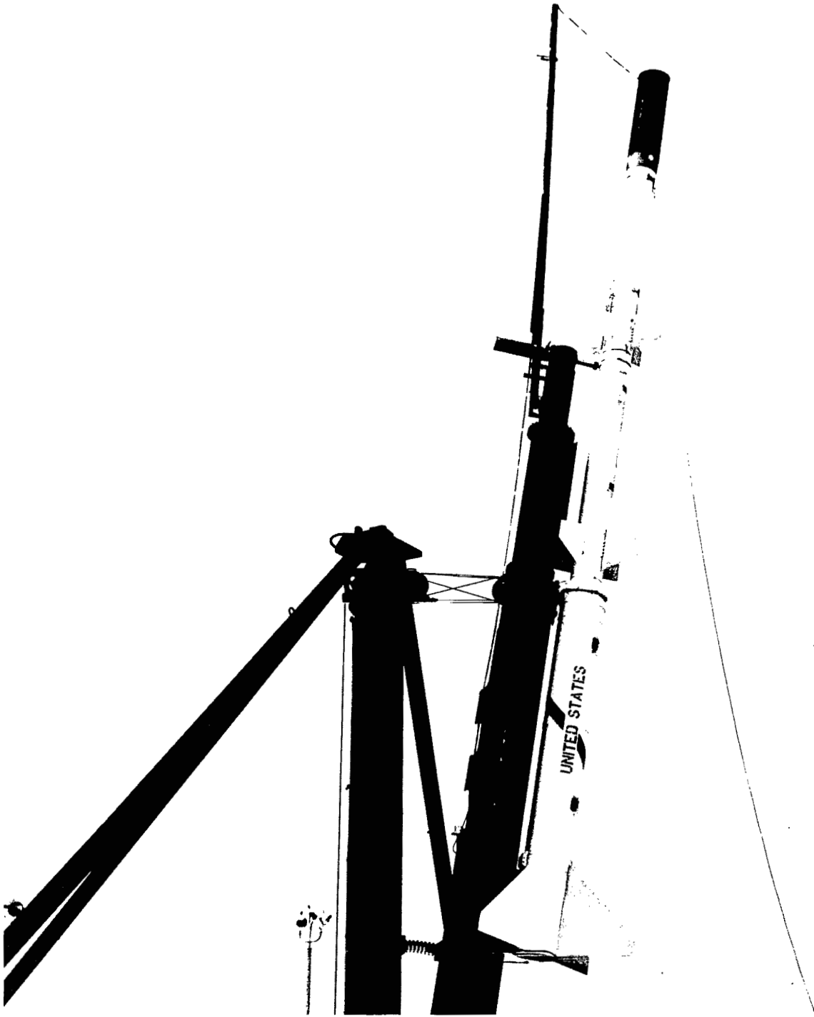
Figure 2.- Modified Javelin on launcher.
