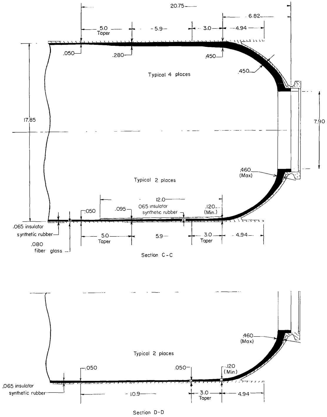
(e) Aft-chamber asbestos insulator.
