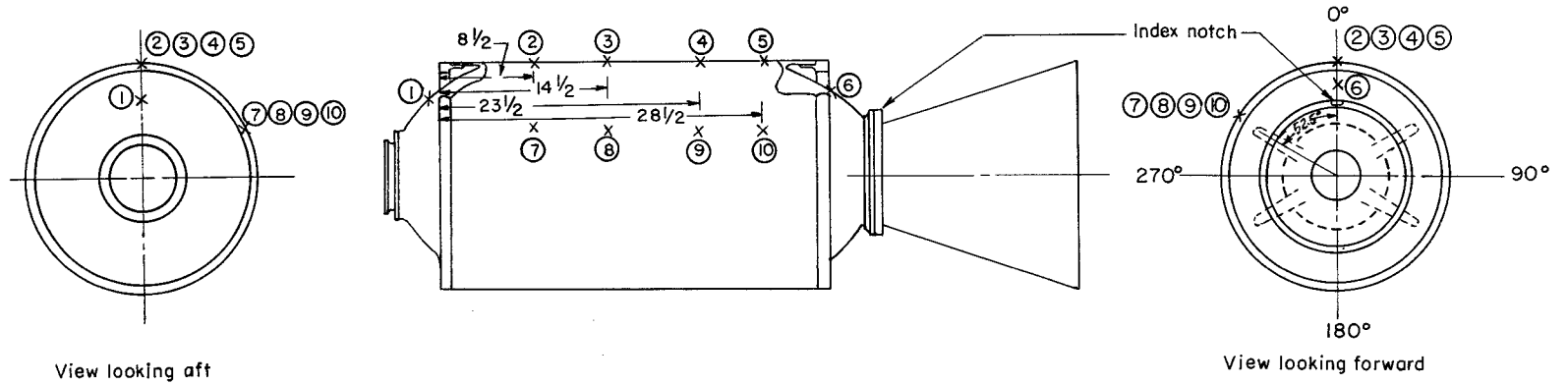
Figure 4.- Temperature-sensor locations. All dimensions are in inches.
