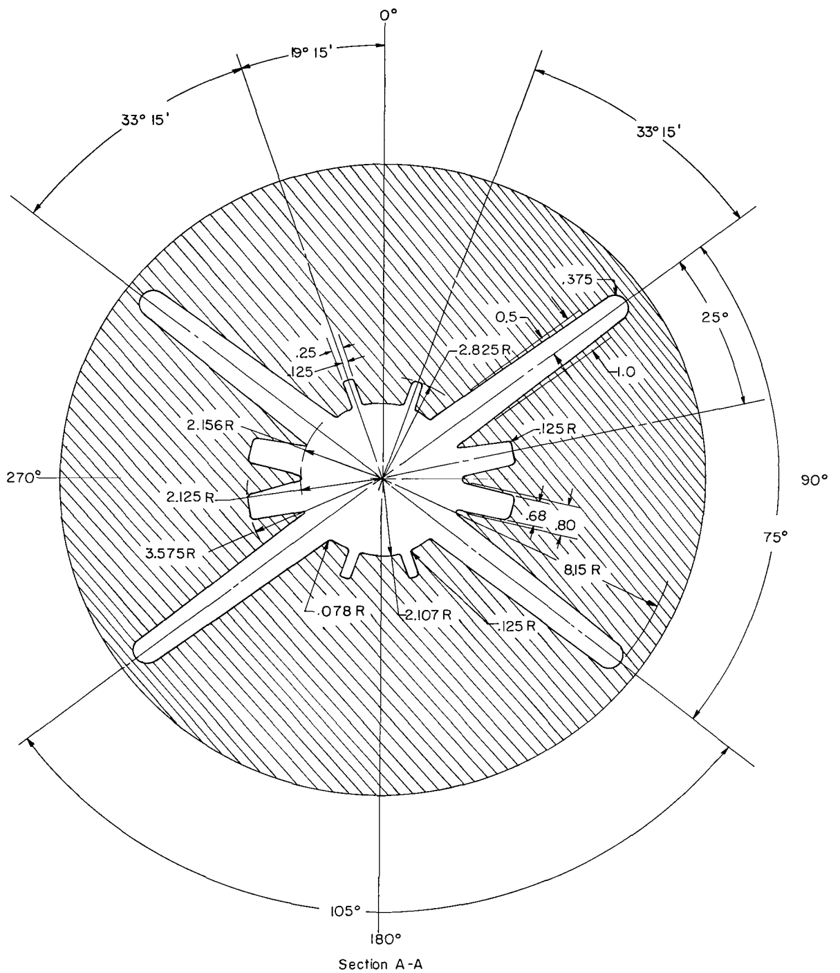
(b) Propellant core geometry.
