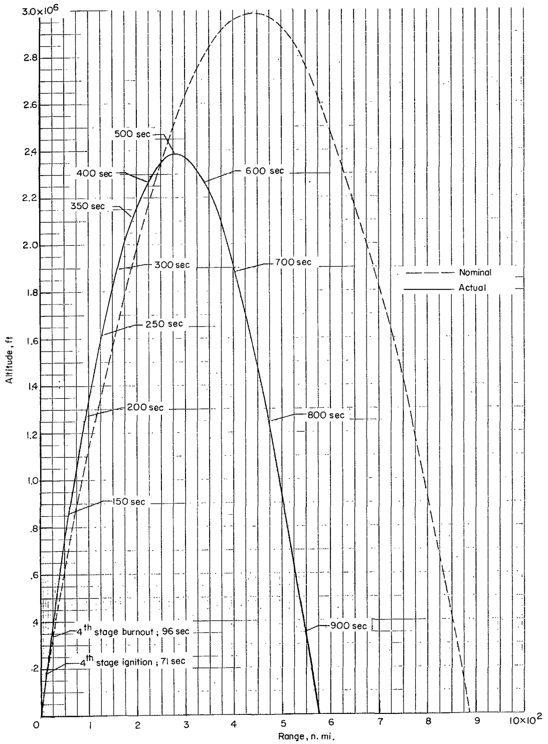
Figure 3.- Comparison of actual and nominal flight path.
