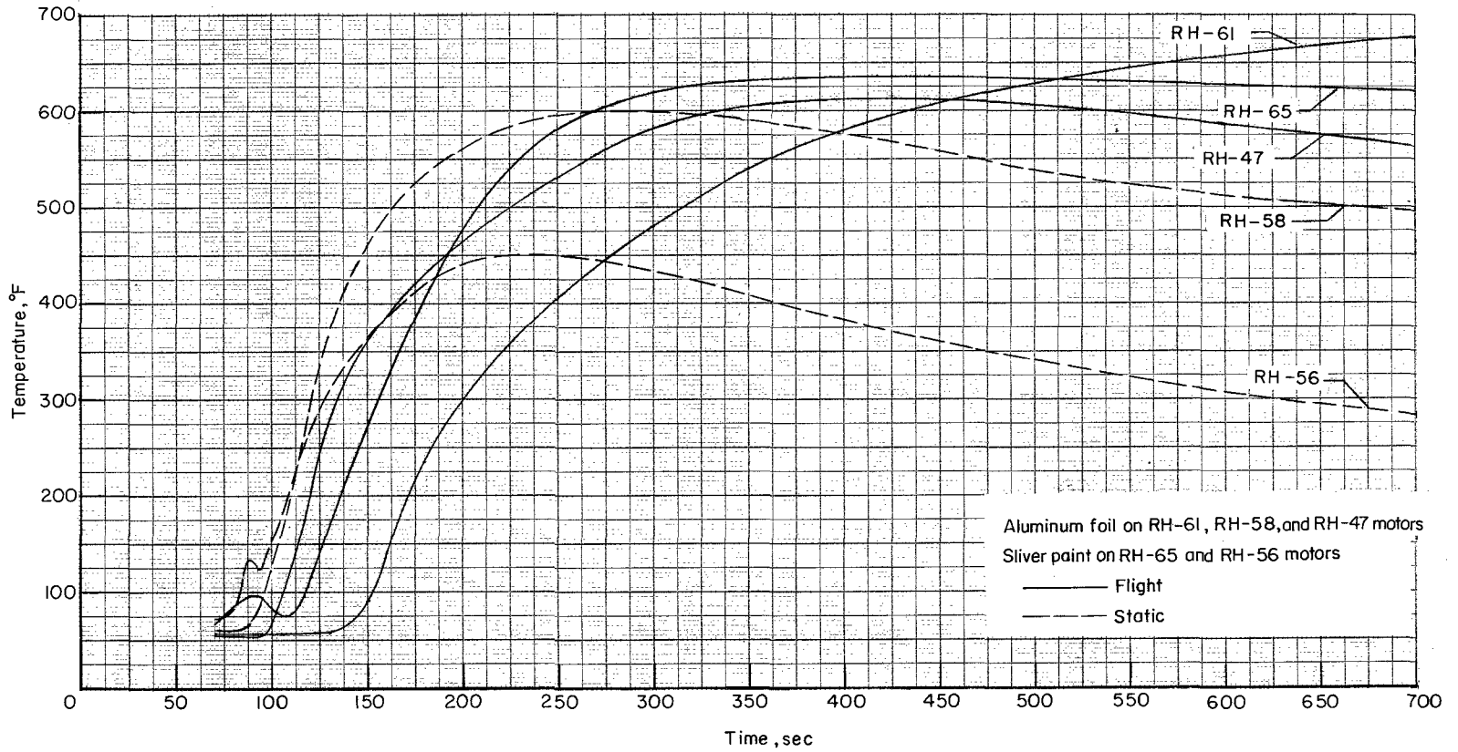
Figure 14.- Comparison of forward-dome temperatures from static and flight tests.
