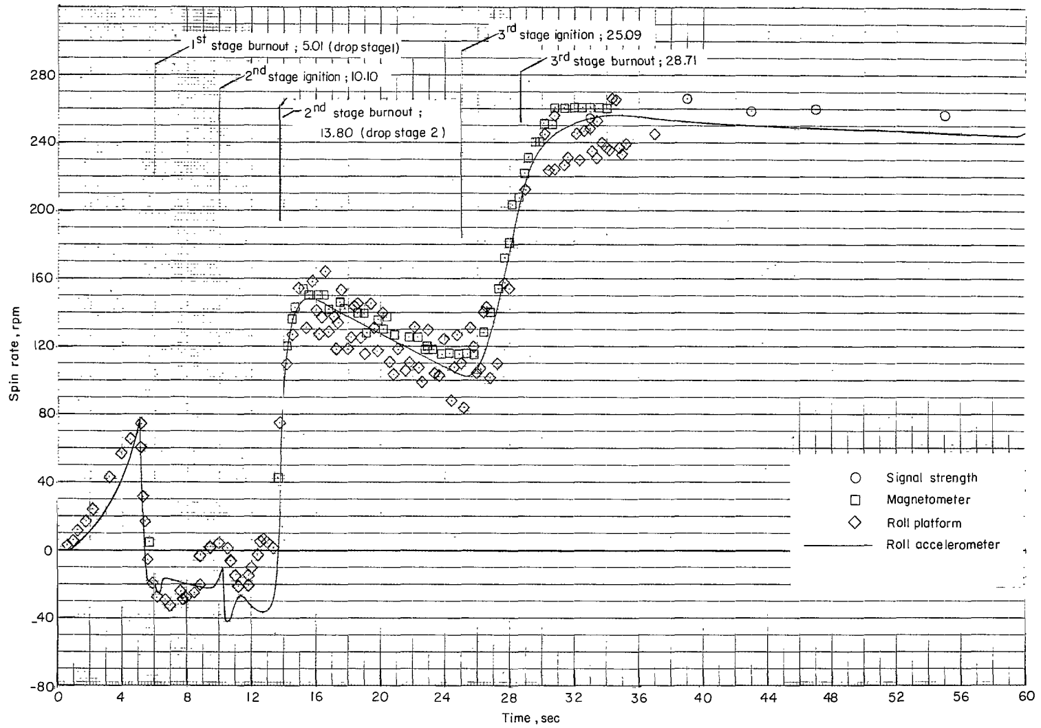
Figure 8.- Comparison of spin rate obtained from various sources.
