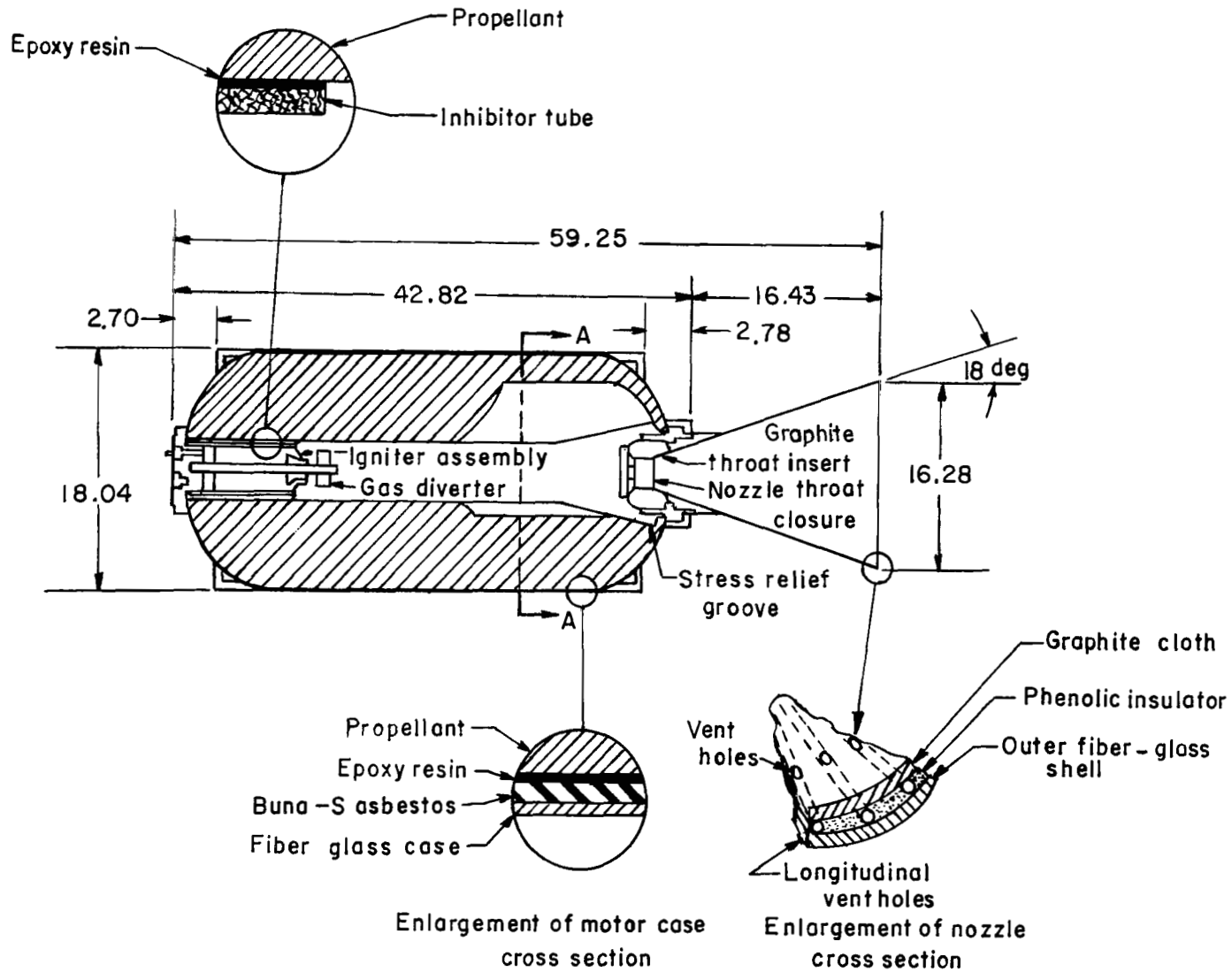
(a) Schematic. (See figure 1(b) for section A-A.)
