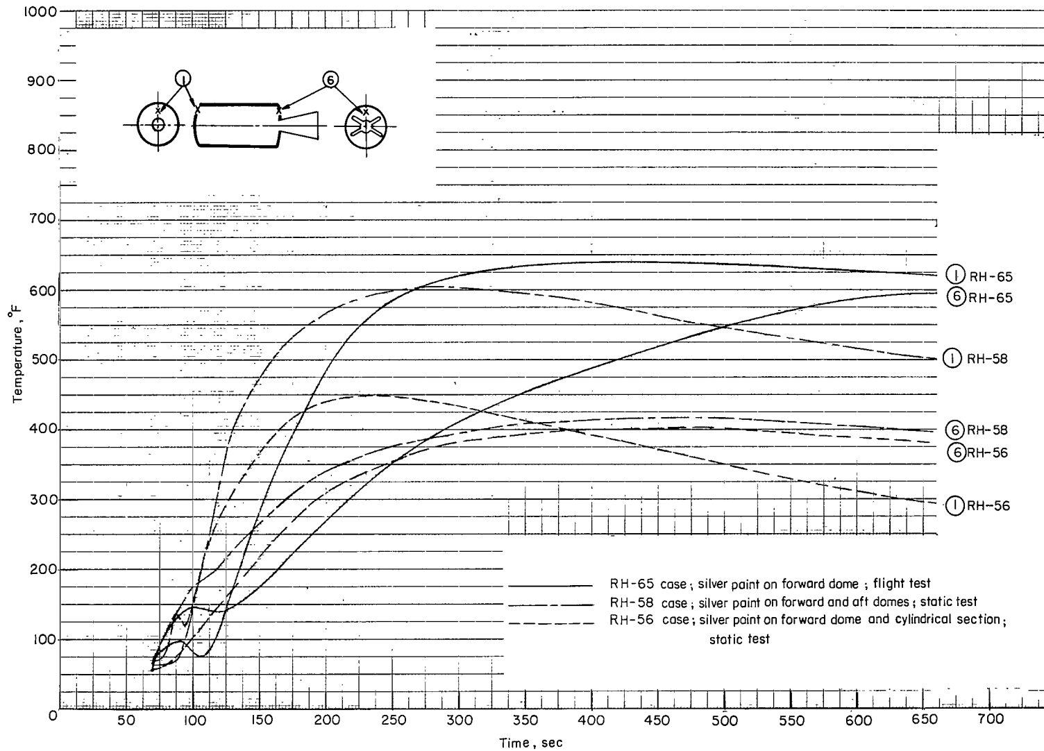
Figure 13.- Forward- and after-dome temperatures measured at thermocouples 1 and 6.
