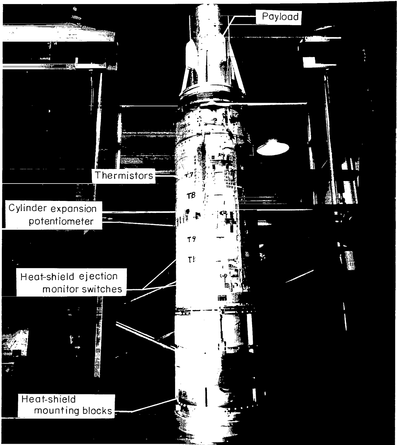
Figure 6.- Altair-II C1 payload stage.
