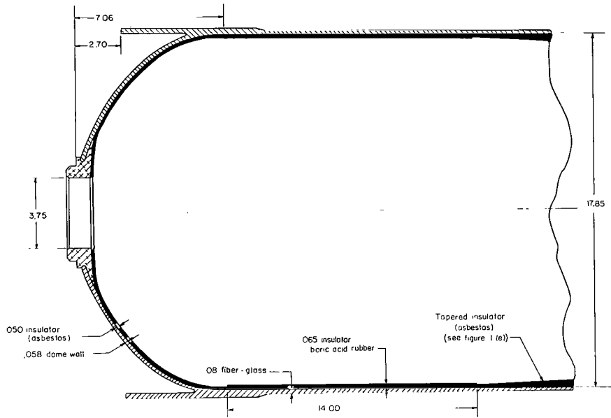
(c) Details of forward dome and cylinder insulator.
