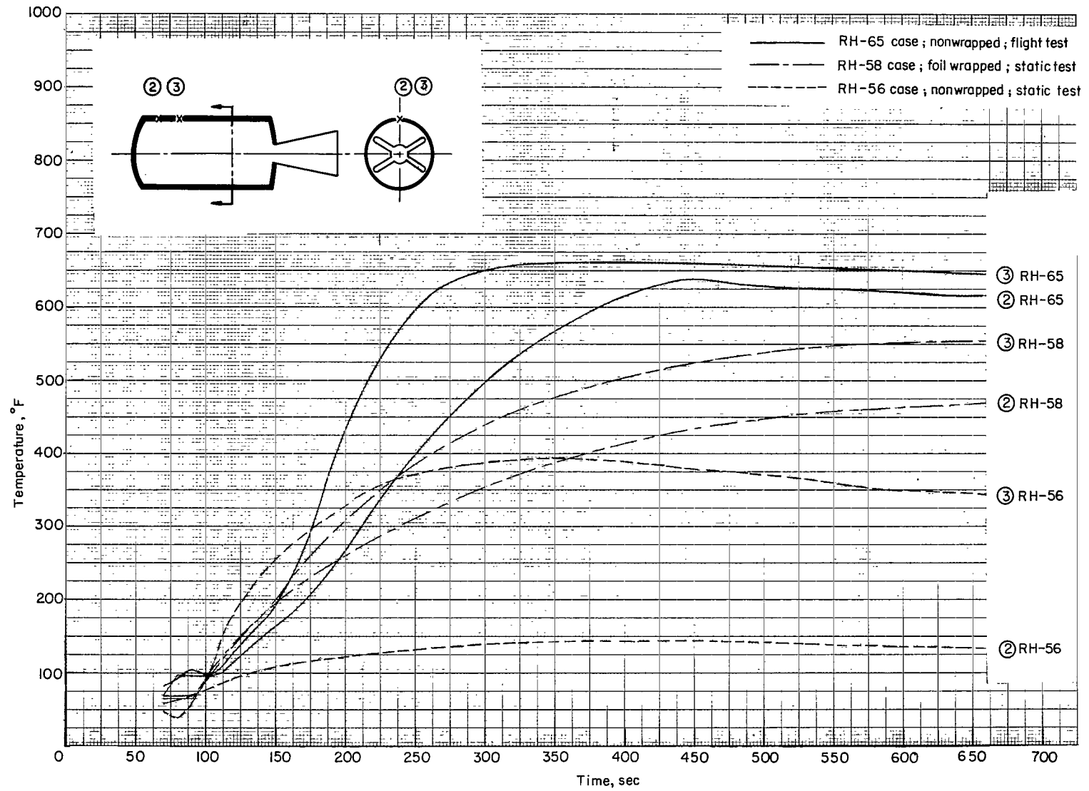
Figure 9.- Forward-cylinder temperatures measured at thermocouples 2 and 3.
