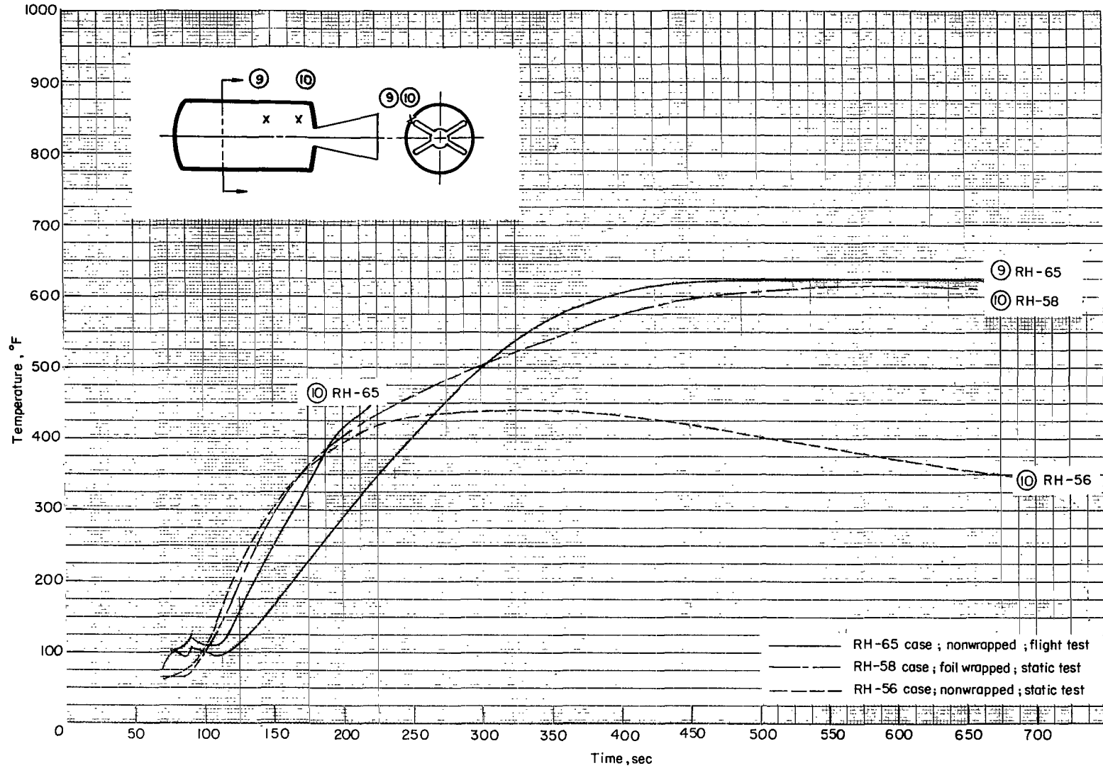
Figure 12.- After-cylinder temperatures measured at thermocouples 9 and 10.
