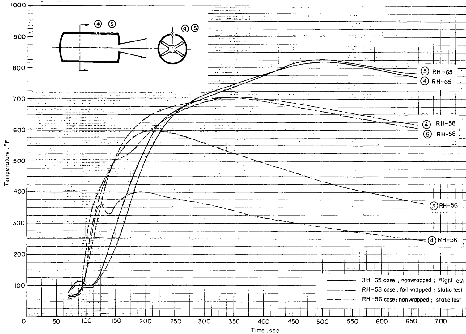
Figure 11.- After-cylinder temperatures measured at thermocouples 4 and 5.
