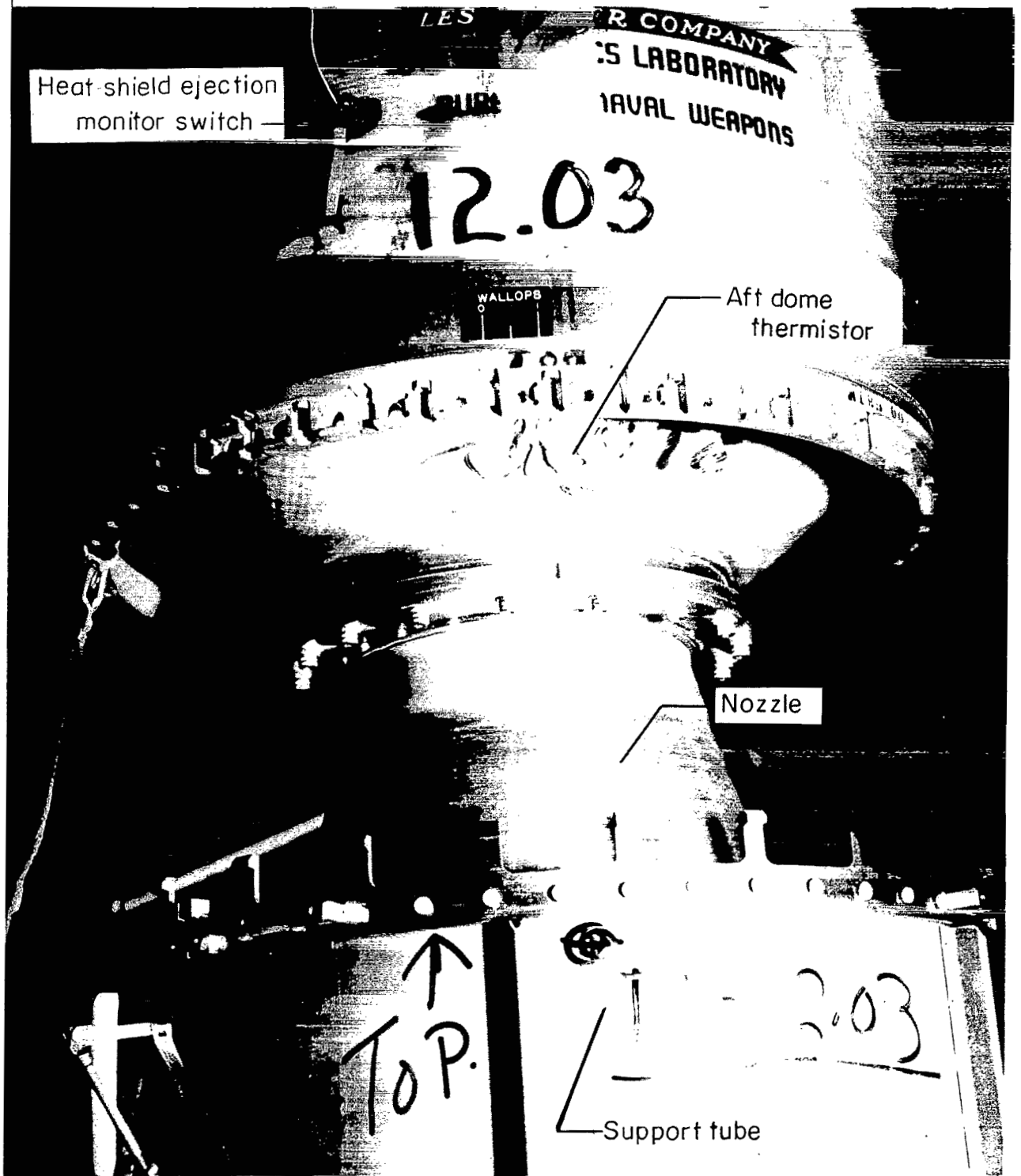
Figure 5.- Altair-IIC1 instrumentation (aft end).
