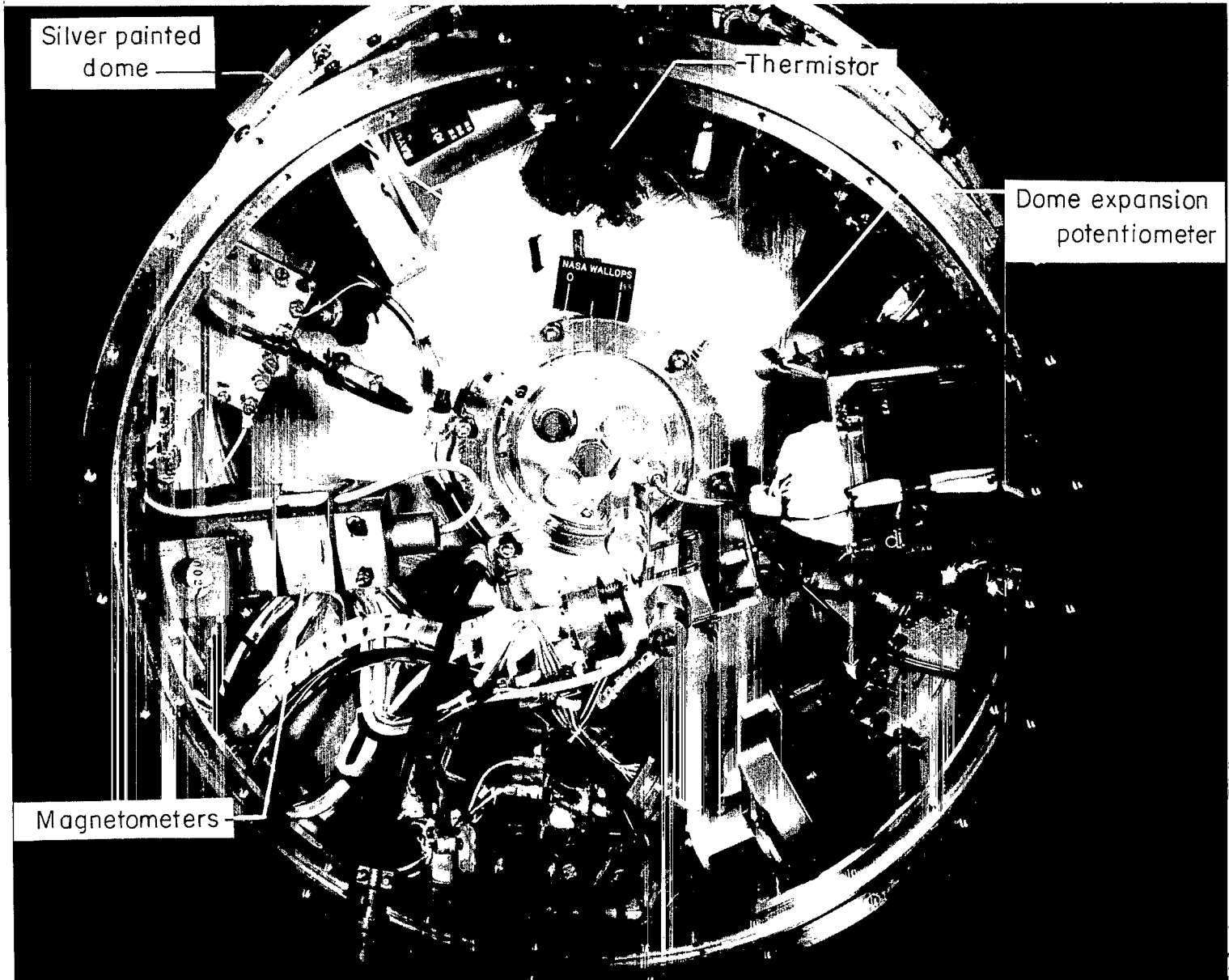
Figure 7.- Altair-II instrument compartment (forward end).
