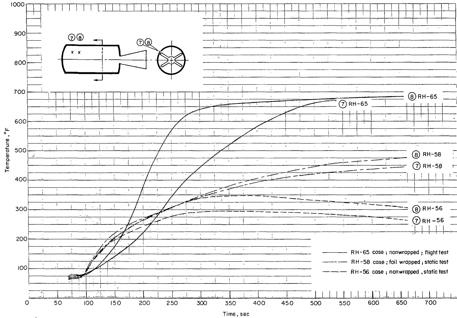
Figure 10.- Forward-cylinder temperatures measured at thermocouples 7 and 8.
