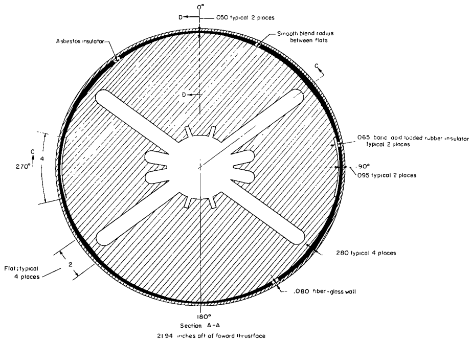
(d) Insulator cross section. (See figure 1(e) for sections C-C and D-D.) Cross section of motor in aft cylinder area.
