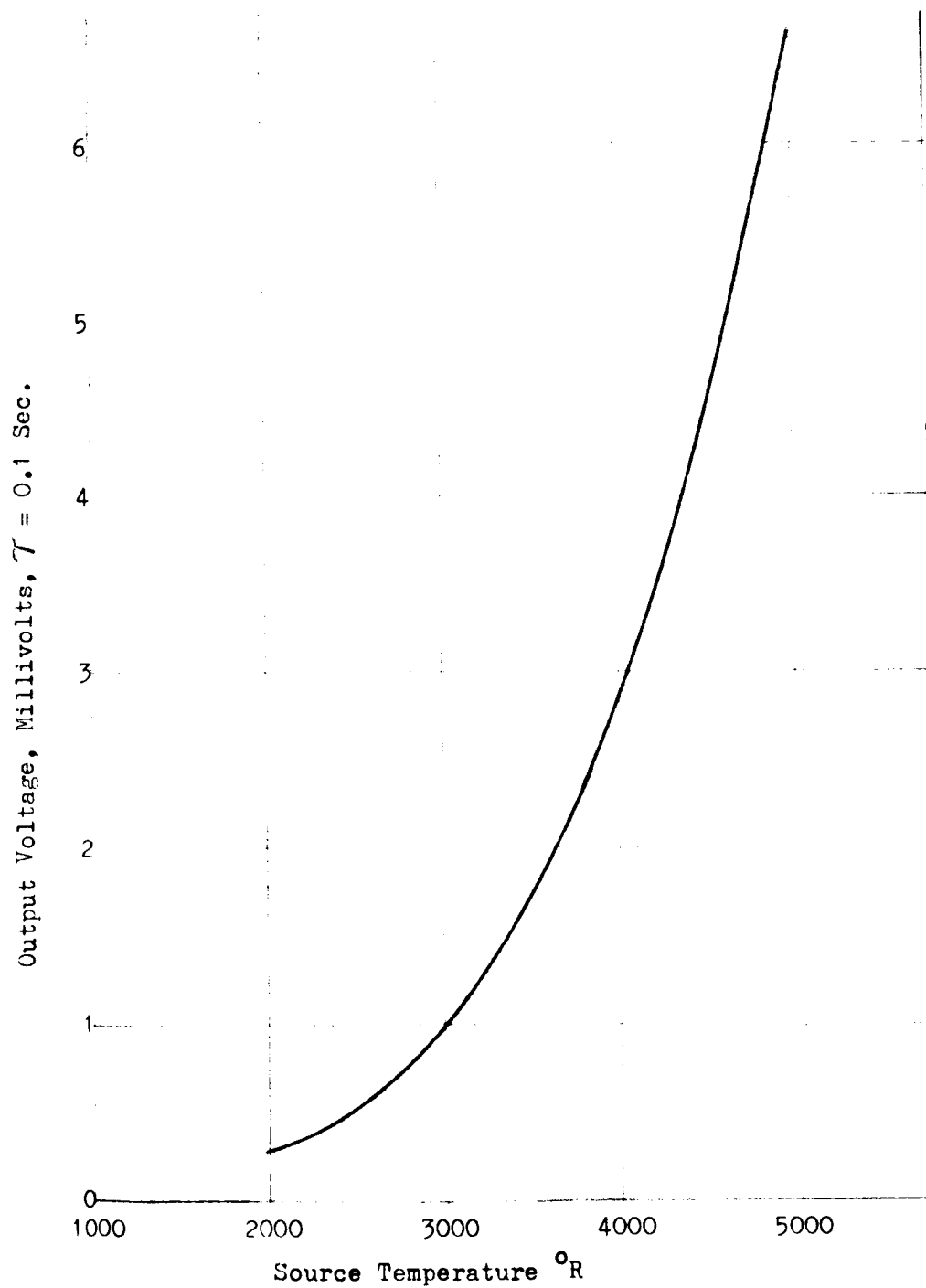
FIGURE 13, TEMPERATURE-MILLIVOLT CURVE FOR CHROMEL VS. ALUMEL FOIL THERMOCOUPLE
