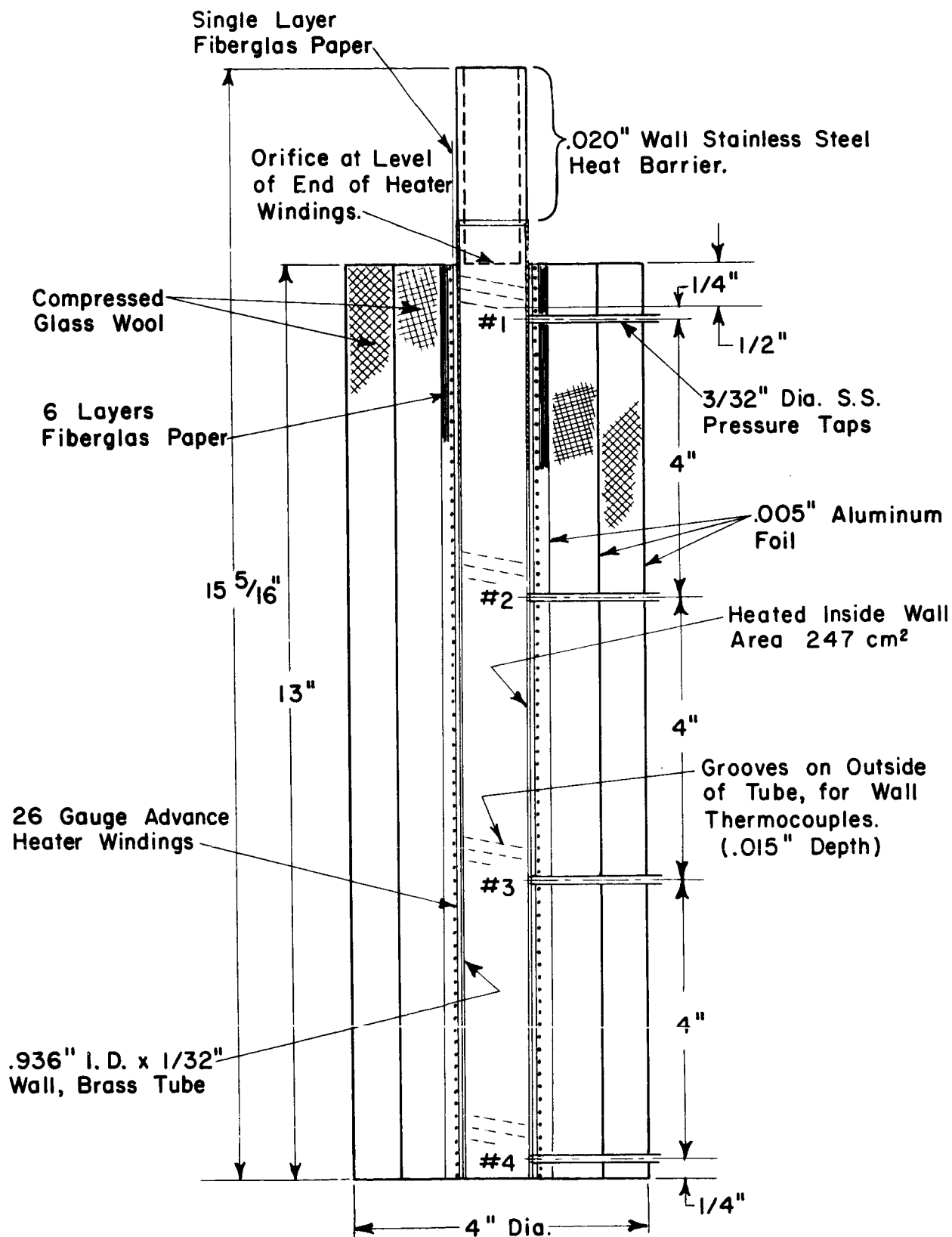
Fig. 3. Heated brass test section.
