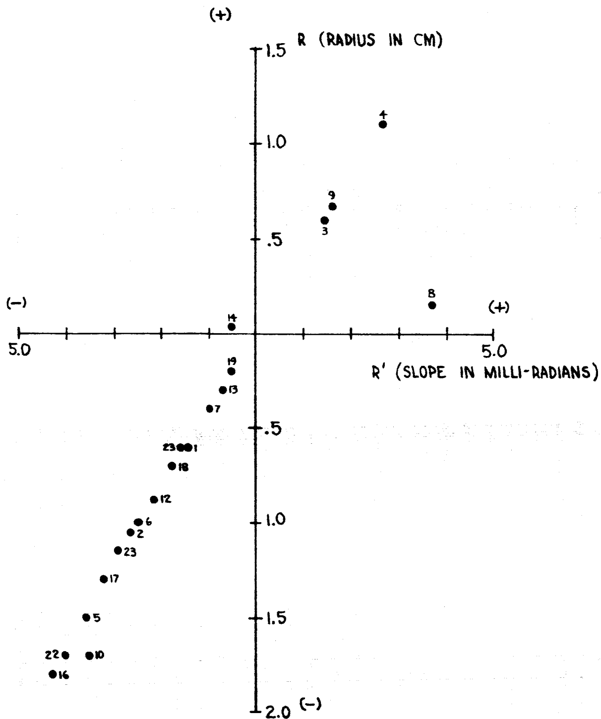
FIG. 9 - INPUT EMITTANCE PROJECTED TO TARGET (2MV)
