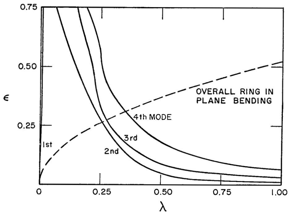
FIG. 12: n=2 MODES, SYMMETRIC, \kappa=0, h/R=0.01
