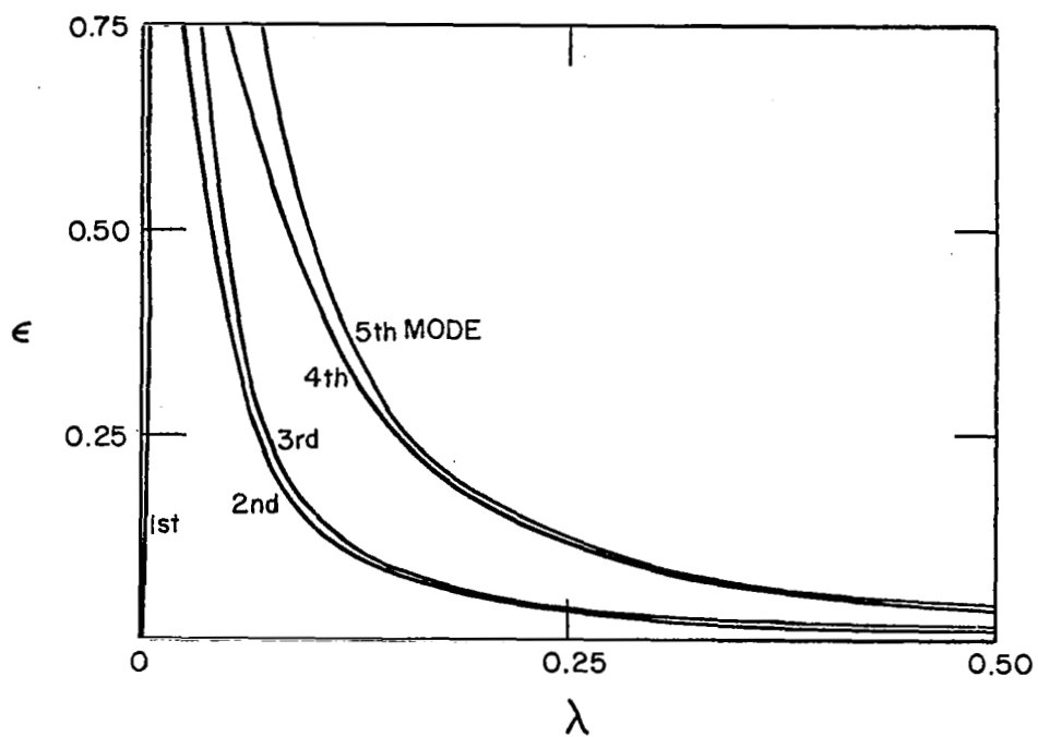
FIG.18: n=2 MODES, SYMMETRIC, \kappa=0 , h/R=0.001
