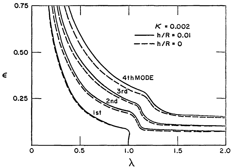
FIG. 2: AXISYMMETRIC MODES, SYMMETRIC, K = 0.002
