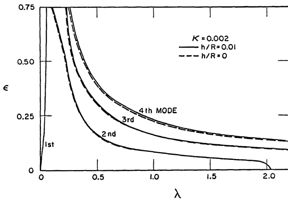
FIG. 7: n = 2 MODES, ANTISYMMETRIC, K = 0.002
