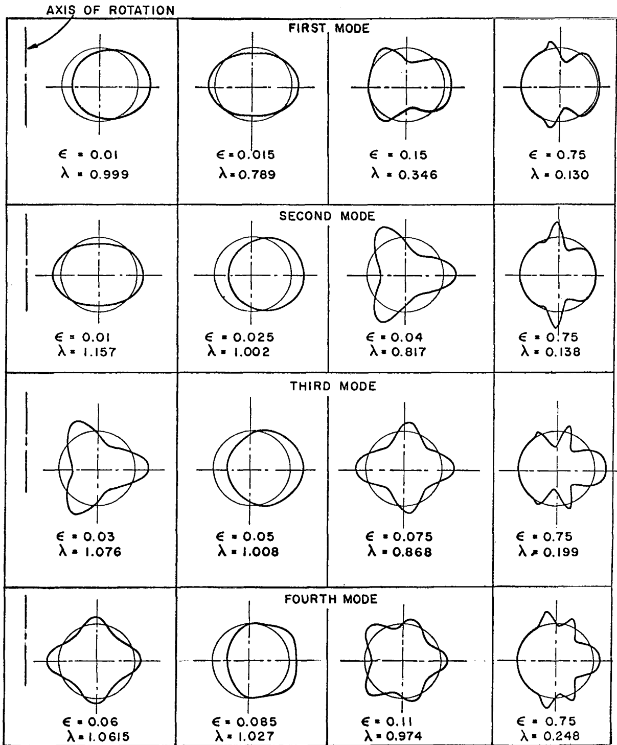
FIG.14: AXISYMMETRIC MODE SHAPES, SYMMETRIC, K=0 , h/R=0.01
