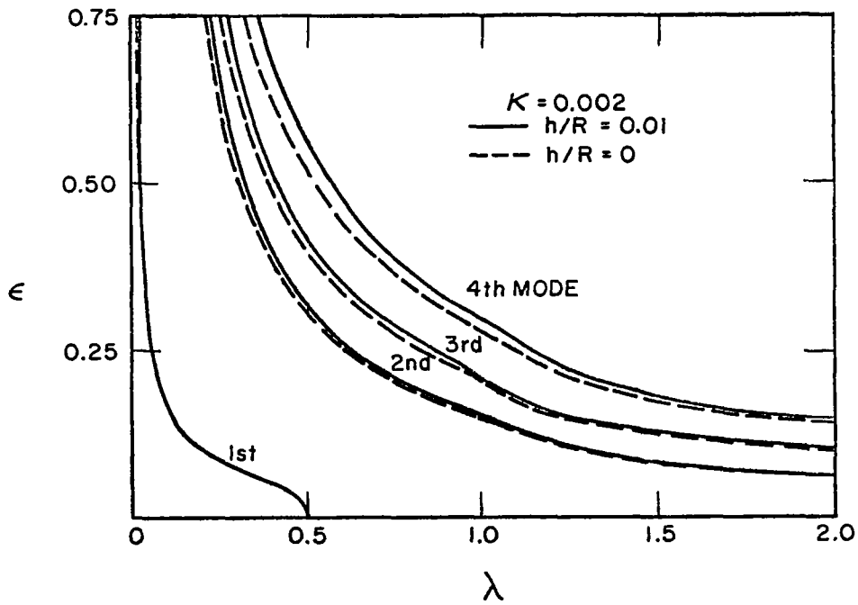
FIG. 3: AXISYMMETRIC MODES, ANTISYMMETRIC, K = 0.002
