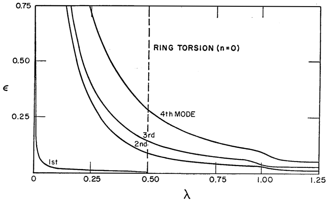
FIG. 11: AXISYMMETRIC MODES, ANTISYMMETRIC, \kappa=0, h/R=0.01
