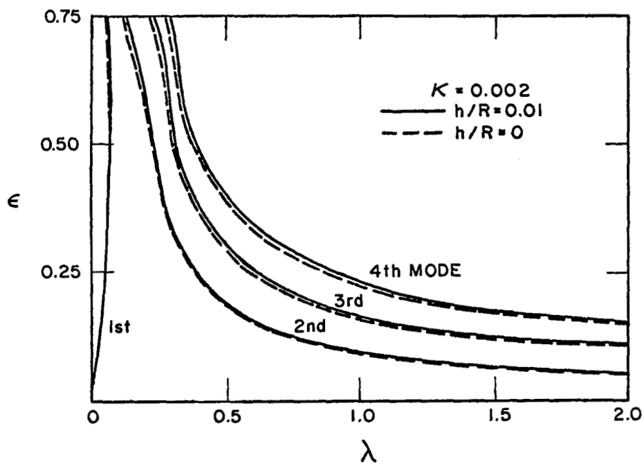
FIG. 6: n = 2 MODES, SYMMETRIC, K = 0.002
