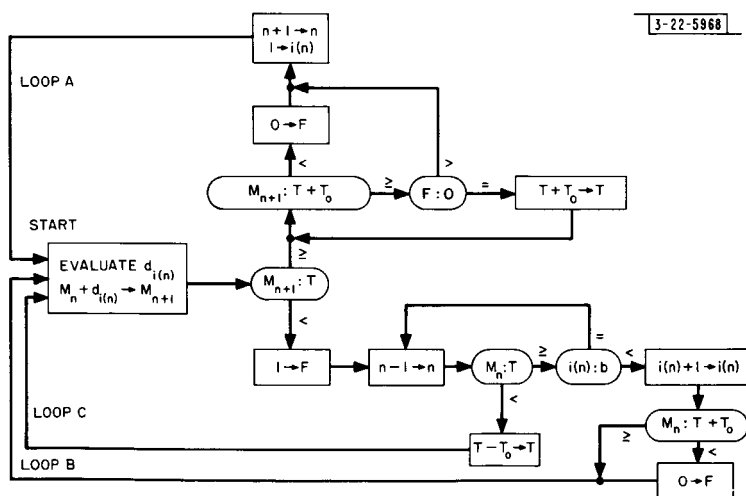
Fig. 5. Flow chart of the sequential decoding procedure (A → B indicates: set B equal to A).
