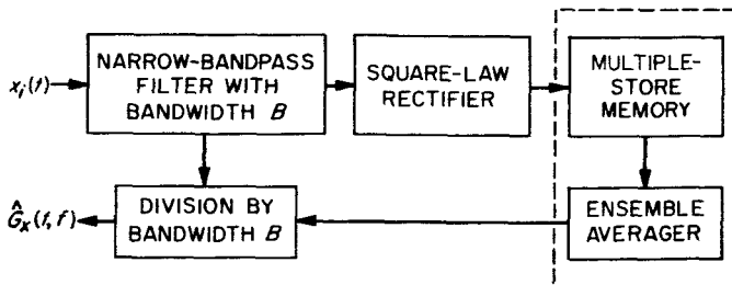
Fig. 6. Time-varying power spectrum measurement
