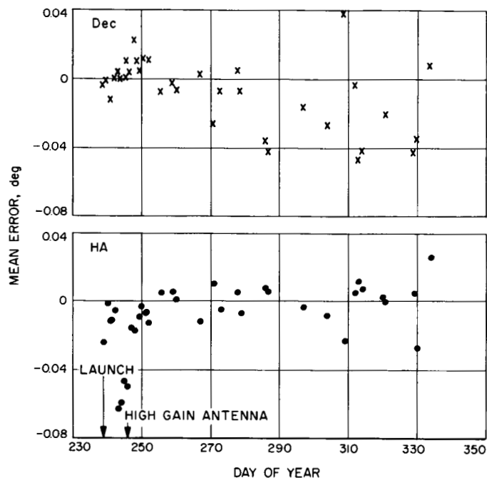
Fig. 28. DSIF-4 HA and Dec mean error vs day of year
