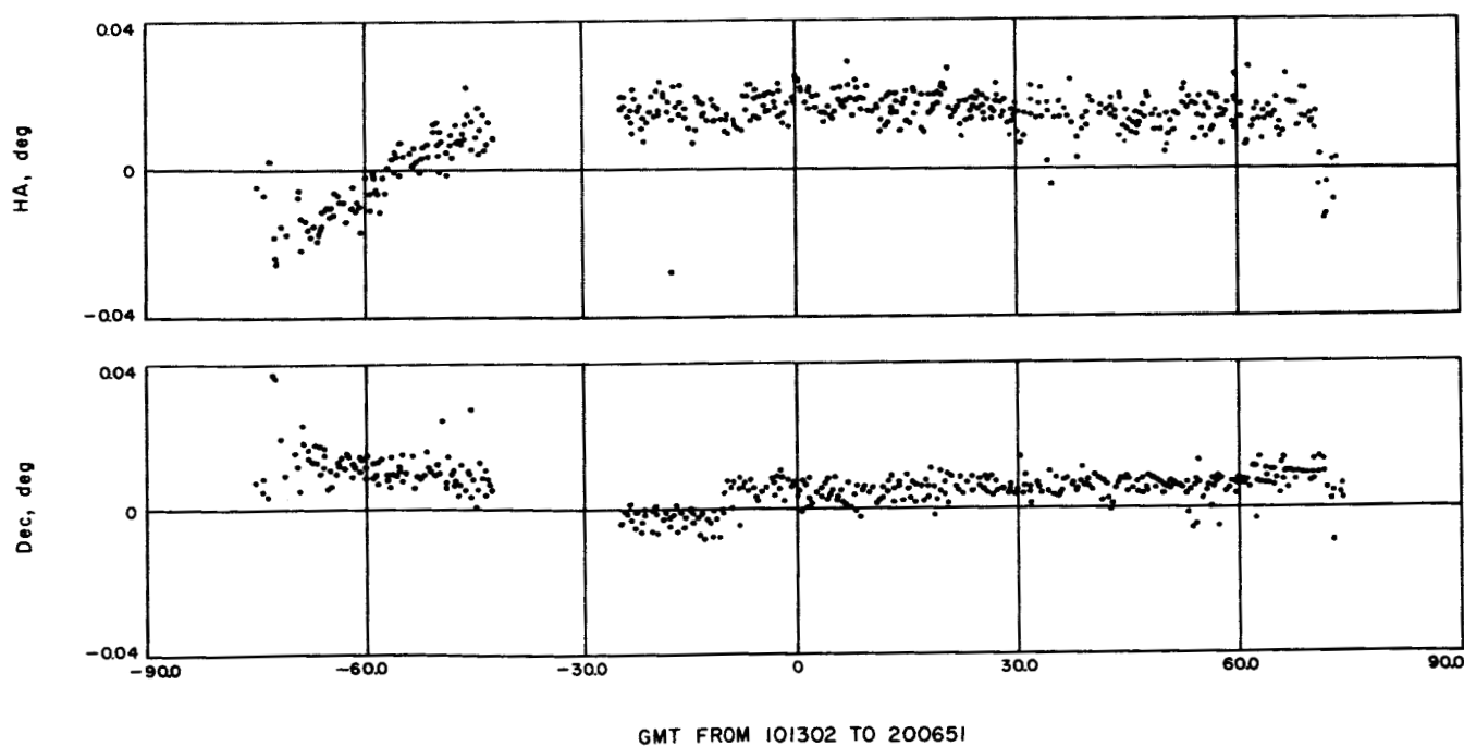
Fig. 34. DSIF-5 HA and Dec residuals vs time (pass No. 2)
