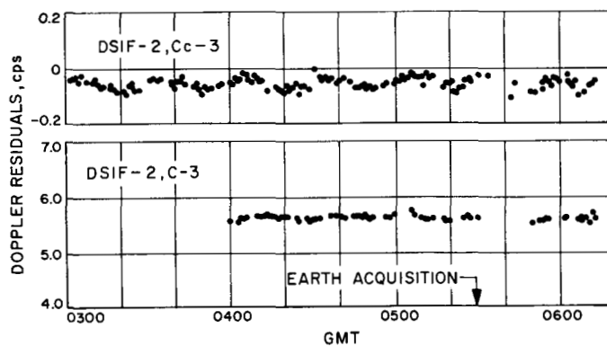
Fig. 9. DSIF-2 and -4 doppler residuals vs time, 3 Sept 1962
