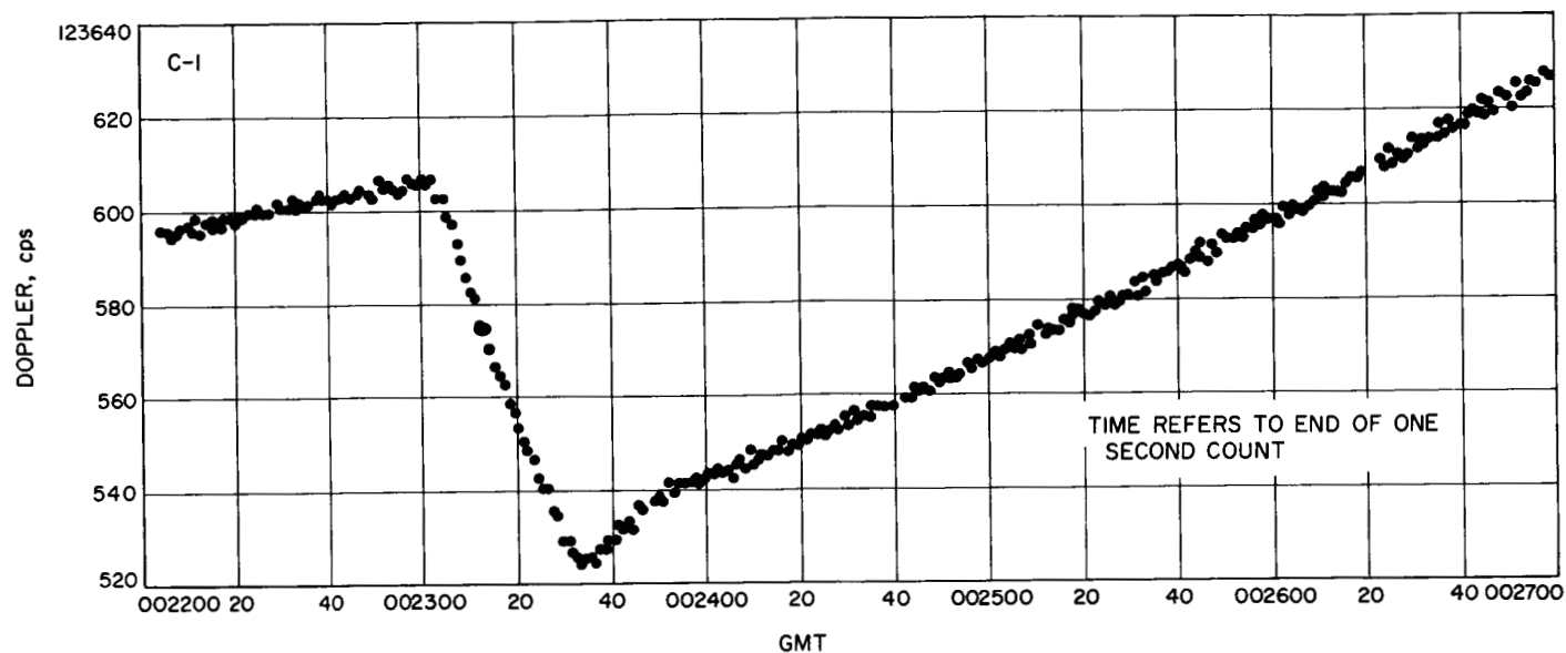
Fig. 12. DSIF-2 C-1 doppler vs time during midcourse, 5 Sept 1962
