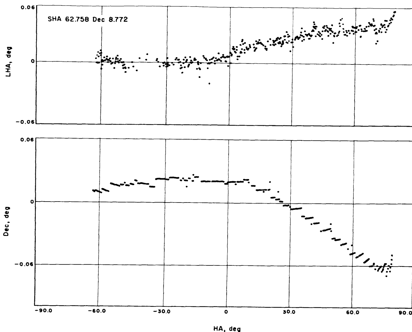
Fig. 3. DSIF-4 star track, 16 Aug 1962
