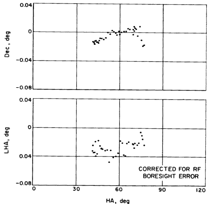
Fig. 20. DSIF-4 LHA and Dec residuals vs HA, 27 Aug 1962 (pass No. 1A)
