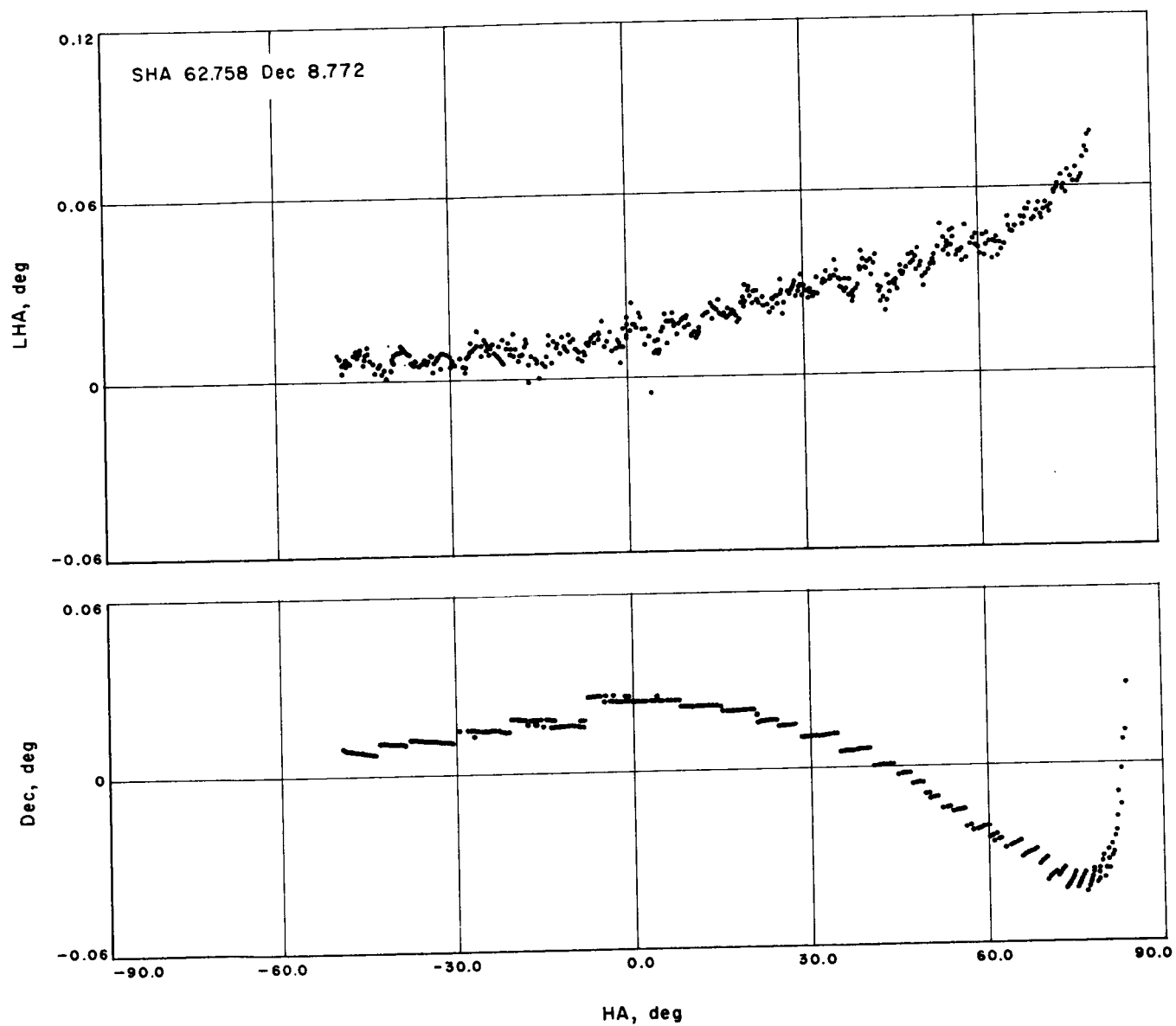
Fig. 4. DSIF-5 star track, 2 Aug 1962
