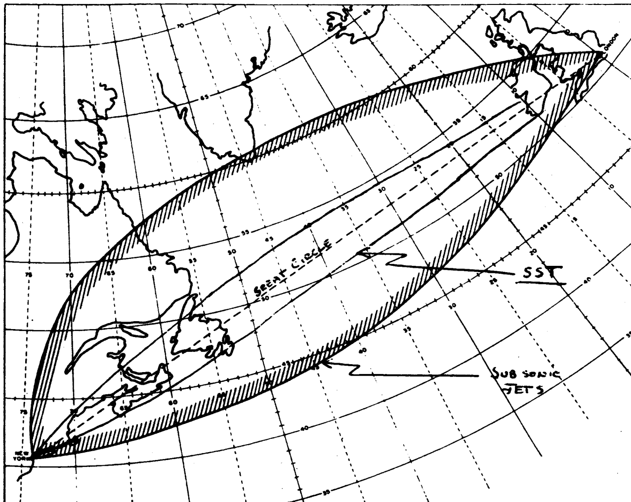
Figure 1 - Envelope of Minimum Time Tracks - 300 Millibar Level
