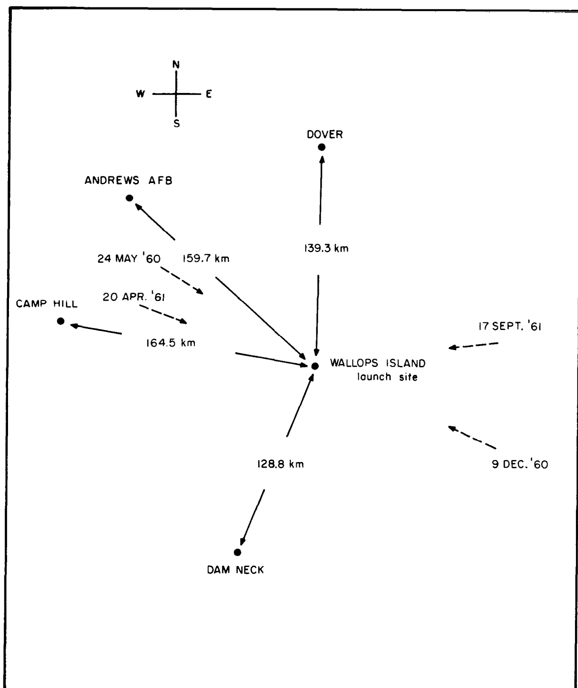
Figure 3. Relative position of camera sites to the Wallops Island Launch site. Dashed arrows represent the solar azimuth angle of the sun at 7^{\circ} solar depression during cloud photography of four specific sodium trails.
