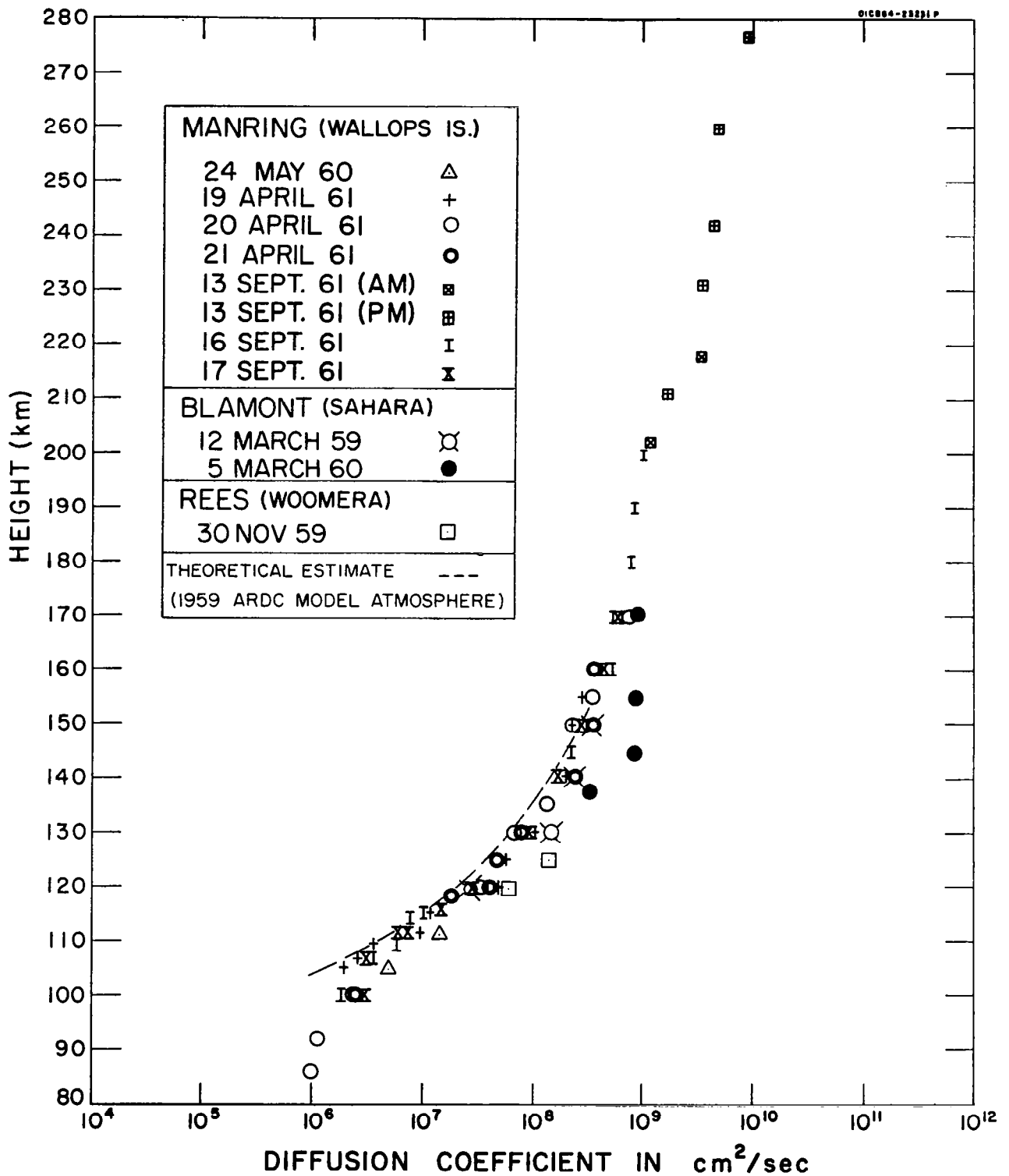
Figure 6. The height variation in the experimental values of molecular diffusion coefficient.
