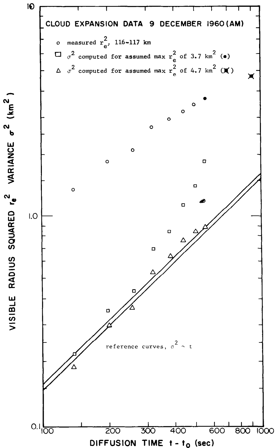
Figure 11. Variation in time of the measured visible radius squared and variance computed from two assumed values of the maximum cloud radius squared, r_e^2 = 3.7 and 4.7 km. The measured r_e^2 are at 116 to 117 km for the morning twilight cloud of 9 December 1960.
