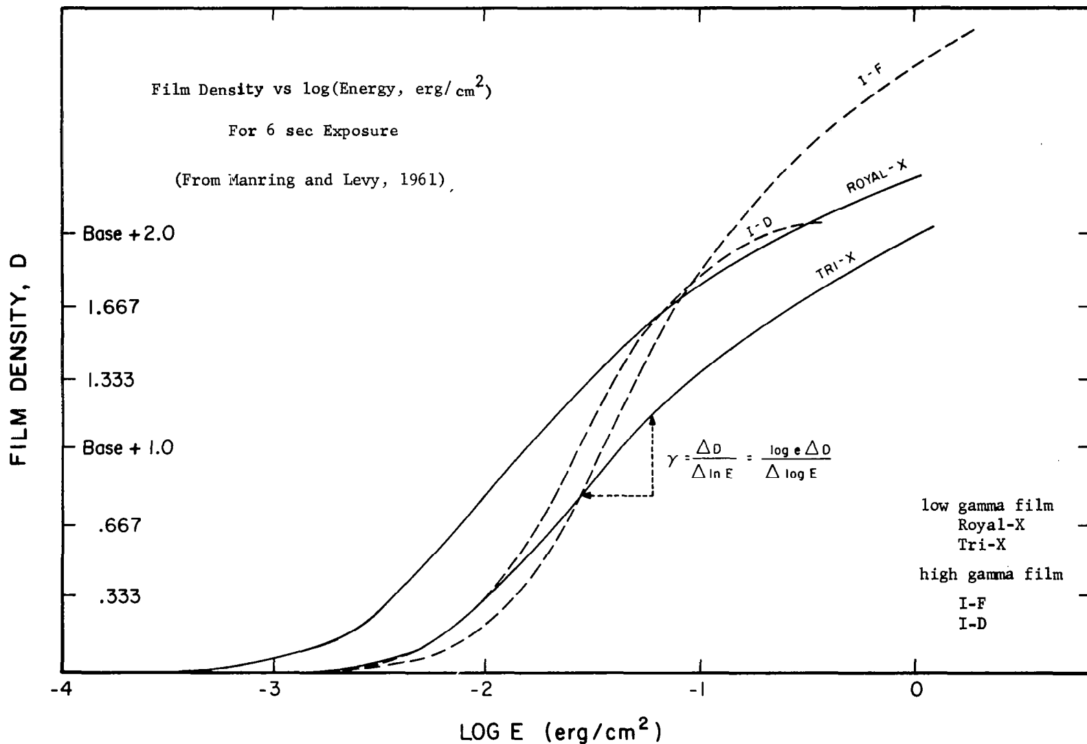
Figure 1. Illustrations of the empirical relationship between the energy received by a film and its degree of darkening, the film density, D.
