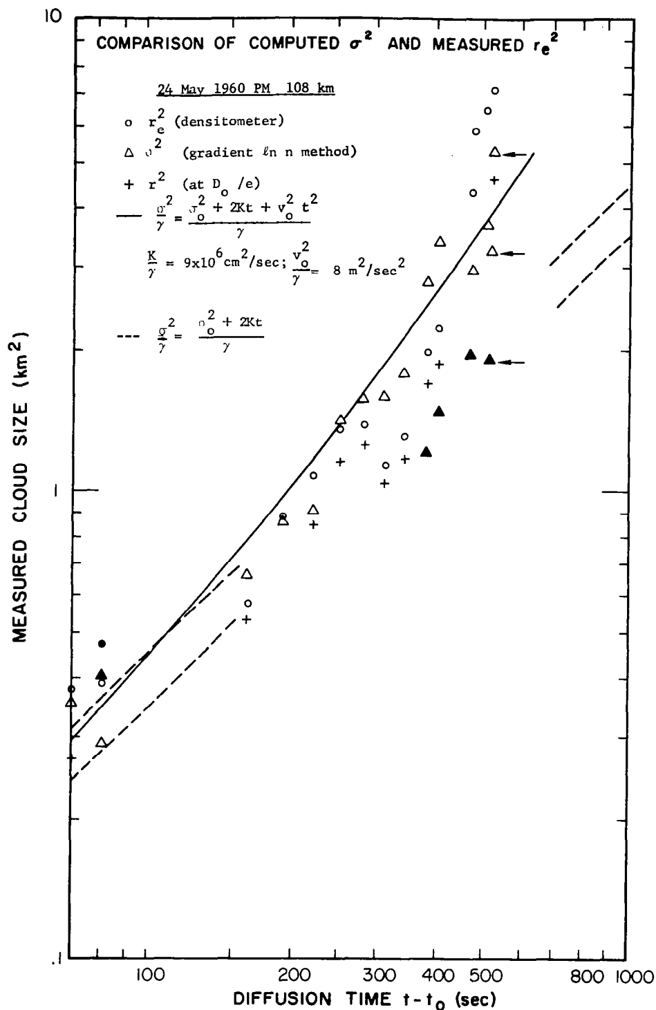
Figure 7. A comparison of the measured visible radius squared with computed values of the cloud variance, \sigma^2 , for the evening twilight of 24 May 1960. The equivalent height of the cloud is 108 \pm 1 km.
