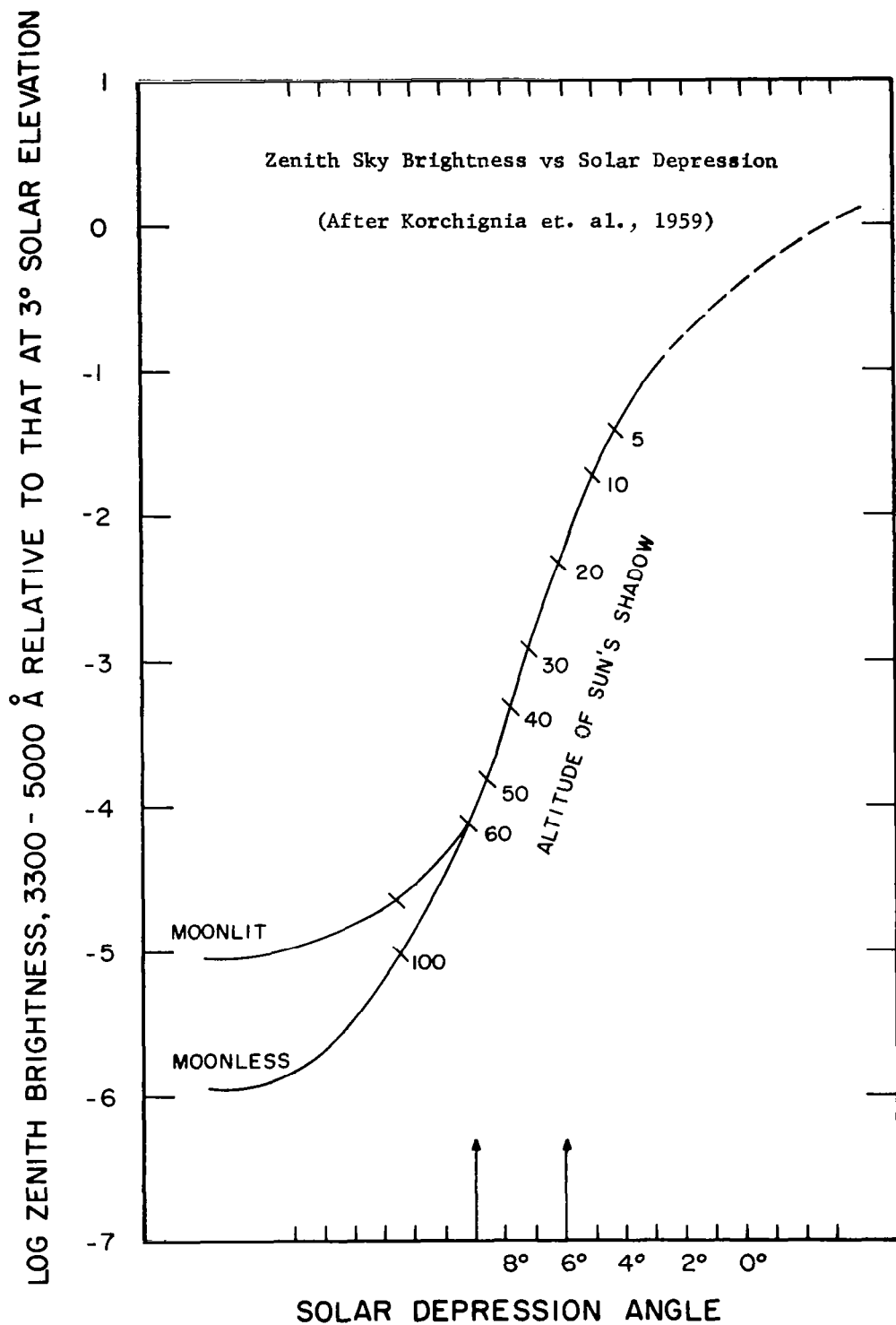
Figure 5. Typical variation of Zenith Sky Brightness at 4000Å with changes in solar depression angle.
