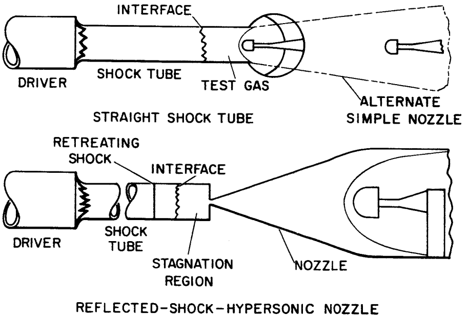
Figure 4. Popular modifications of simple shock tube.
