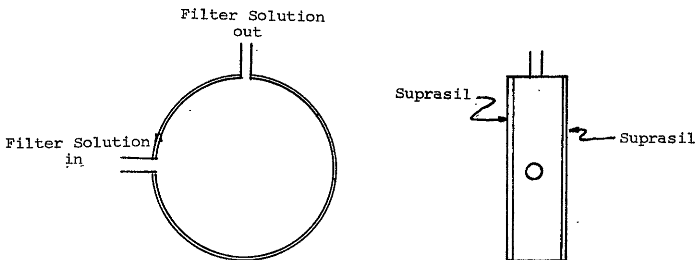
Figure 16 FILTER SOLUTION TEST CELL
