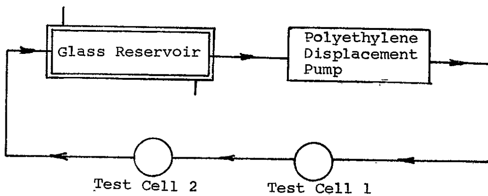
Figure 17 SCHEMATIC OF LIQUID FILTER ASSEMBLY
