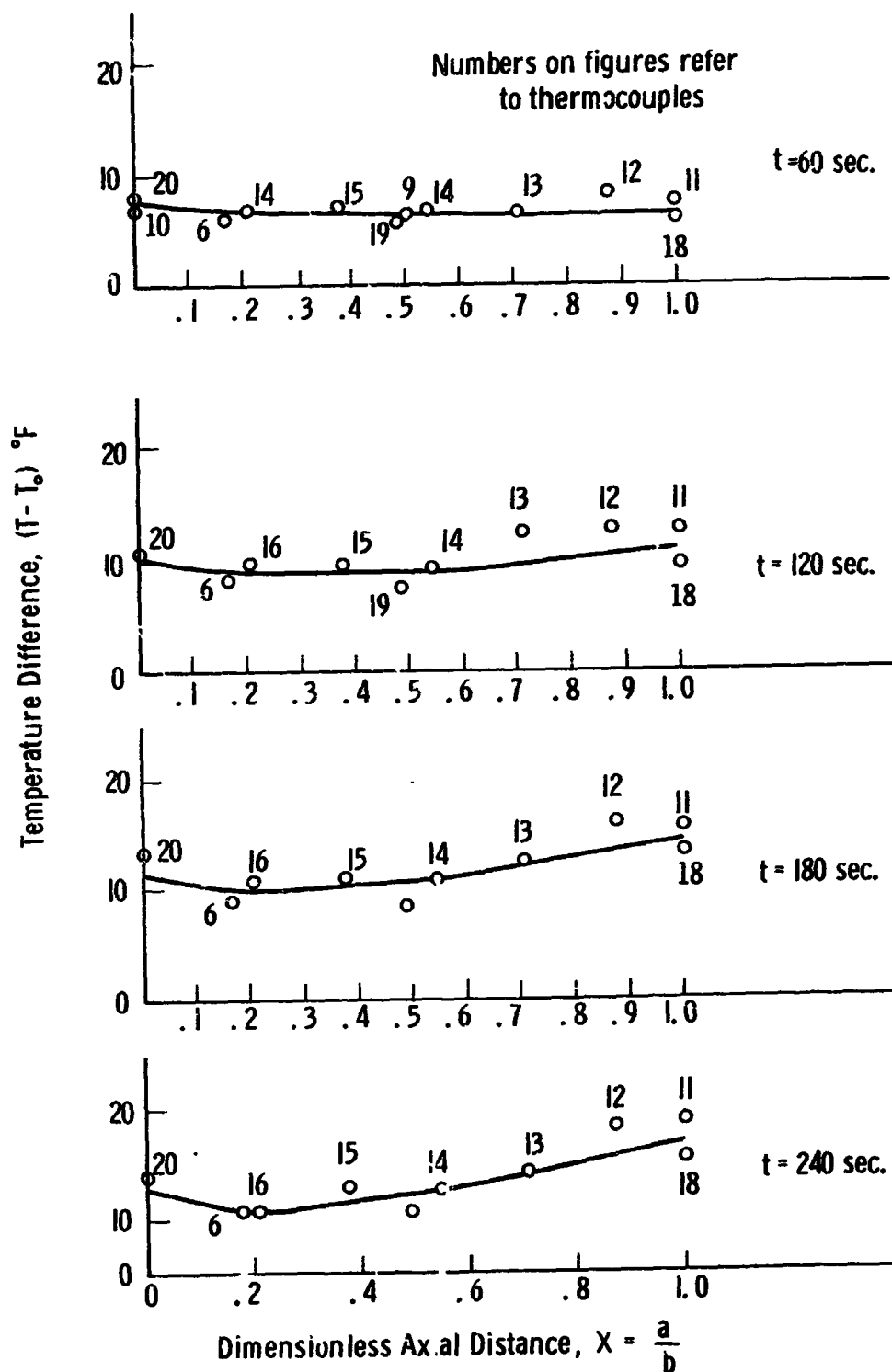
Fig. 14. Wall temperature distribution, run 2, cylindrical container. (q/A)_w = .500 \text{ Btu/hr ft}^2 .
