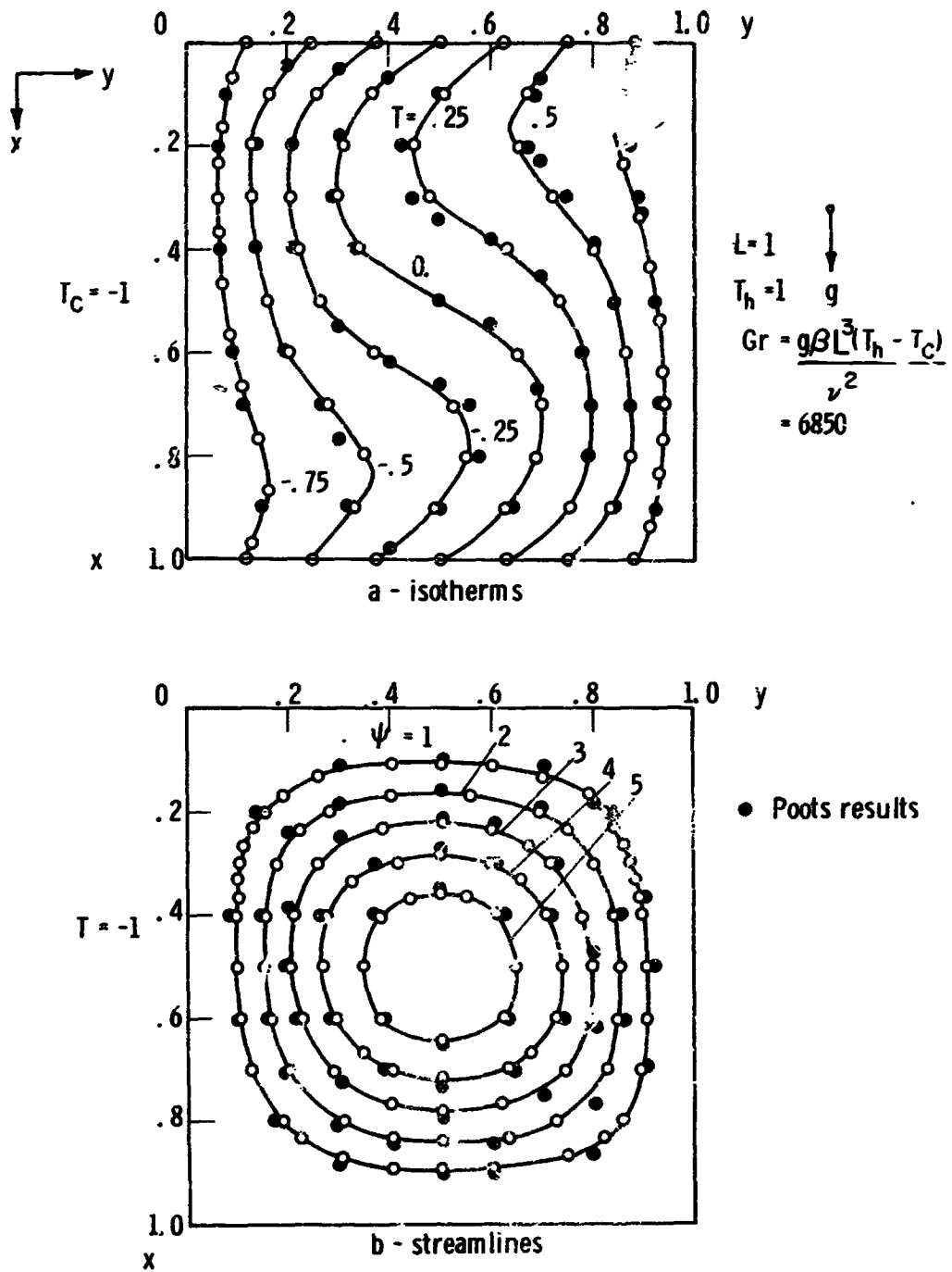
Fig. 17. Results for the rectangular cavity problem using 31 \times 31 grid.
