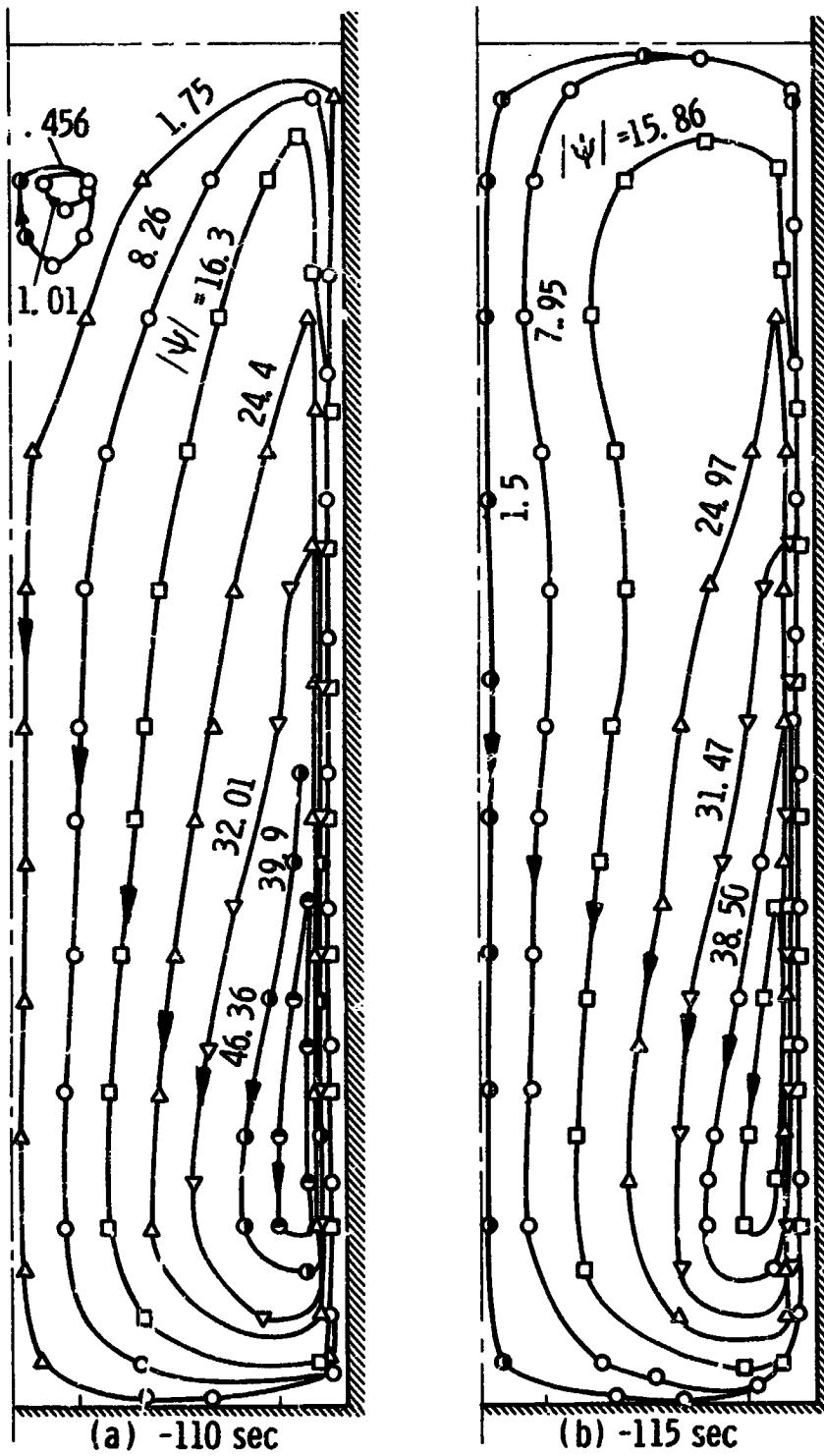
Fig. 32. Isotherms in the rectangular container, run 1. Time is 110 sec.
