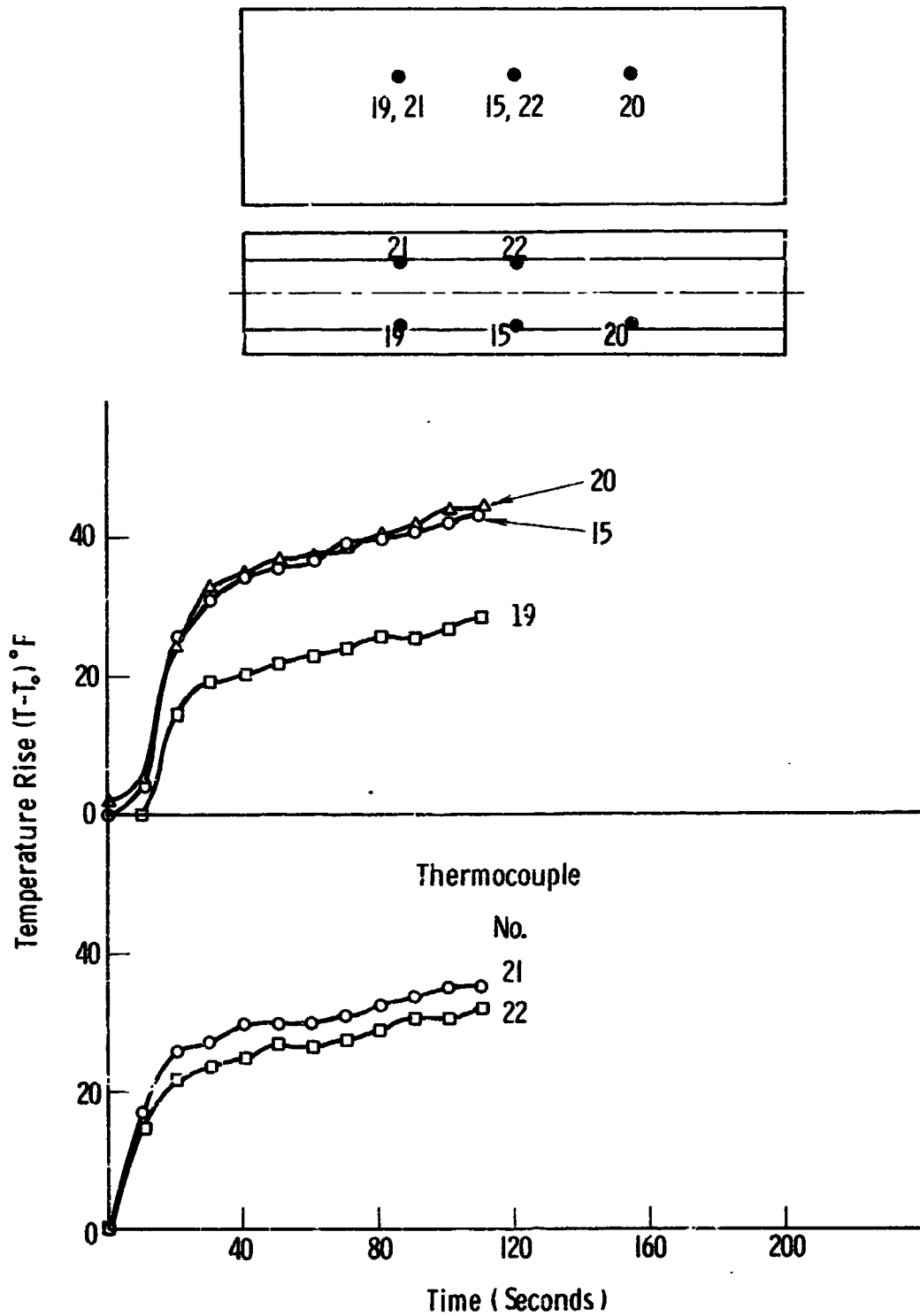
Fig. 13. Typical wall temperature response, rectangular container.
