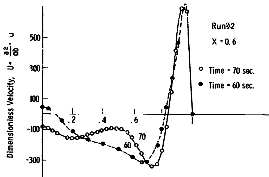
Fig. 54. Calculated velocity distribution at high values of time in the cylindrical container, run 2. (q/A)_w = 500 \text{ Btu/hr ft}^2 .
