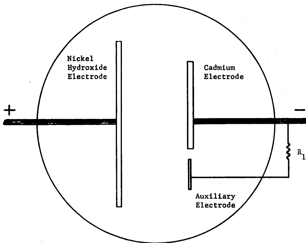
Figure 1 Schematic of Auxiliary Electrode Cell
