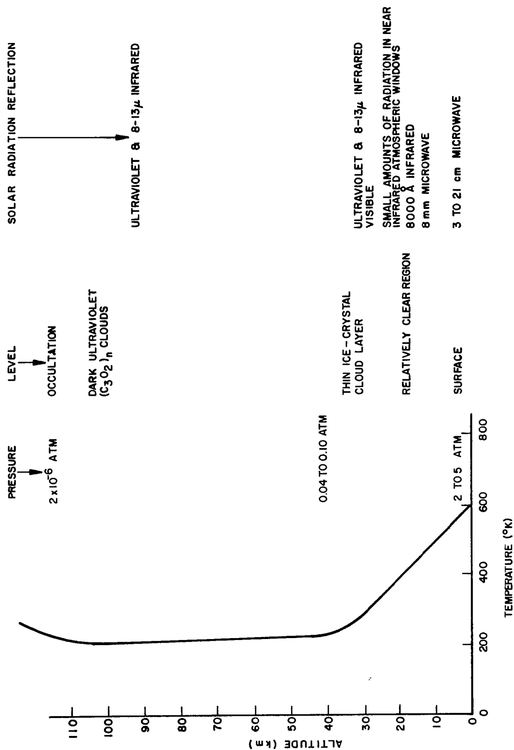
GREENHOUSE MODEL OF THE VENUSIAN ATMOSPHERE
