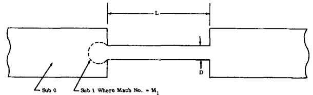
Fig. A14 Pressure Chamber Configuration
