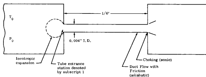
Fig. A17 Pressure Chamber Configuration Showing Operating Conditions
