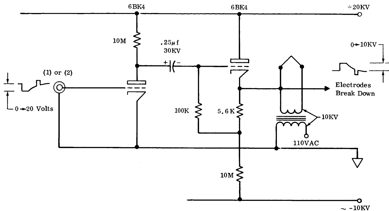
Fig. 14 Repeller H. V. Amplifier
