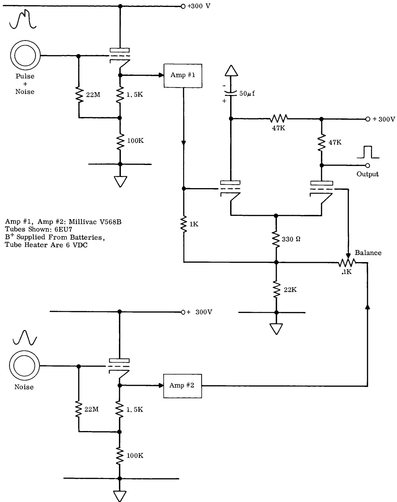
Fig. 2 Difference Amplifier
