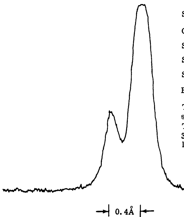
Figure 18. Signal of Figure 17 after integration with Enchancetron.
