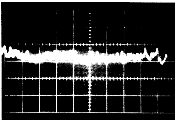
Figure 6. Single sweep oscilloscope trace of a 1P28 photomultiplier output signal buried in noise. (Argon lines 4333.56 and 4335.35Å).
