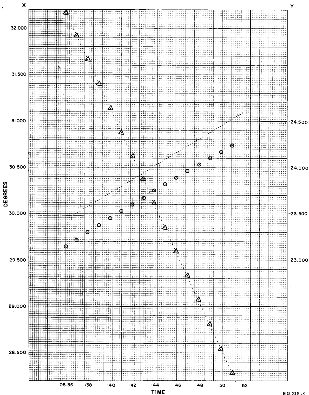
Figure 2-37. Program Star Track, Betelgeuse
