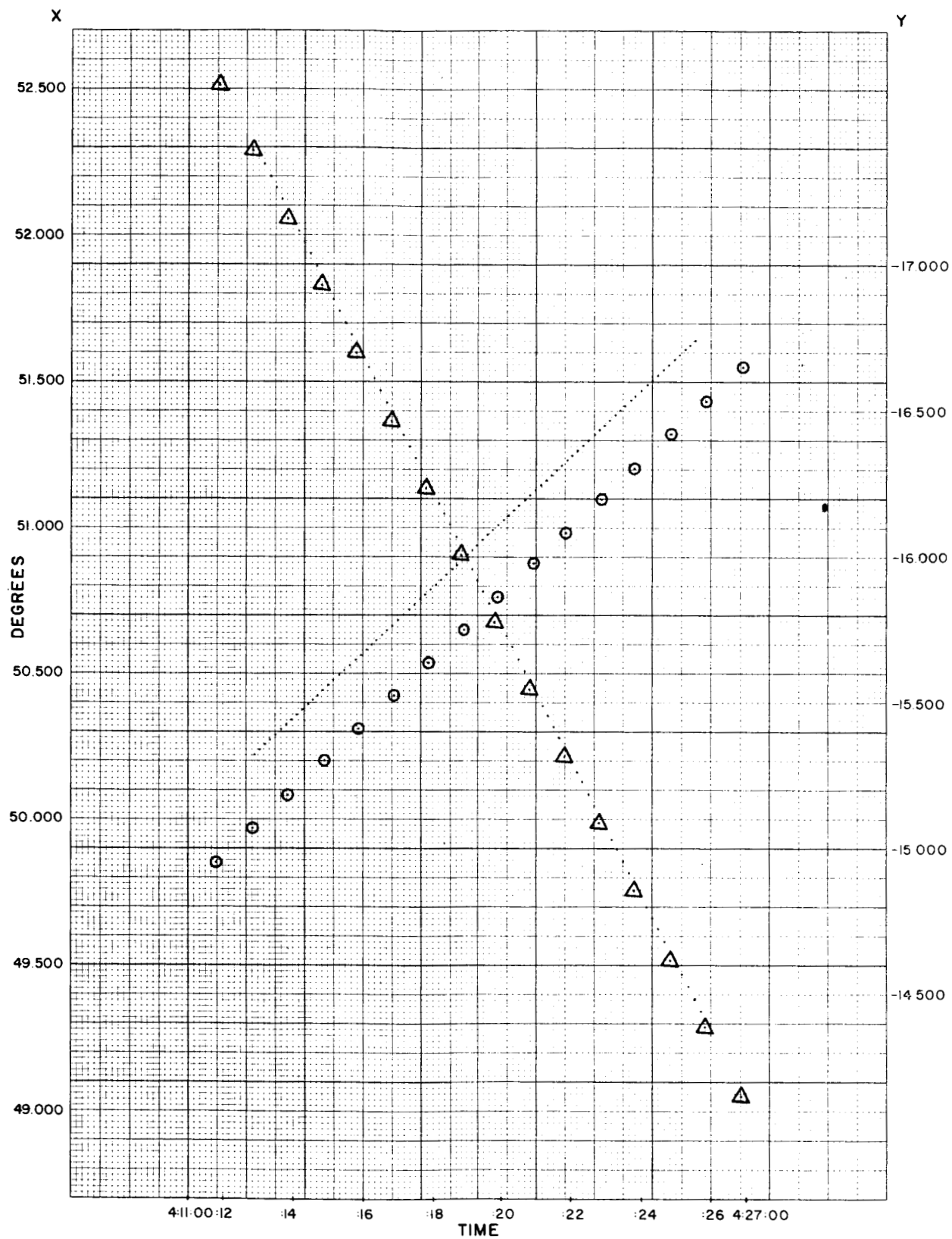
Figure 2-40. Program Star Track, Betelgeuse
