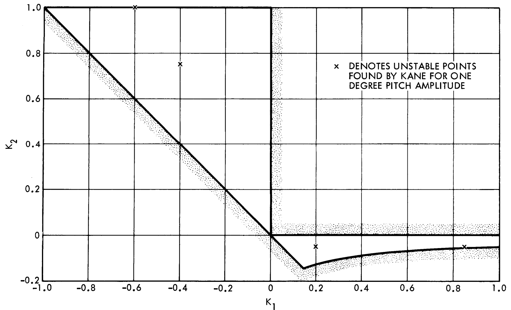
Figure 3.5. Locations of Points for Which Pure Pitch Motion is Unstable
