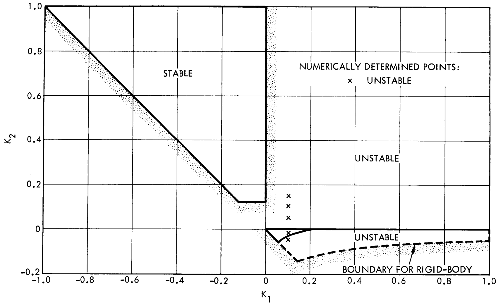
Figure 3.14. Regions of Infinitesimal Stability for Damped System, With \omega_n = 5
