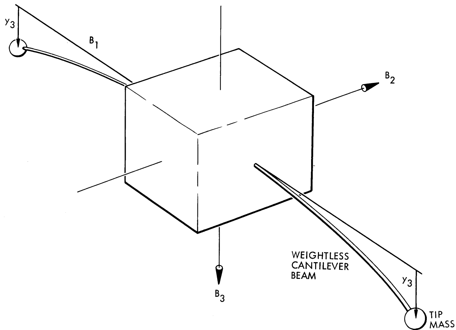
Figure 4.2. Satellite With Appendages
