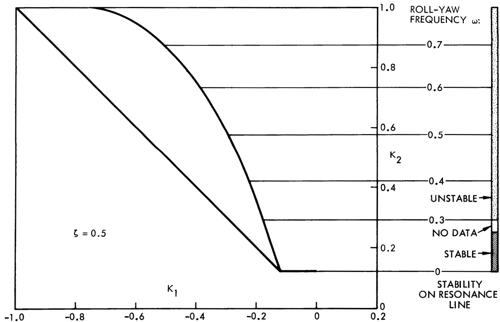
Figure 3.22. Effect of Damping on Stability of Planar Pitch Motion, for \omega_n = 5 , Half Amplitude One Degree
