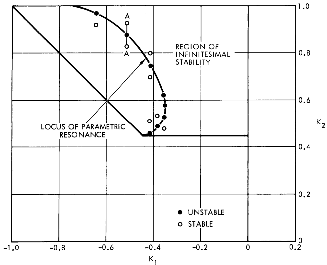
Figure 3.17. Locus of Parametric Resonance for \omega_n = 1 , Showing Numerical Stability Results for One Degree Pitch Amplitude
