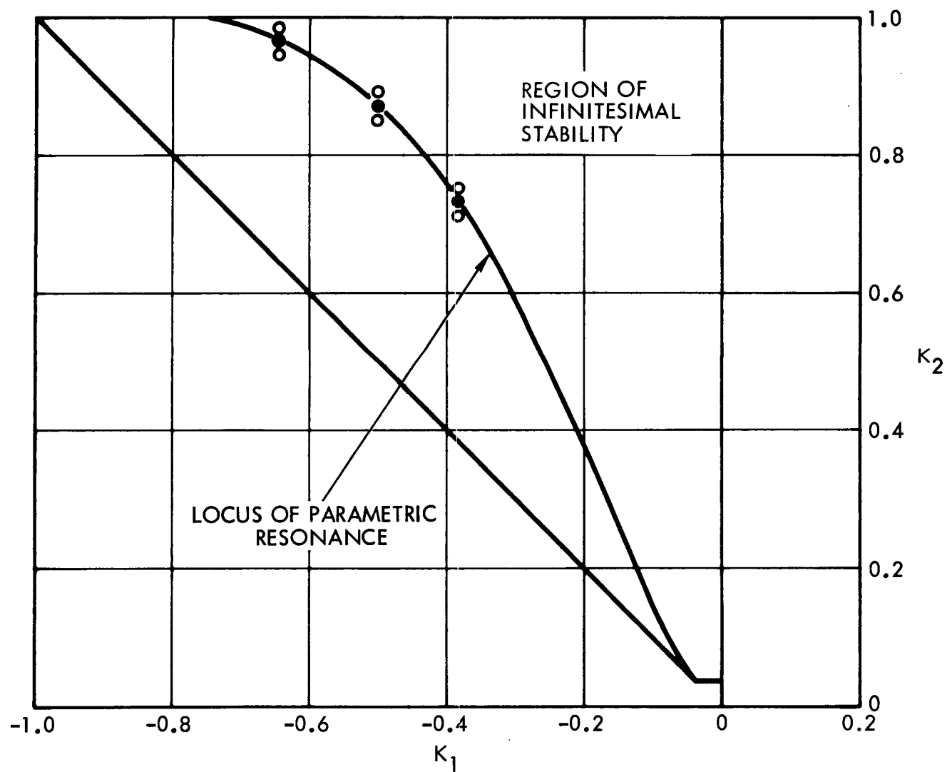
Figure 3.19. Locus of Parametric Resonance for \omega_n = 10 , Showing Numerical Stability Results for One Degree Pitch Amplitude
