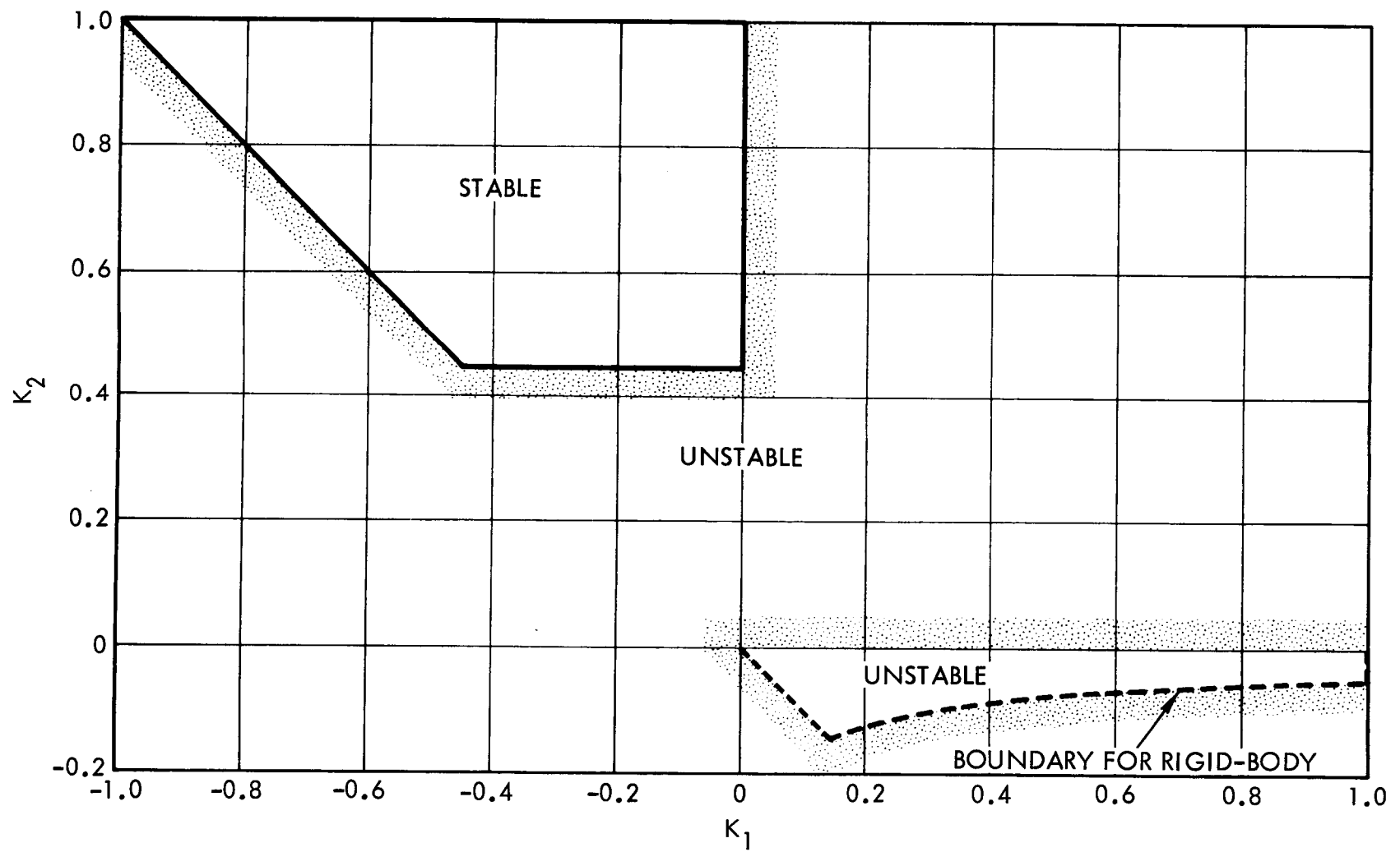
Figure 3.15. Region of Infinitesimal Stability for Damped System, With \omega_n = 1
