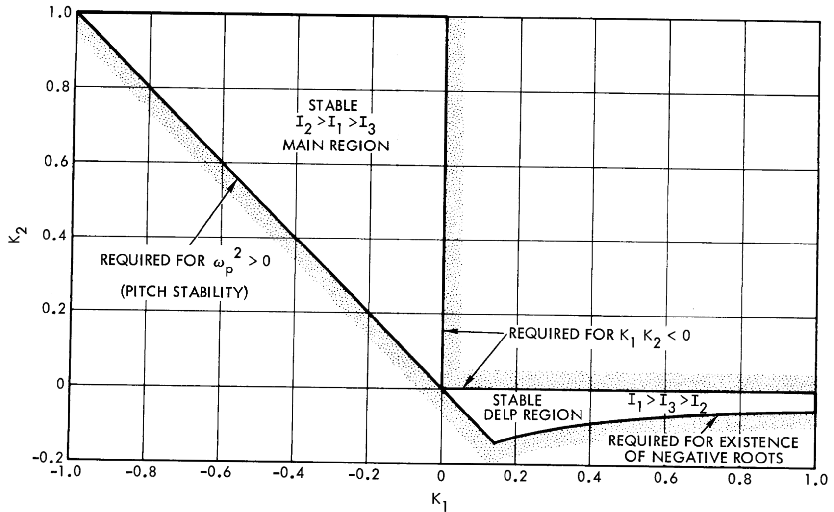
Figure 3.3. Regions of Satellite Stability in K_1 - K_2 Plane, Showing Reasons for Existence of Boundaries.
