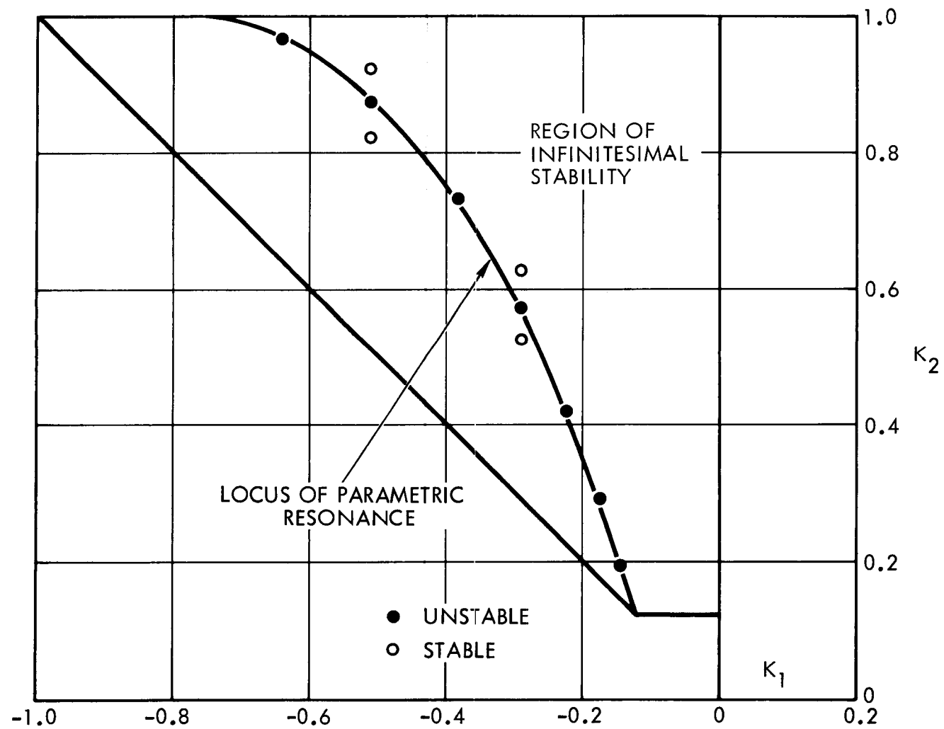
Figure 3.18. Locus of Parametric Resonance for \omega_n = 5 , Showing Numerical Stability Results for One Degree Pitch Amplitude
