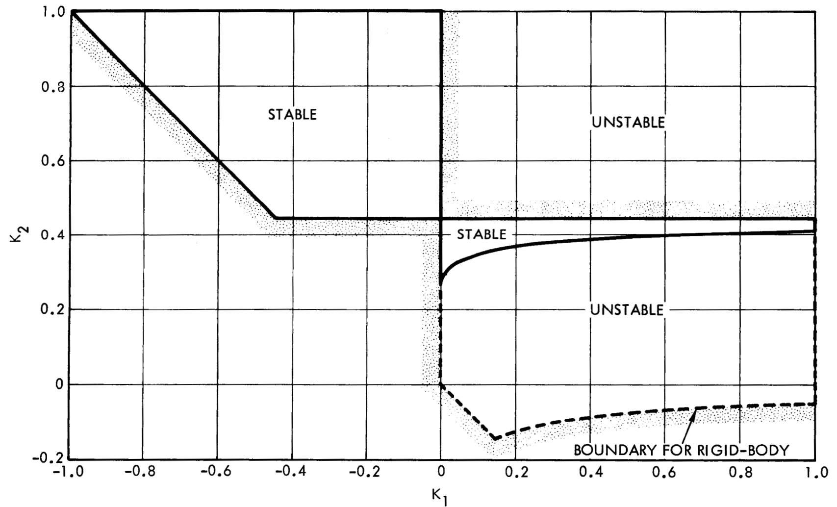
Figure 3.13. Regions of Infinitesimal Stability for \omega_n = 1
