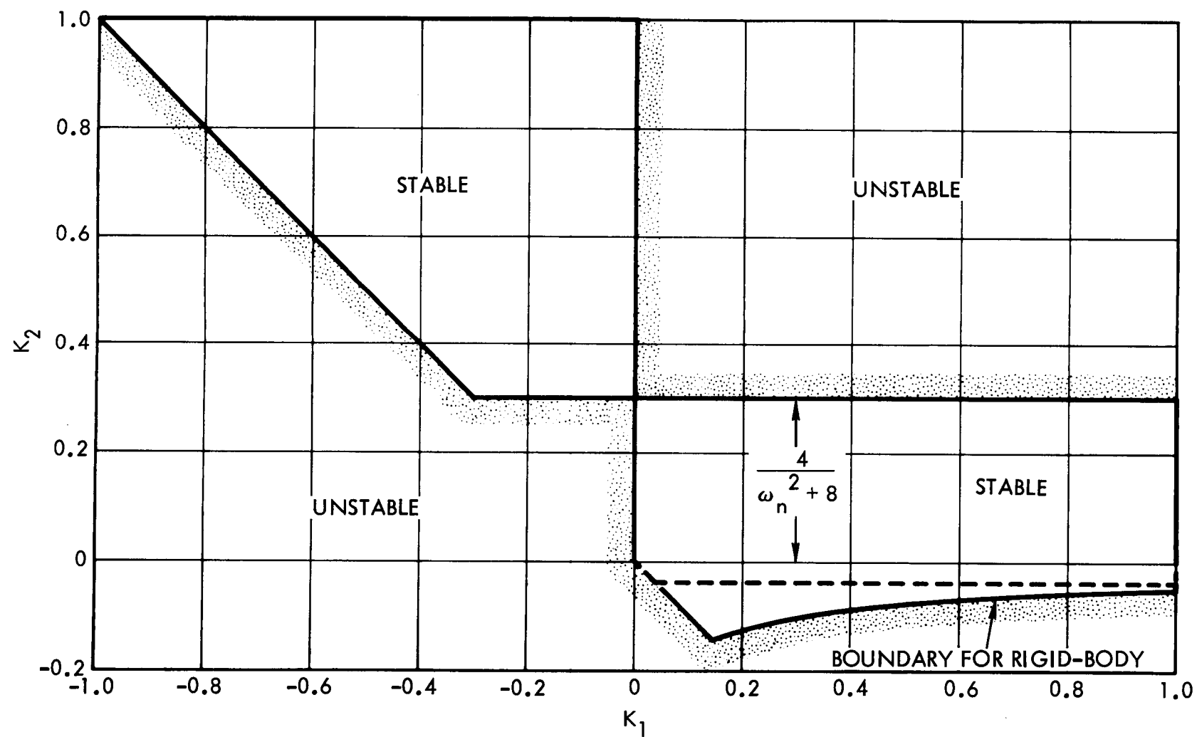
Figure 3.9. Partial Stability Diagram for Flexible Body
