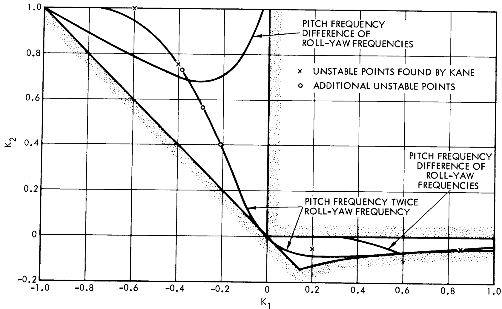
Figure 3.6. Loci of Coincidence Between Pitch and Roll-Yaw Frequencies, Showing Relationship to Numerical Results
