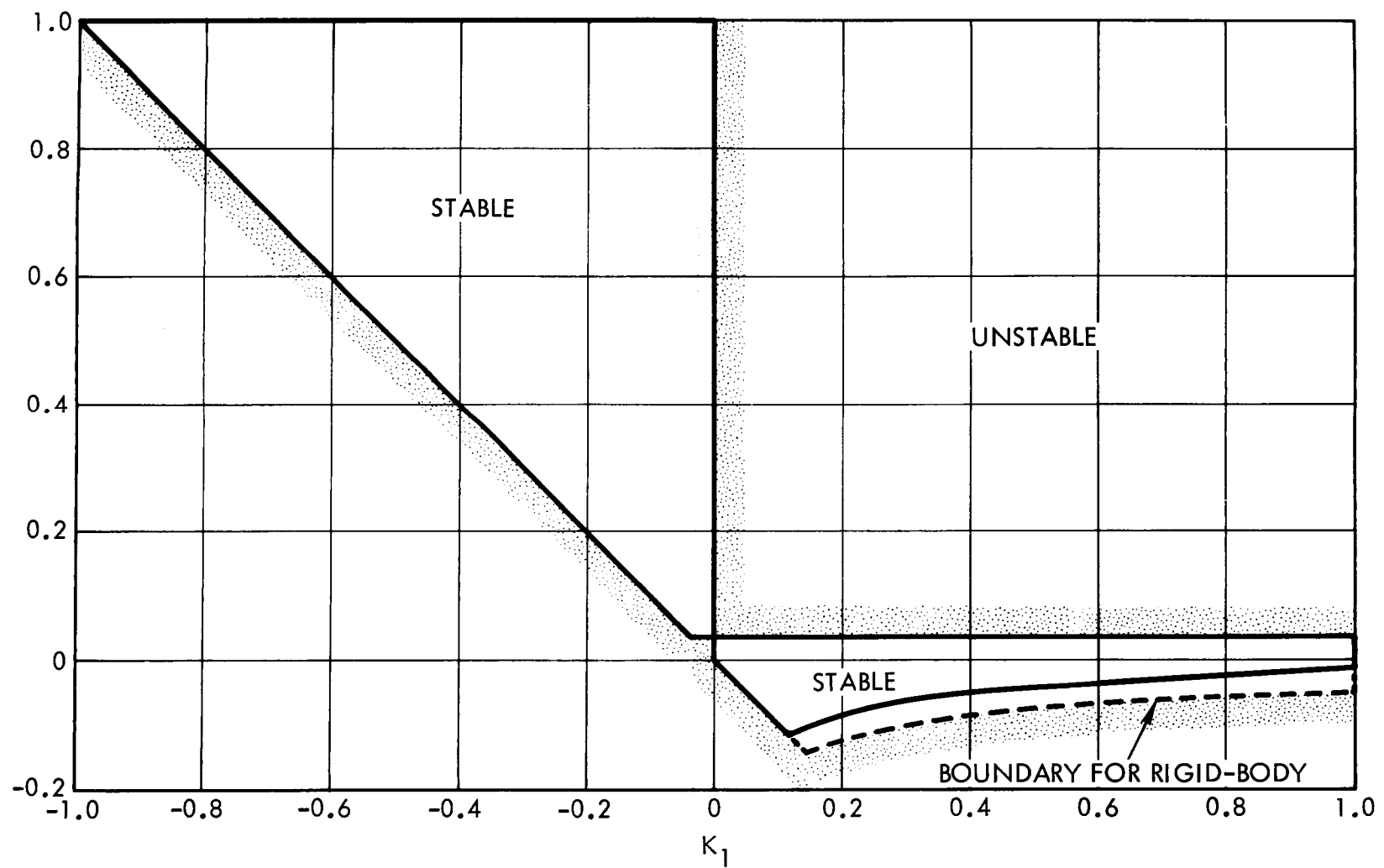
Figure 3.11. Regions of Infinitesimal Stability for \omega_n = 10
