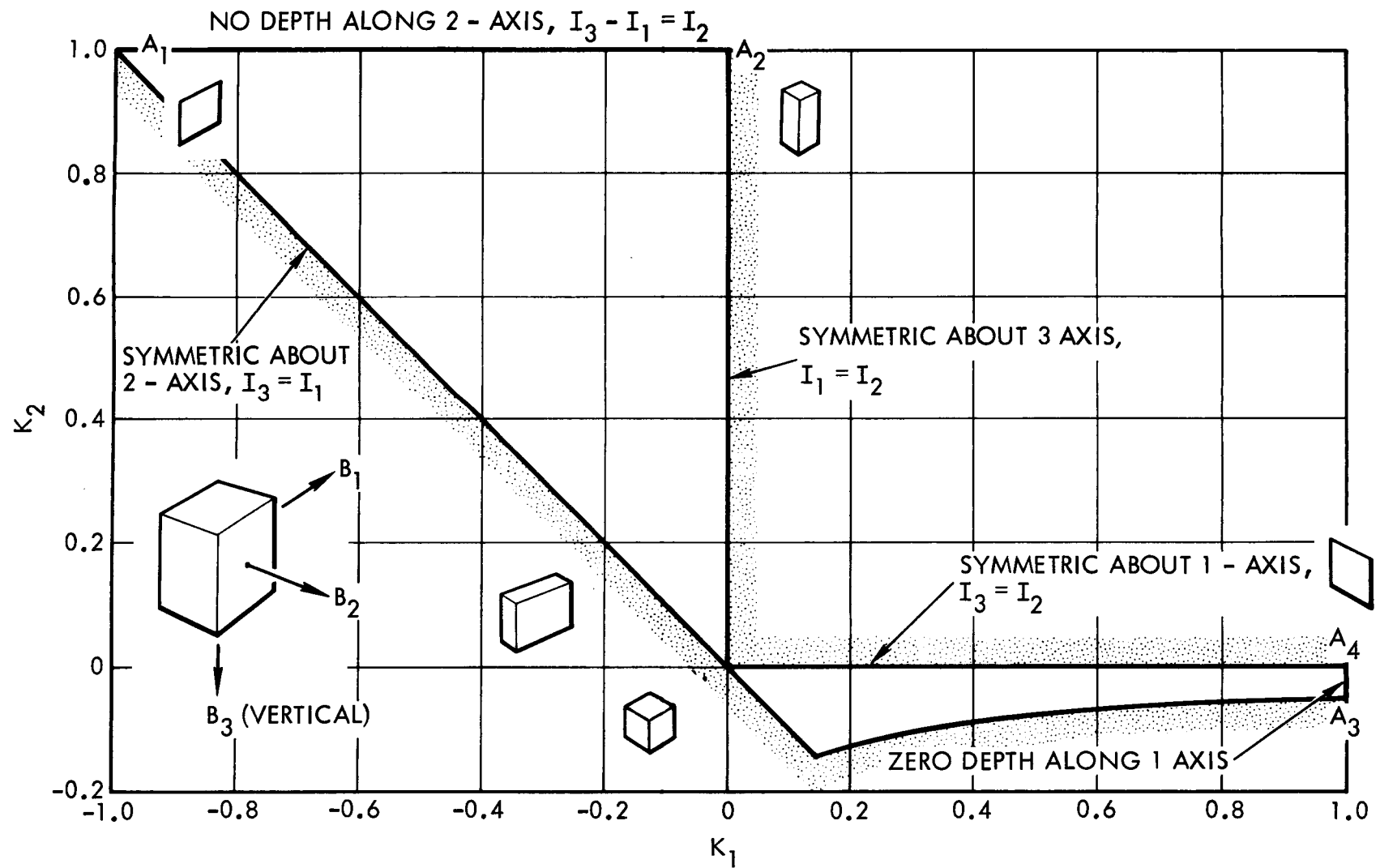
Figure 3.4. Physical Character of Satellites in Various Regions of K_1 - K_2 Plane
