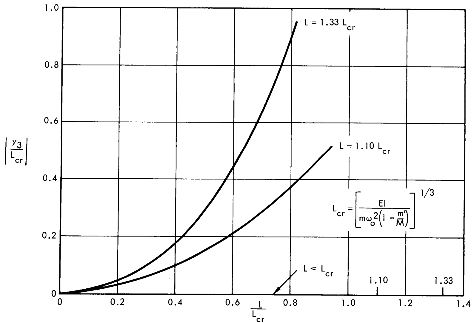
Figure 4.4. Equilibrium Shapes of Weightless Cantilever With Tip Mass, as a Function of Beam Length
