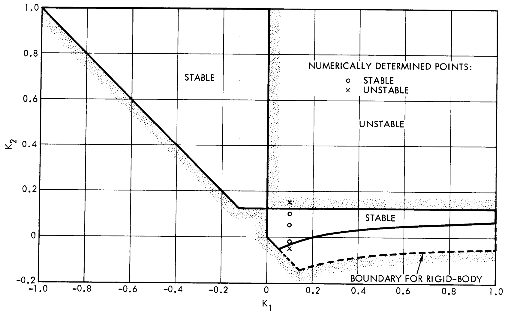
Figure 3.12. Regions of Infinitesimal Stability for \omega_n = 5
