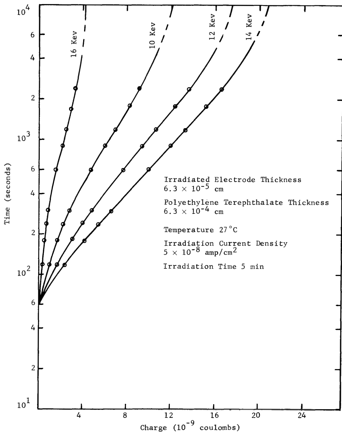
Figure 2.5. External Charge Transfer from Thermal Release of Trapped Irradiation Electrons for the Indicated Primary Electron Energies.
