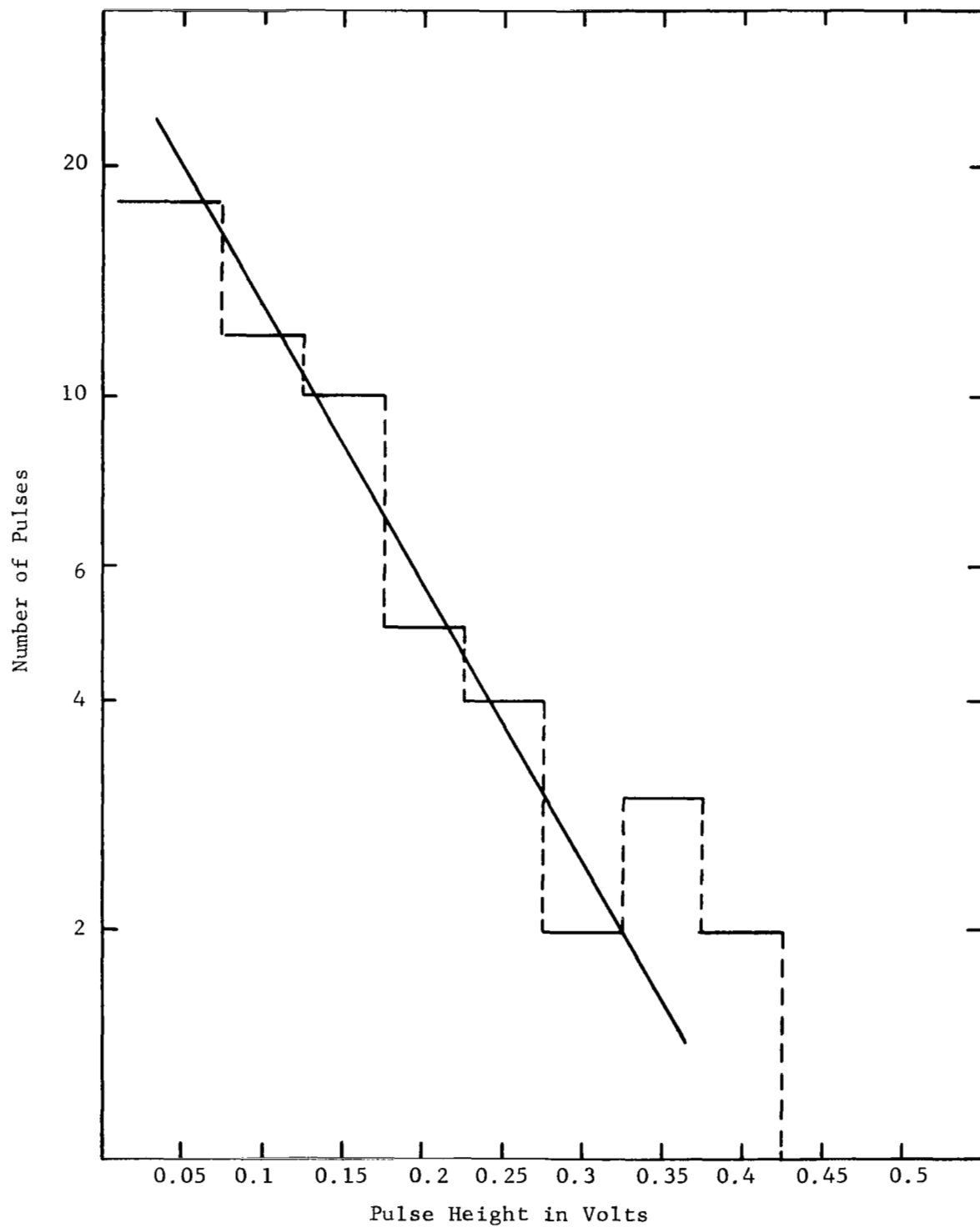
Fig. 3.10. Pulse Height Distribution from Spontaneous Discharge of Electron Irradiated Polyethylene Terephthalate Film.
