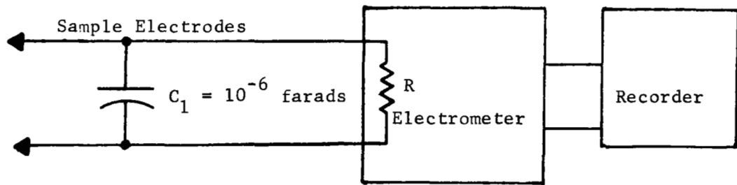
Figure 2.4. Circuit used to Measure External Charge Transfer Resulting from Thermal Release of Trapped Electrons.
