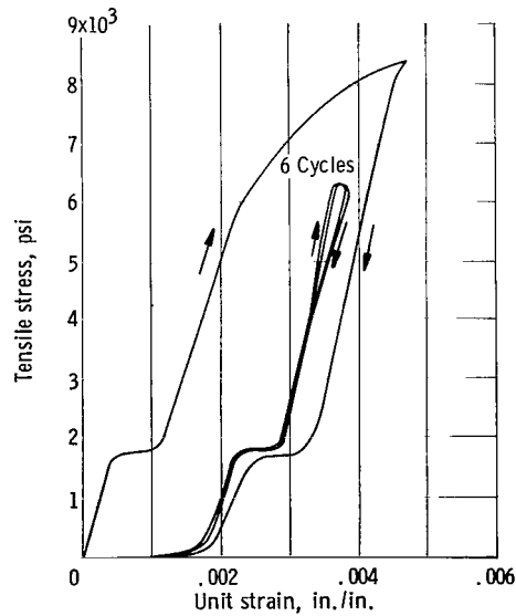
Figure 8. - Stress-strain curve of AMA laminate showing six loading cycles after an initial stress of 8300 pounds per square inch. Temperature, -300^{\circ}\text{F} .
