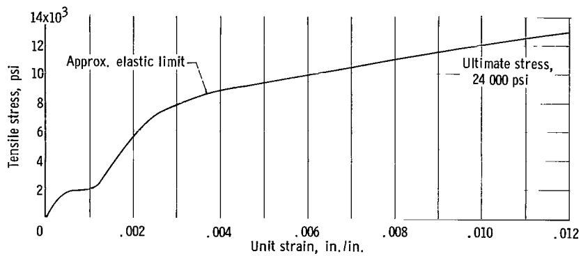
Figure 7. - -300^{\circ}\text{F} stress-strain curve for AMA laminate (0.0007 in. aluminum, 0.001 in. Mylar, 0.0007 in. aluminum).
