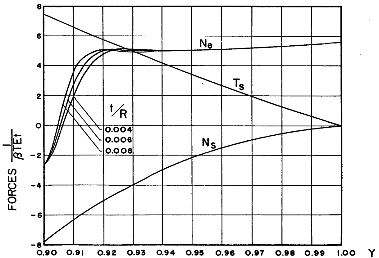
FIG. 8 MEMBRANE FORCES N_\theta , T_s AND N_s ( N=2 )
