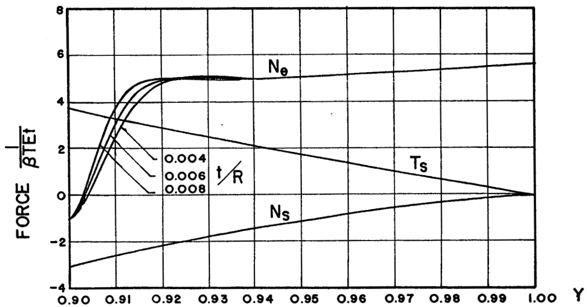
FIG. 2 MEMBRANE FORCES N_\theta T_s AND N_s ( N=1 )
