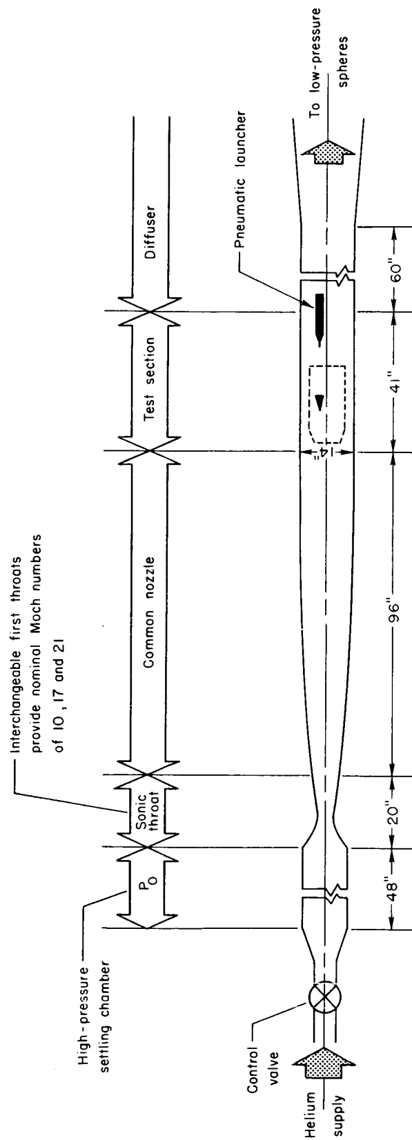
Figure 6.- Schematic of the Ames 14-Inch Helium Tunnel.
