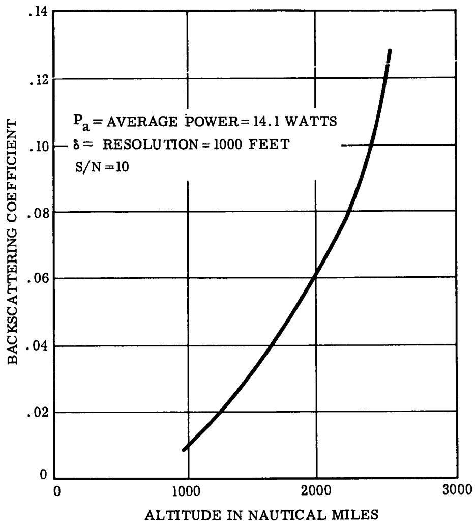
Figure 3.3.1-13. Backscattering Coefficient vs. Altitude
