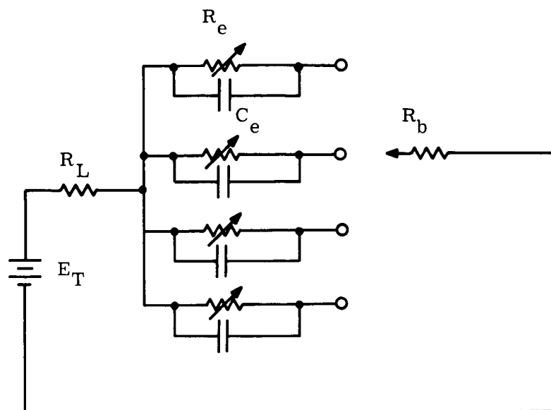
Figure 2.3.2-1. Equivalent Circuit
