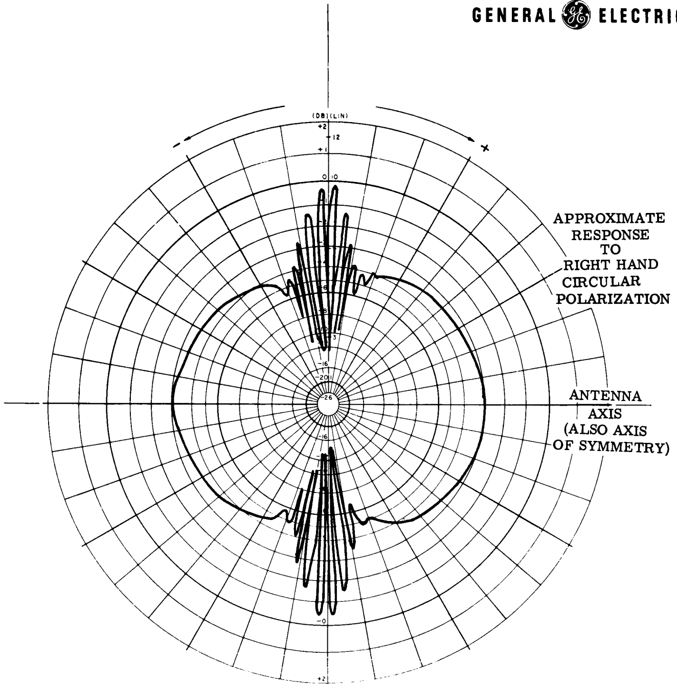
Figure 1.7.2-5. Pattern of Antennas of Figure 1.7.2-2
