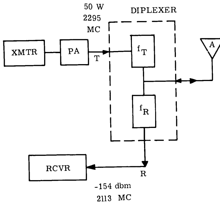
Figure 1.7.5-1. S-Band Diplexer
