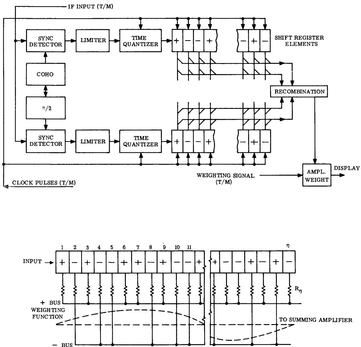
Figure 3.3.1-7. Shift Register Data Processor and Weighted Shift Register Chain
