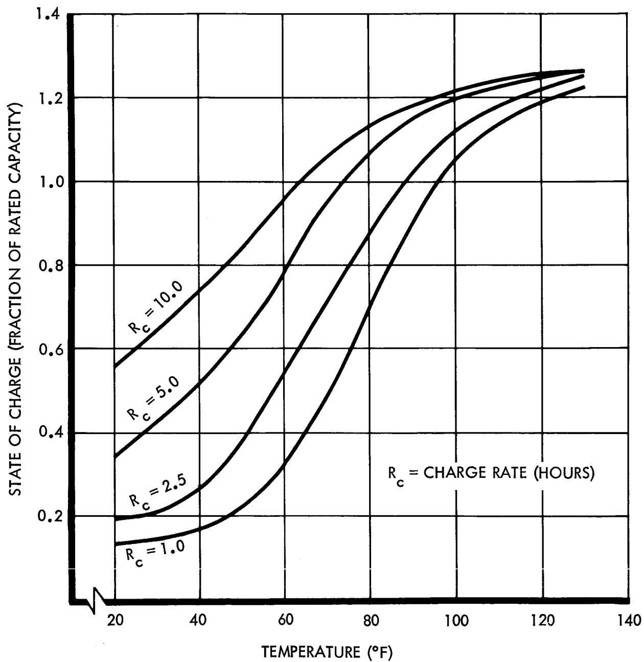
Figure 2-9. Silver-Cadmium Cells. Maximum State of Charge versus Temperature (Charge Rate is the Parameter.)
