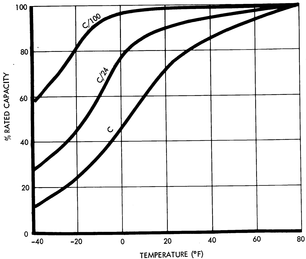
Figure 2-2. Silver-Zinc Cells, Effect of Temperature on Capacity to 1.0 Volt (Discharge Rate is the variable parameter)
