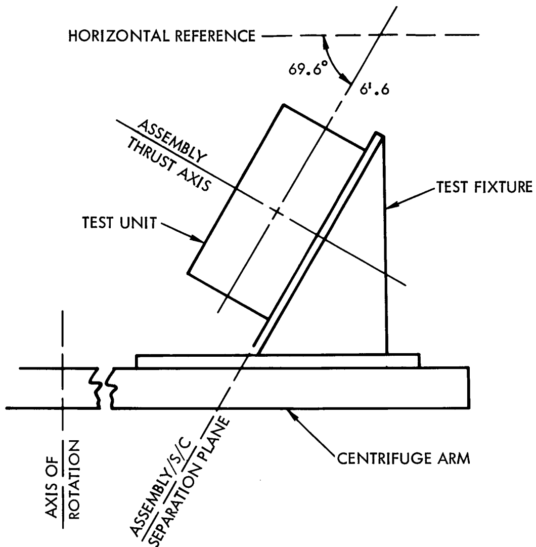
Figure 3-8. Unit Orientation, Linear Acceleration Test
