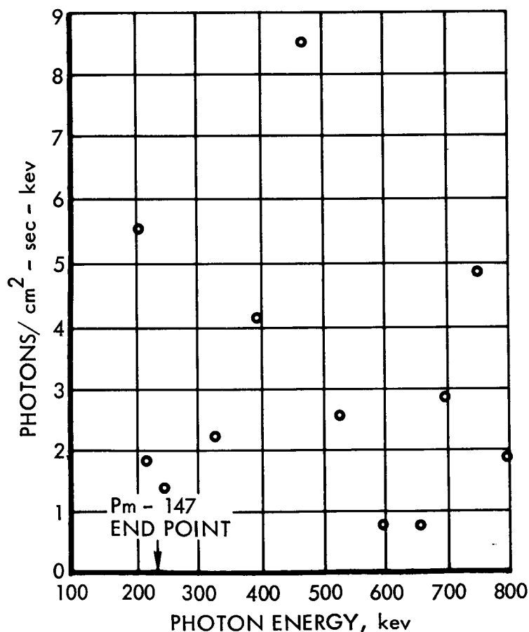
Figure 3-15. Differential Number-Energy Spectrum of the Observed Contaminants in a 1-Watt Pm-147 Source at a Distance of 1 m (Ref. 1)
