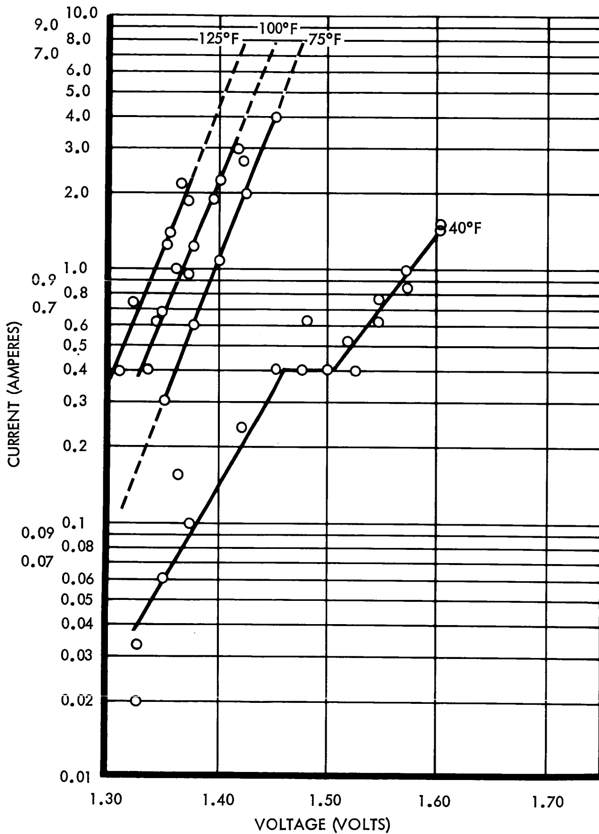
Figure 2-15. 20AH Nickel-Cadmium Cells, Effects of Voltage and Temperature on Steady-State Overcharge Current
