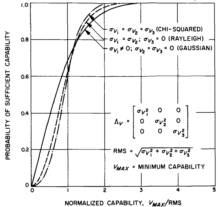
Fig. 4. Probability of sufficient capability
