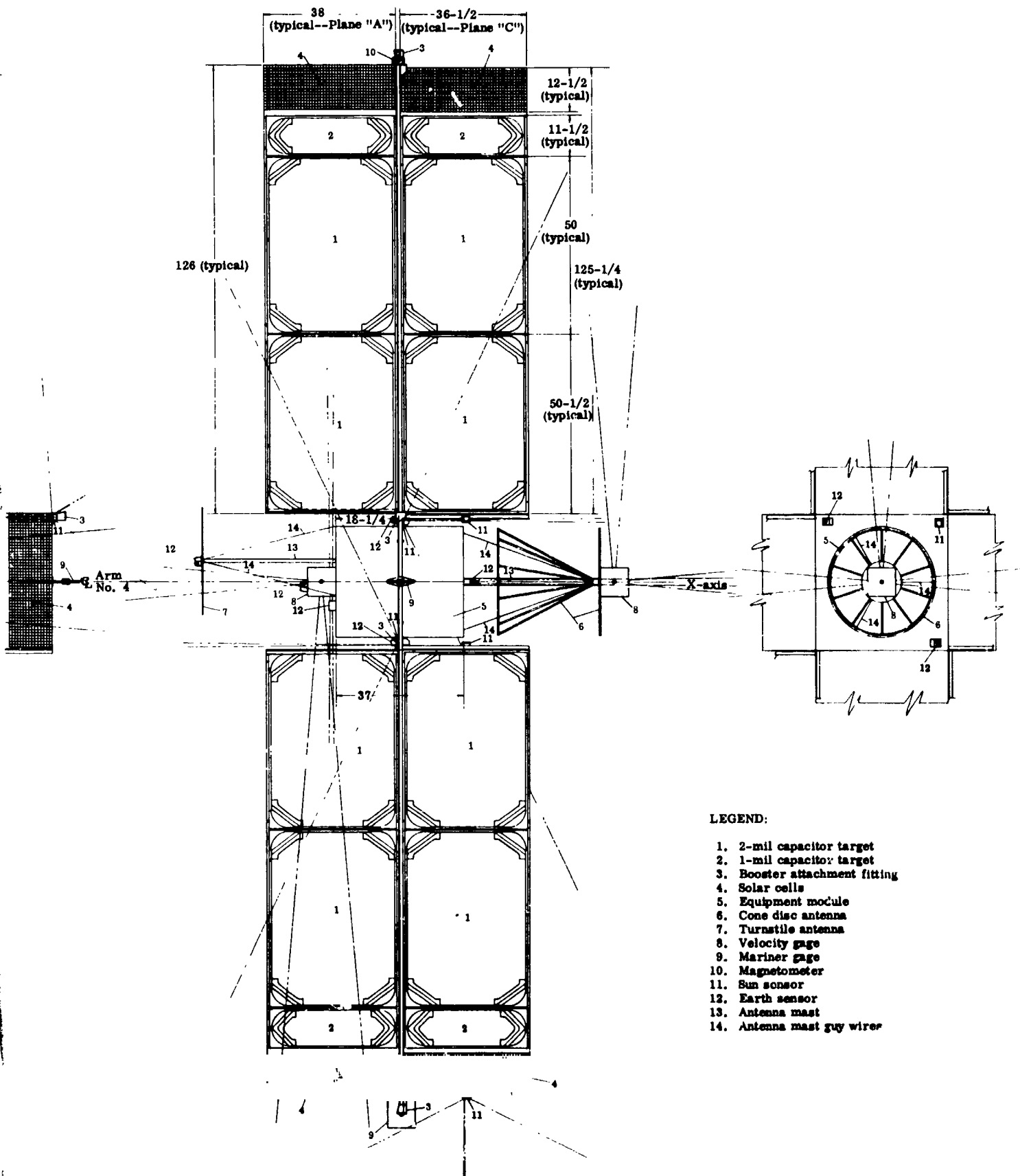
Fig. I-9. M100 General Arrangement
