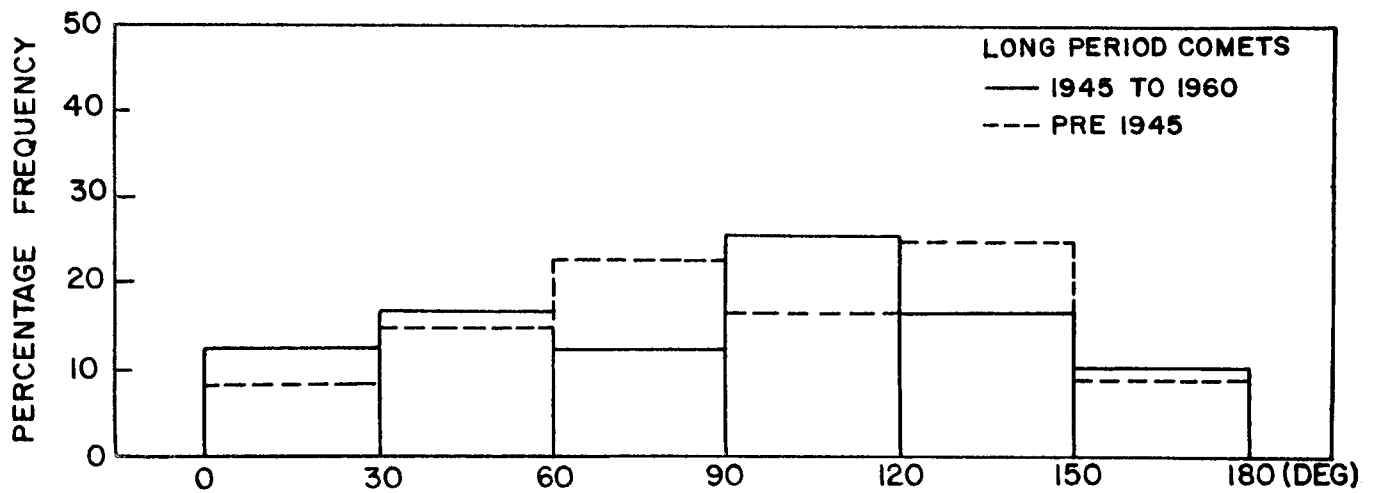
FIG. 2 FREQUENCY DISTRIBUTION FOR INCLINATION OF LONG PERIOD COMET SAMPLES
