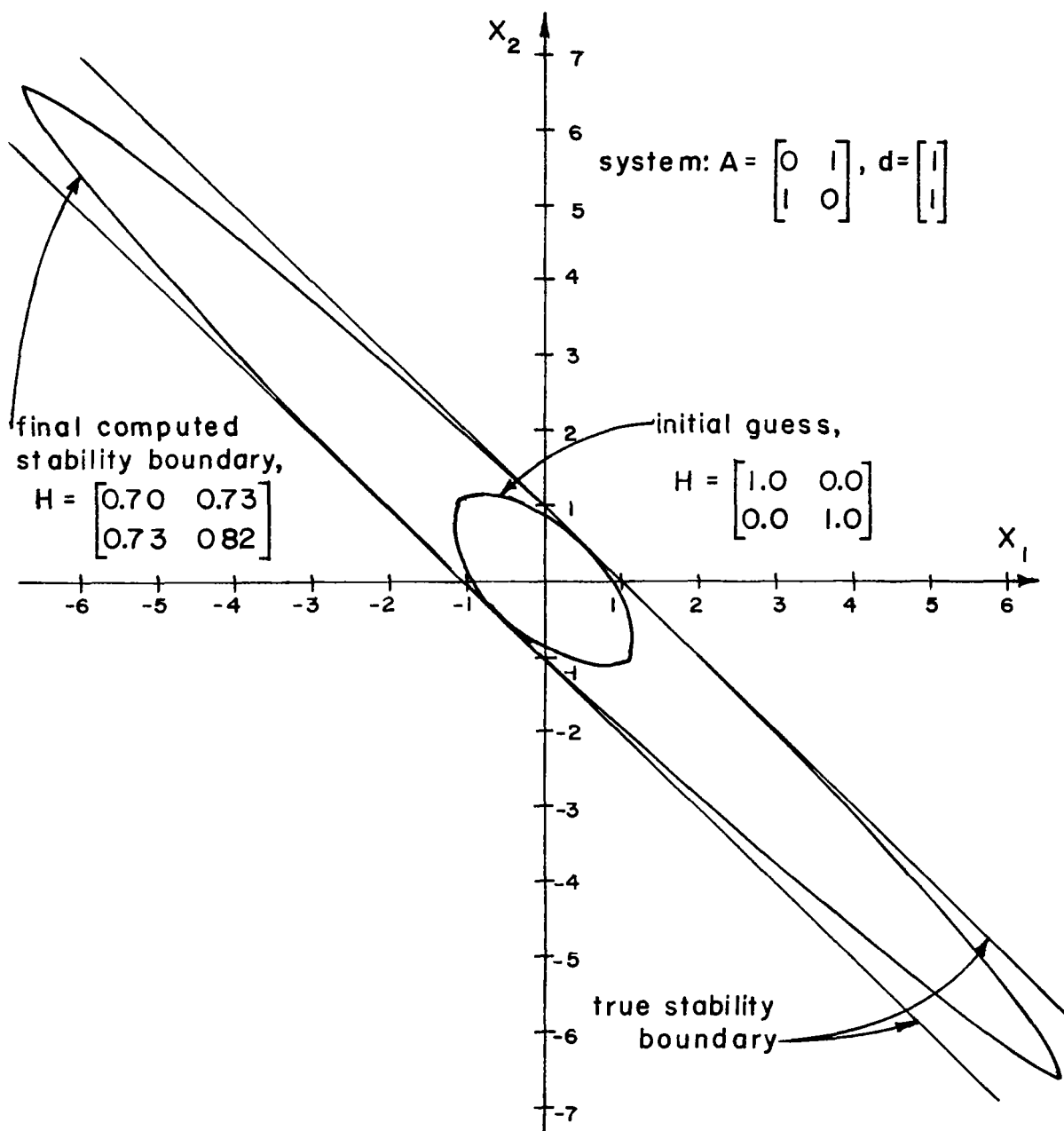
Fig. 4-10 Stability Boundaries for Example 4-5.
