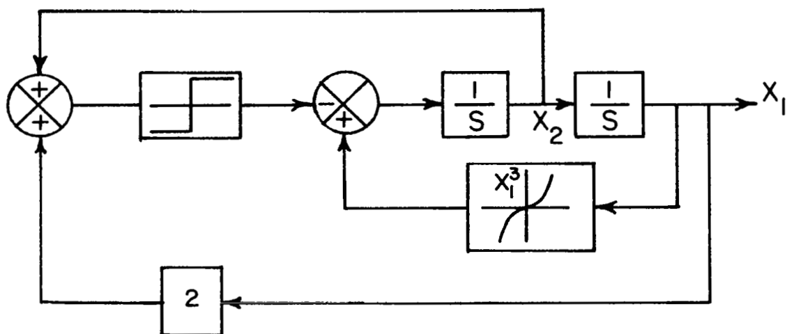
Fig. 4-11 The System with Non-linear Plant of Example 4-6.
