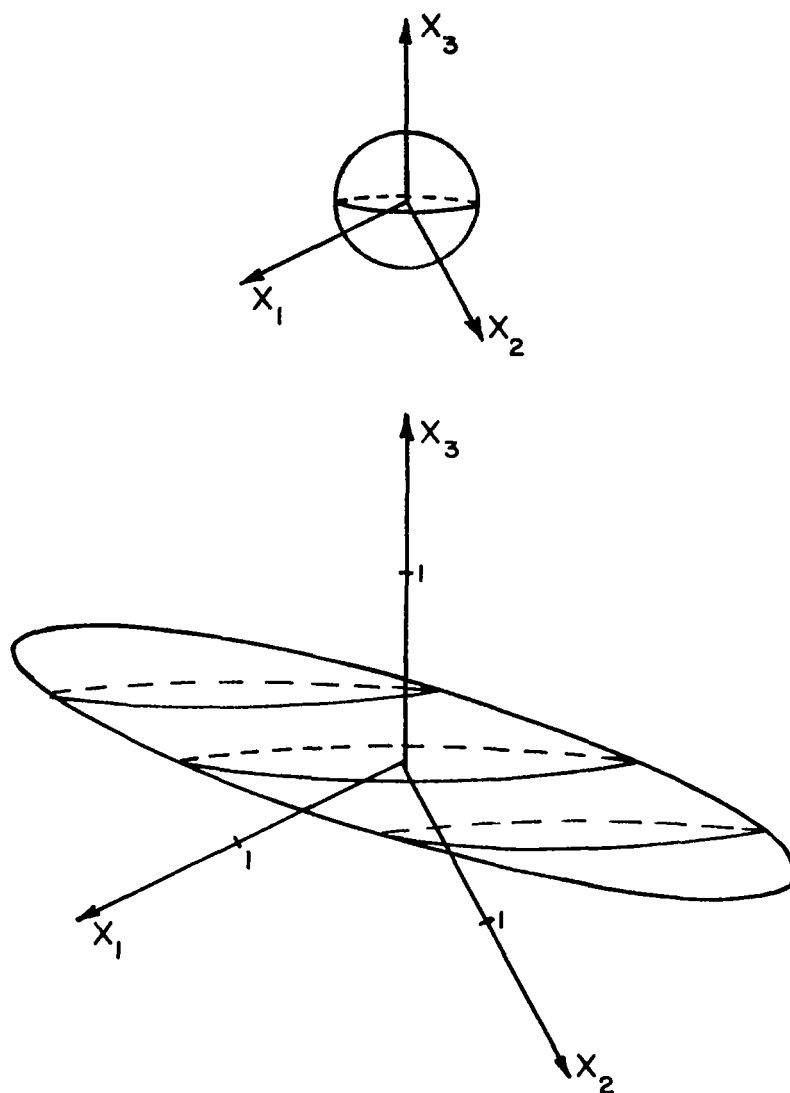
Fig. 4-15 Initial and Computed Stability Boundaries of Example 4-8.
