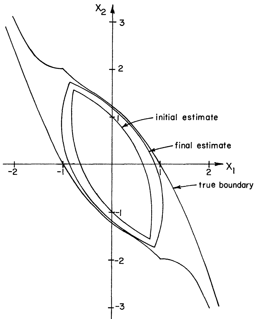
Fig. 4-12 Stability Boundaries for Example 4-6.
