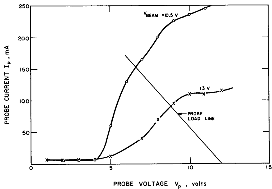
FIG. 15 "PLASMA BRIDGE" PROBE CHARACTERISTICS
