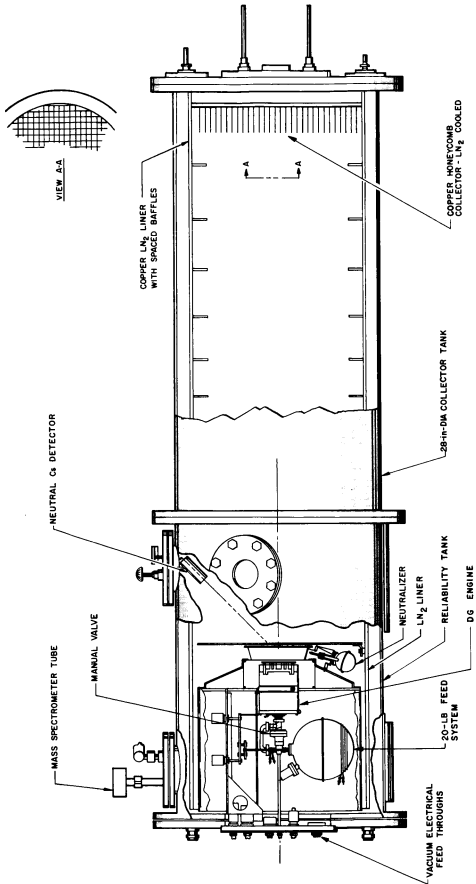
FIG. 6 THE 2000-HOUR ENGINE SYSTEM
