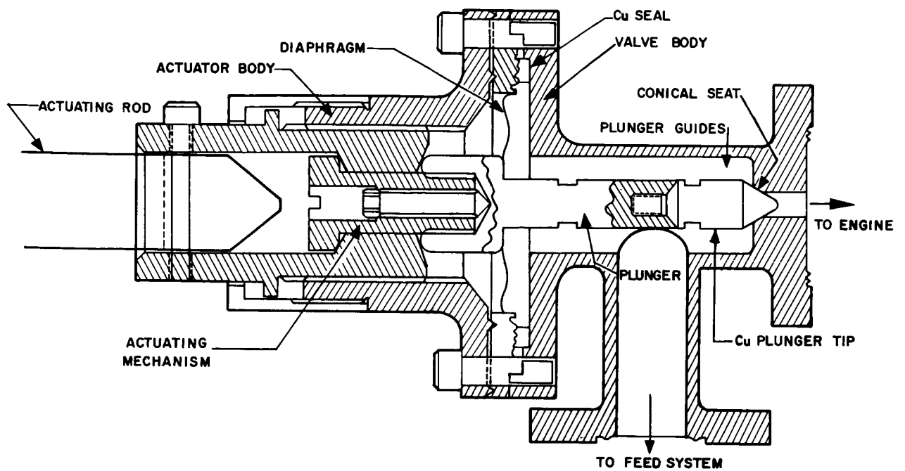
FIG. 9 MANUAL VALVE
