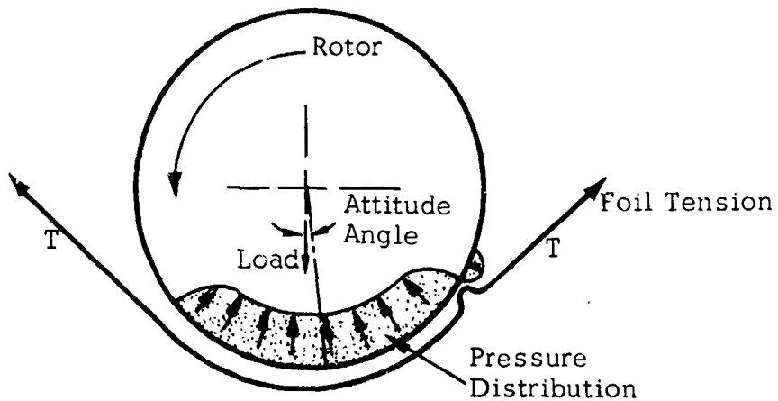
Self-Acting Foil Bearing
