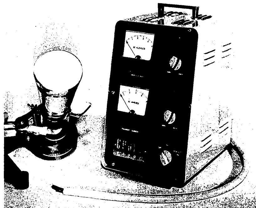
Fig. 17 - Field Emission Microscope Tube (Not Mounted) and Power Supply Which Can Heat the Tip While an Emission Pattern is Being Viewed
