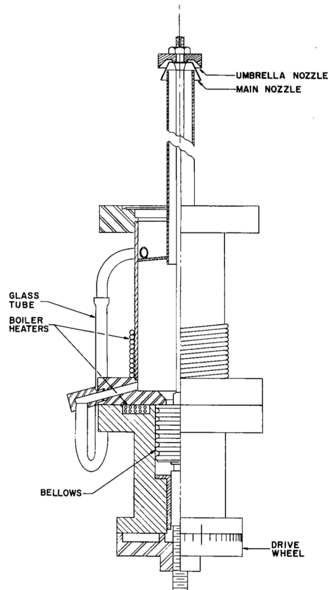
Fig. 1 - Diagram (Right) and Photograph (Left) of a Special Test Apparatus for Evaluation of Experimental Diffusion Pump Nozzles. A Dual Expansion Nozzle is Shown. The Drive Mechanism Provides for Continuous Variation of Nozzle Gap During Operation.
