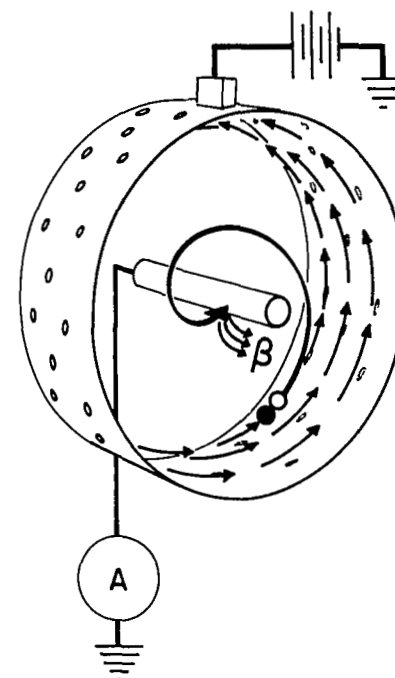
Fig. 11 - Basic Configuration of Magnetron Pressure Gauge. Ions and Cathode Generated Electrons Are Measured by the Ammeter, A . The Ions Are Formed by Gas Impacts with the Electron Cloud Near the Anode. Cesium Raises the Escape Probability \beta for Avalanche Initiating Electrons.
