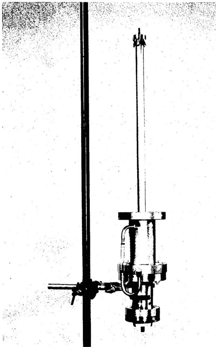
Fig. 1 - Diagram (Right) and Photograph (Left) of a Special Test Apparatus for Evaluation of Experimental Diffusion Pump Nozzles. A Dual Expansion Nozzle is Shown. The Drive Mechanism Provides for Continuous Variation of Nozzle Gap During Operation.
