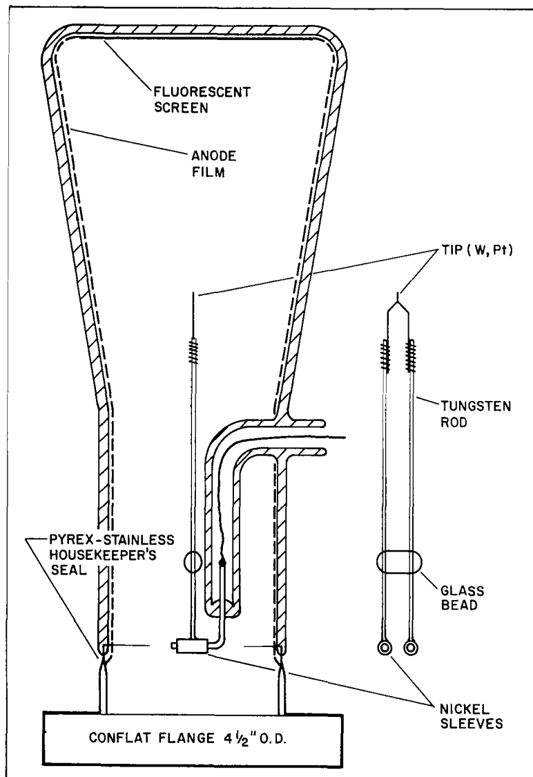
Fig. 16 - Field Emission Microscope Tube Details. Tip Assembly and Support Rods Are Easily Removed from Press Fit Mountings.
