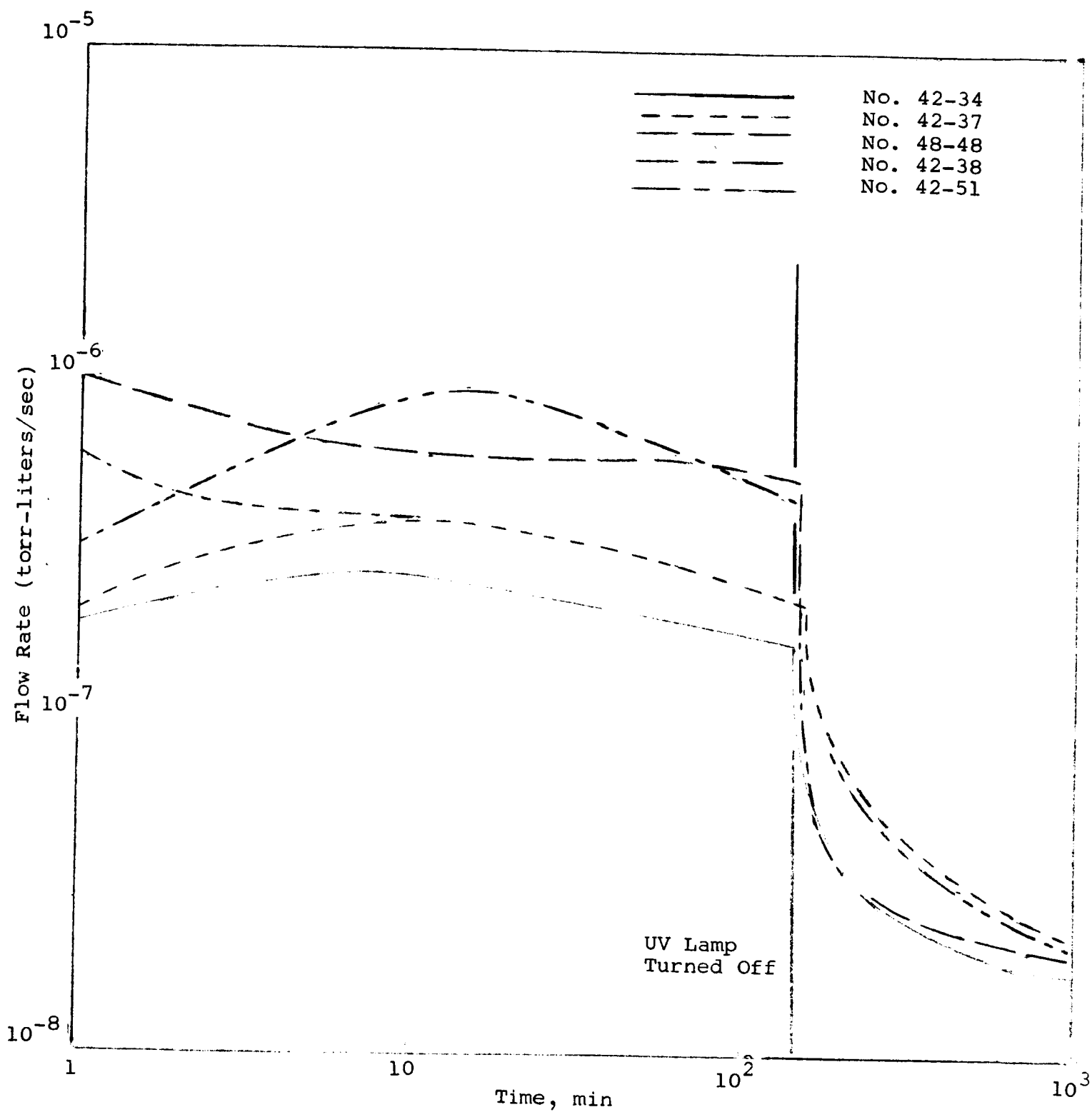
Figure 2 OUTGASSING OF CANDIDATE COATINGS
