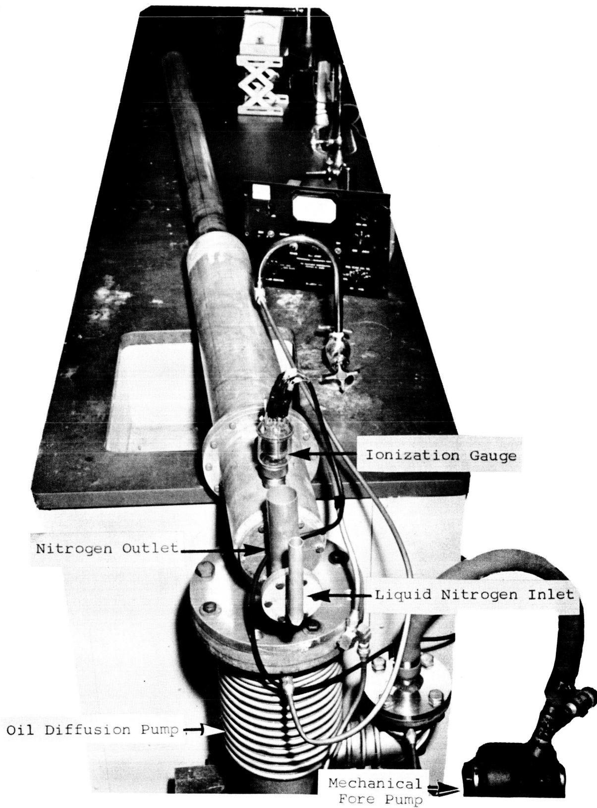
Figure 3 NUCLEAR EXPOSURE FIXTURE
