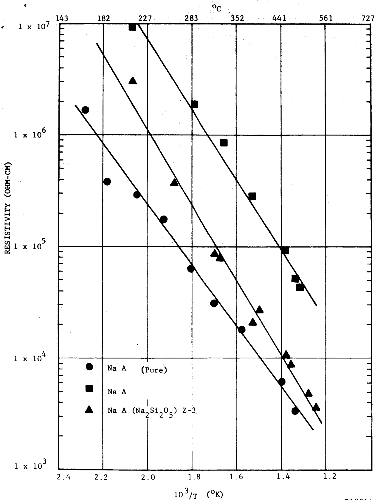
FIGURE 31. EFFECT OF H 3 PO 4 AND Na 2 Si 2 O 5 BINDERS ON RESISTIVITY OF NaA ZEOLITES
