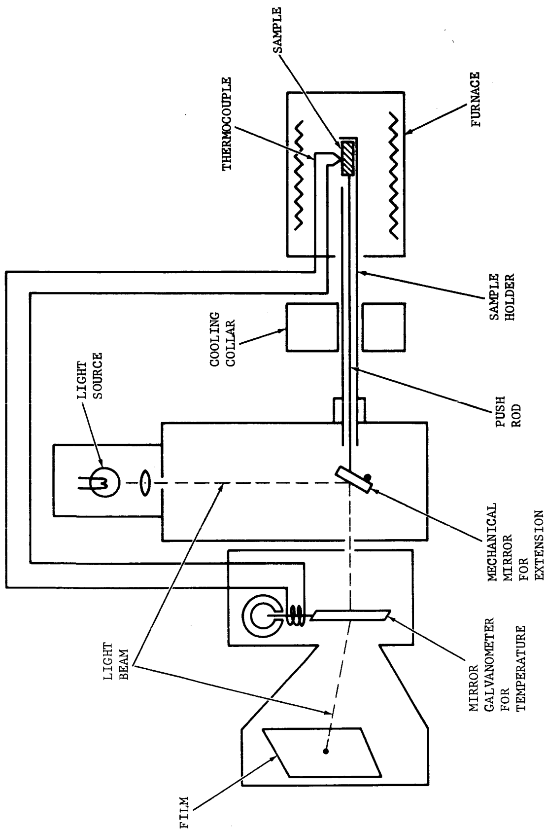
FIGURE 24. JET DILATOMETER
