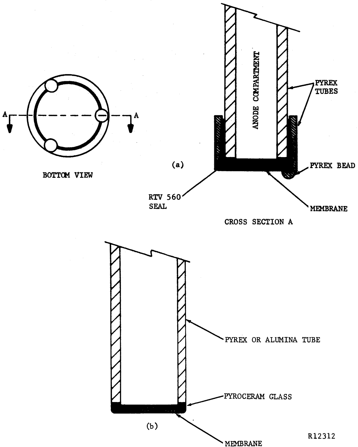
FIGURE 38. ANODE COMPARTMENTS
