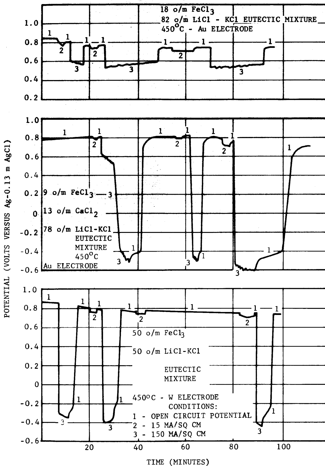
FIGURE 20. \text{FeCl}_3 REDUCTION. EFFECT OF DILUENT AND ELECTRODE
