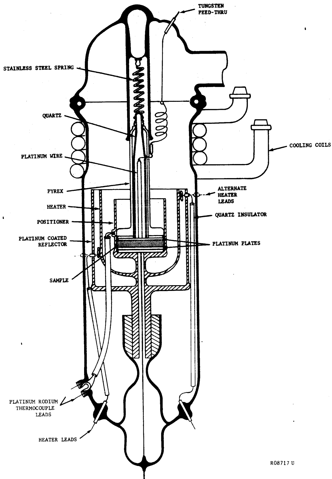
FIGURE 27. CONDUCTIVITY CELL
