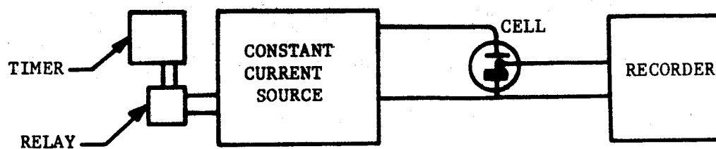
FIGURE 3. BLOCK DIAGRAM OF APPARATUS FOR POLARIZATION STUDIES
