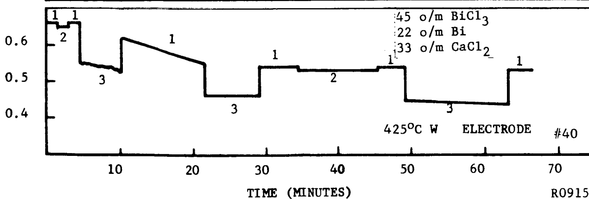
FIGURE 13. BiCl 3 REDUCTION. EFFECT OF DILUENT, TEMPERATURE, AND ELECTRODE
