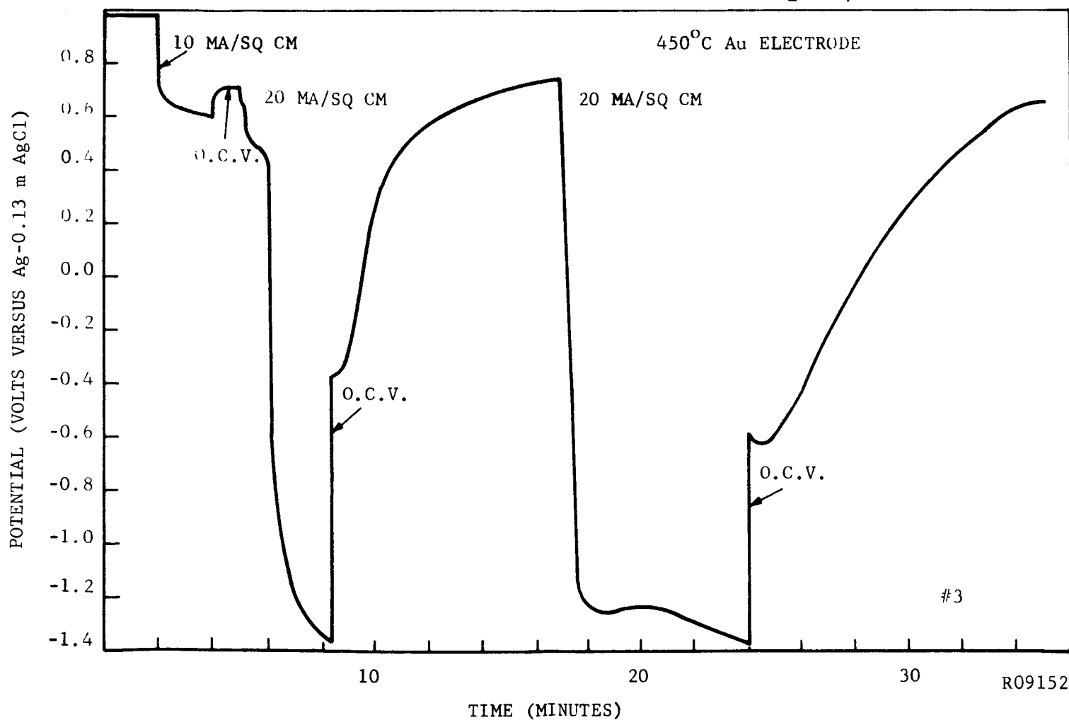
FIGURE 17. REDUCTION OF MOLTEN K_2Cr_2O_7
