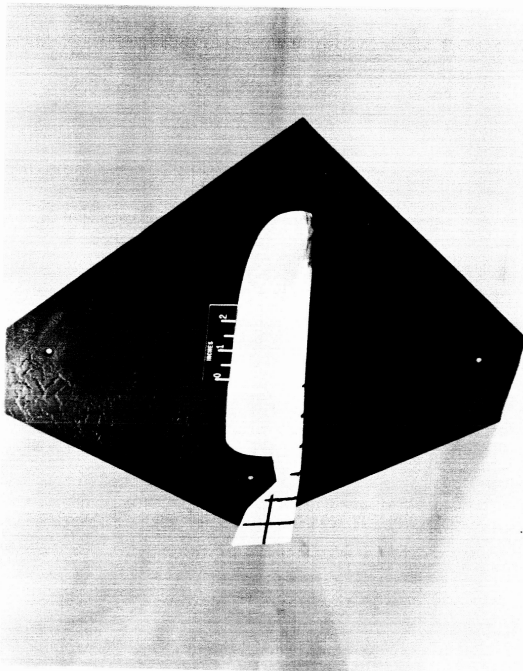
(a) Supersonic test. M = 3.0 . L-59-2014
