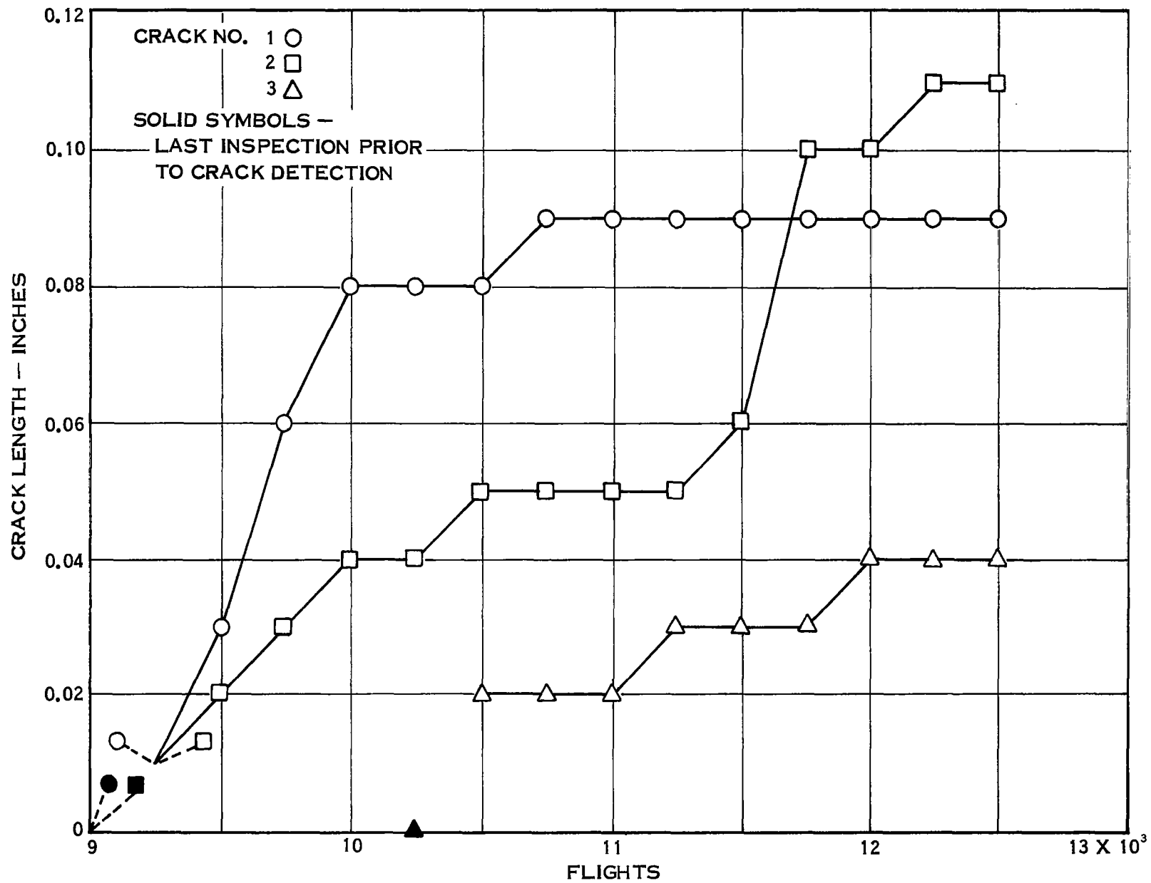
Figure 30. Crack Propagation Curves for All Cracks, Test Specimen Number 8
