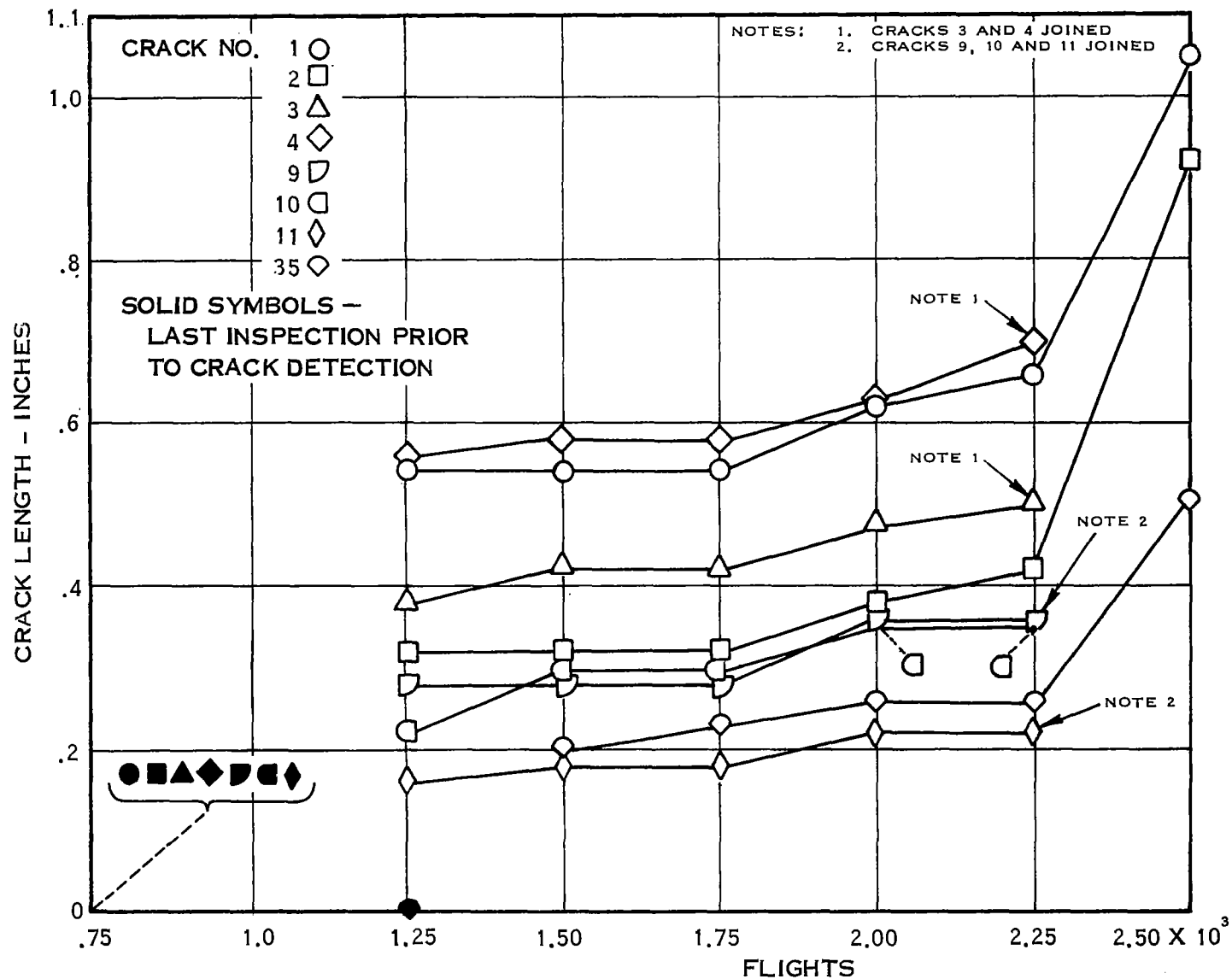
Figure 26. Crack Propagation Curves for Selected Cracks, Test Specimen Number 4
