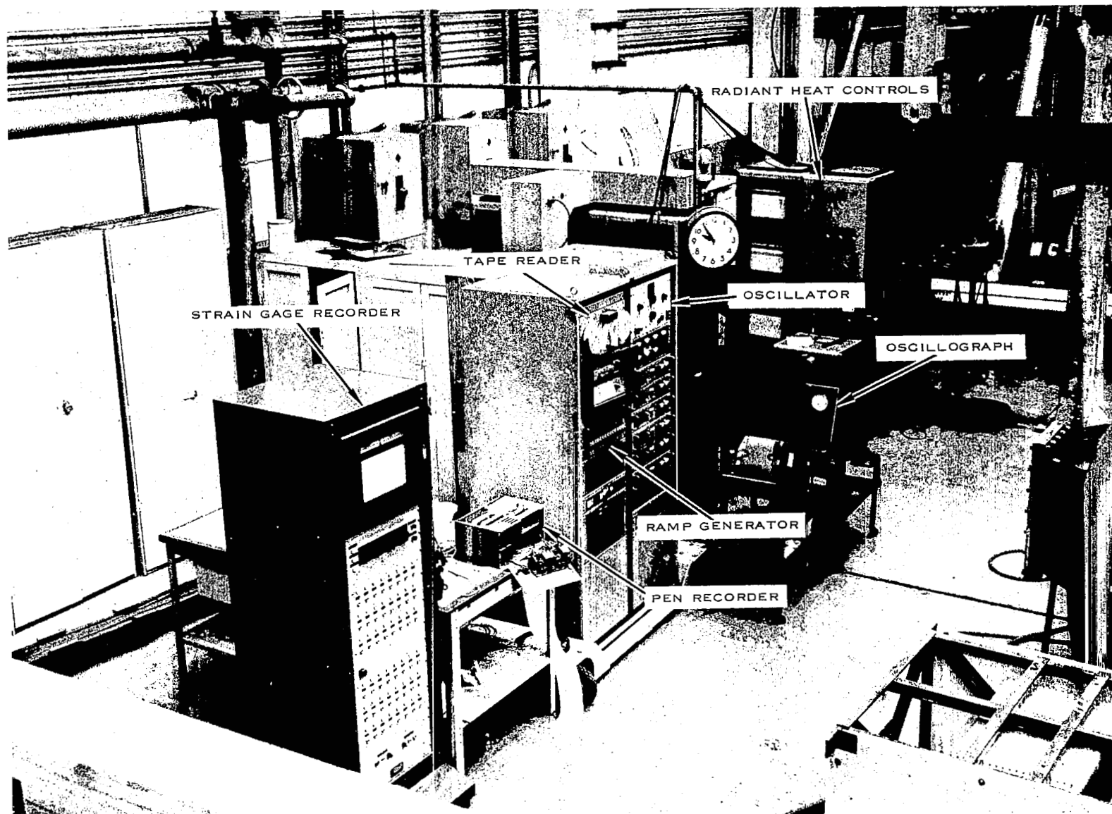
Figure 10. Overall View of Control Equipment
