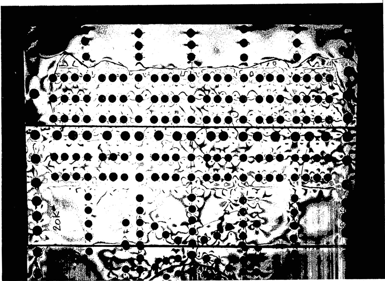
Figure 12. Photostress Evaluation, Box Beam Number 1. View Showing Isochromatics Around Centerline Splice
