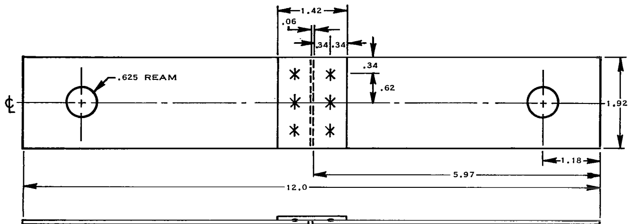
TYPE 2 - LOAD CARRYING SPOTWELD SPECIMEN
