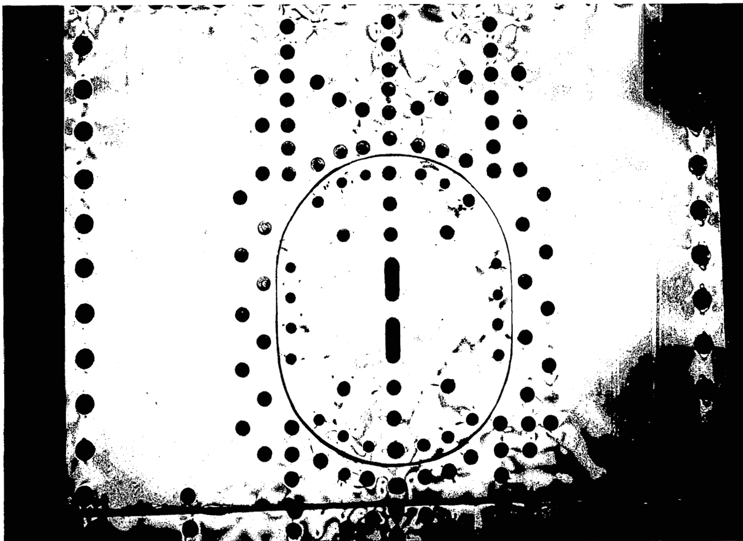
Figure 11. Photostress Evaluation, Box Beam Number 1. View Showing Isochromatics Around Structural Door
