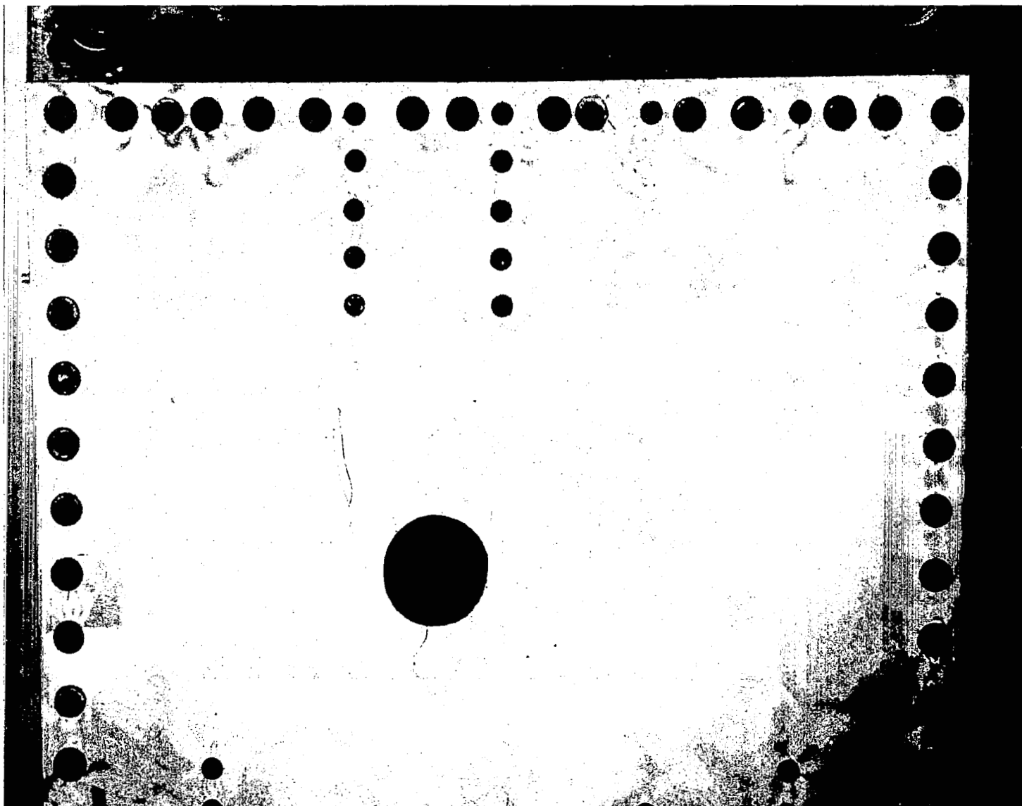
Figure 13. Photostress Evaluation, Box Beam Number 1. View Showing Isochromatics Around Circular Cut-out
