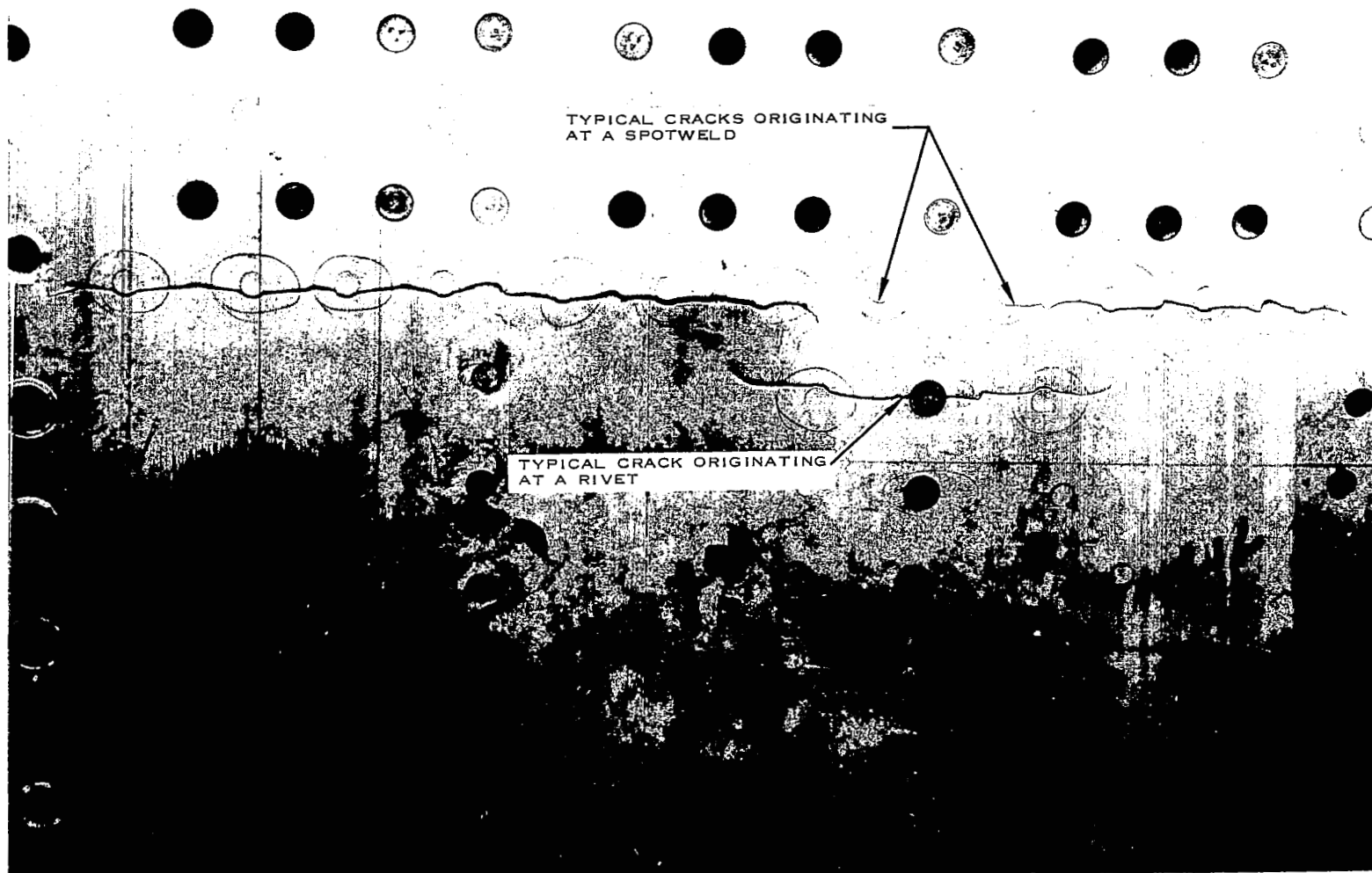
Figure 16. Photo Showing Typical Cracks Around Rivets and Spotwelds. Number 4 Test Skin
