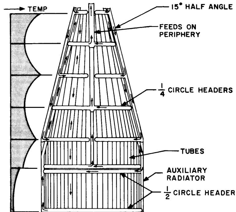
Figure 4-10. Axial Flow and Temperature Profiles
