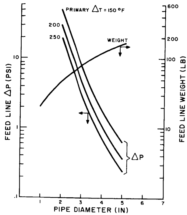
Figure 7-5. Primary Loop Piping Weight and Pressure Drop
