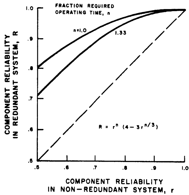
Figure 3-6. Probability of No More Than One Failure in Four Parallel Systems Accounting for Size Effects
