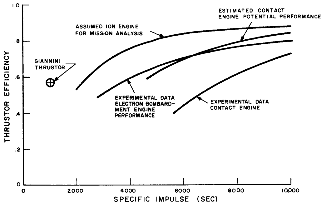
Figure 9-3. Efficiency of Candidate Thrustors
