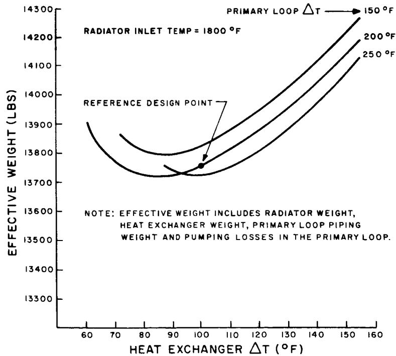
Figure 7-8. Optimization of Heat Exchanger \Delta T
