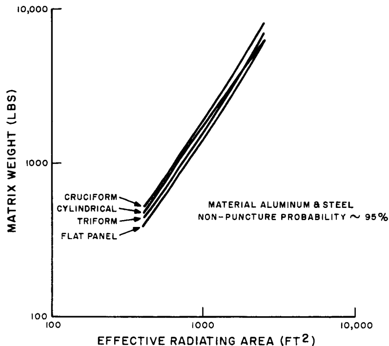
Figure 4-8. Matrix Weight versus Effective Radiating Area
