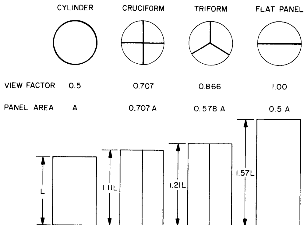
Figure 4-5. Comparison of Fixed Radiator Arrangements
