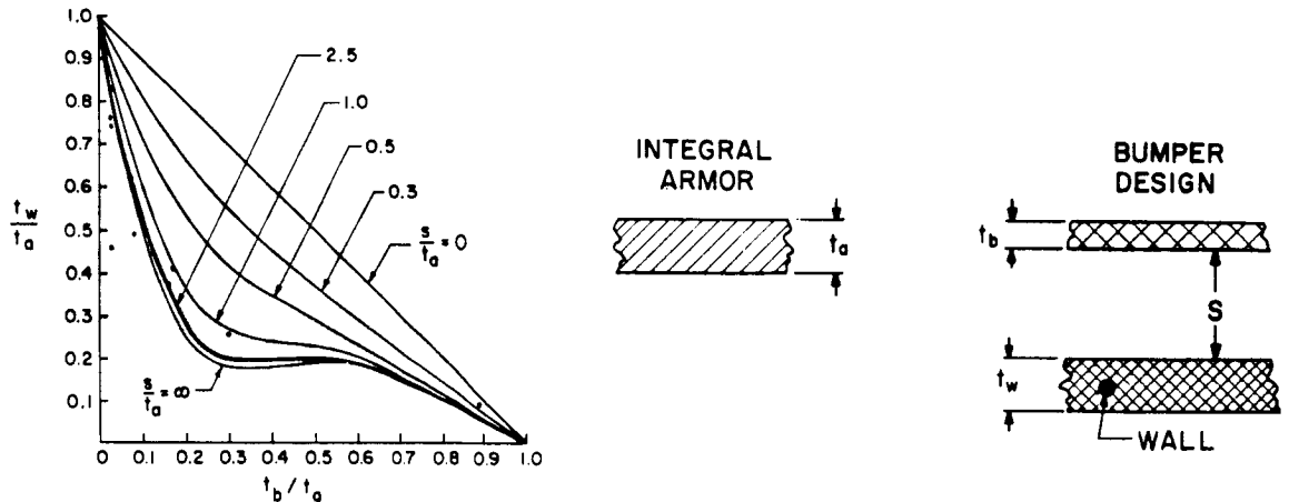
Figure 5-6. Meteoroid Bumper Criterion
