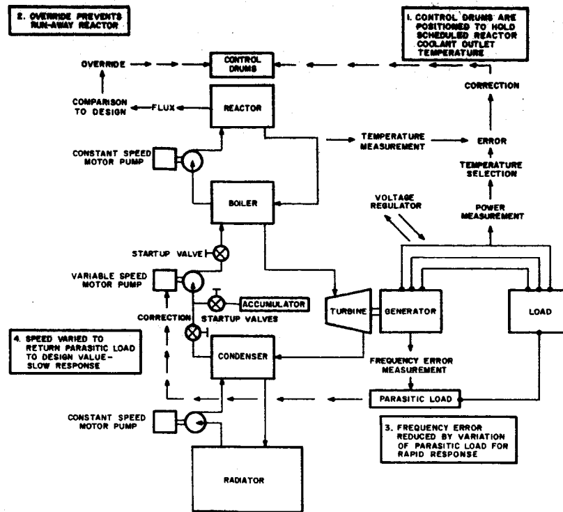
Figure 6-4. Conceptual View of Powerplant Controls
