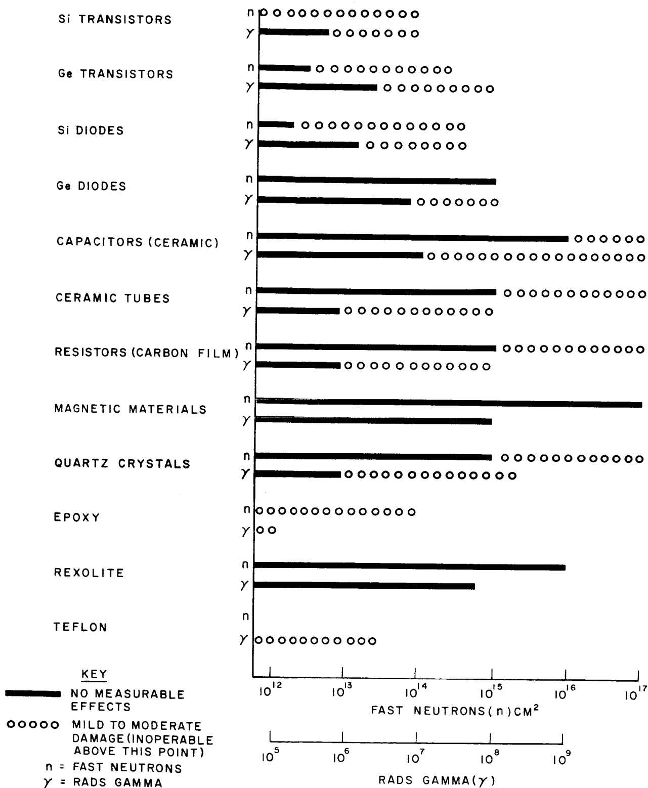
Figure 6-14. Gamma and Neutron Threshold Radiation Tolerance
