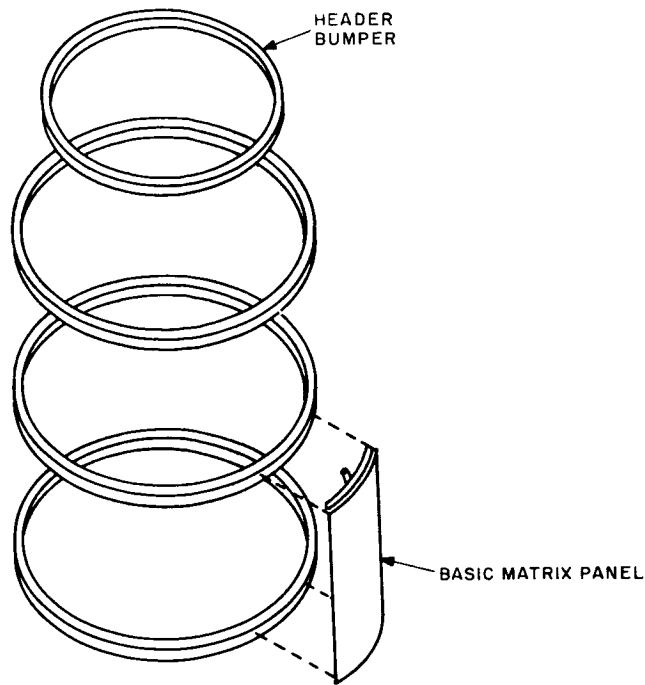
Figure 5-9. Fabrication Techniques
