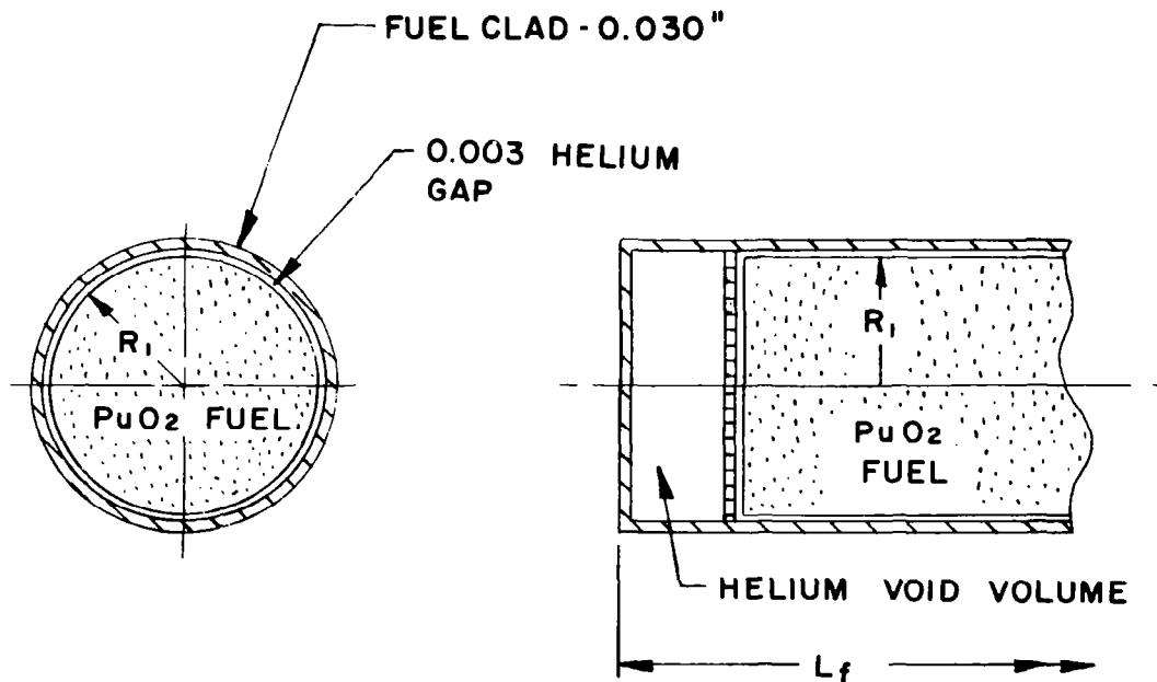
Figure 5-20. Fuel Capsule
