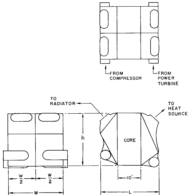
Figure 6-28. Recuperator
