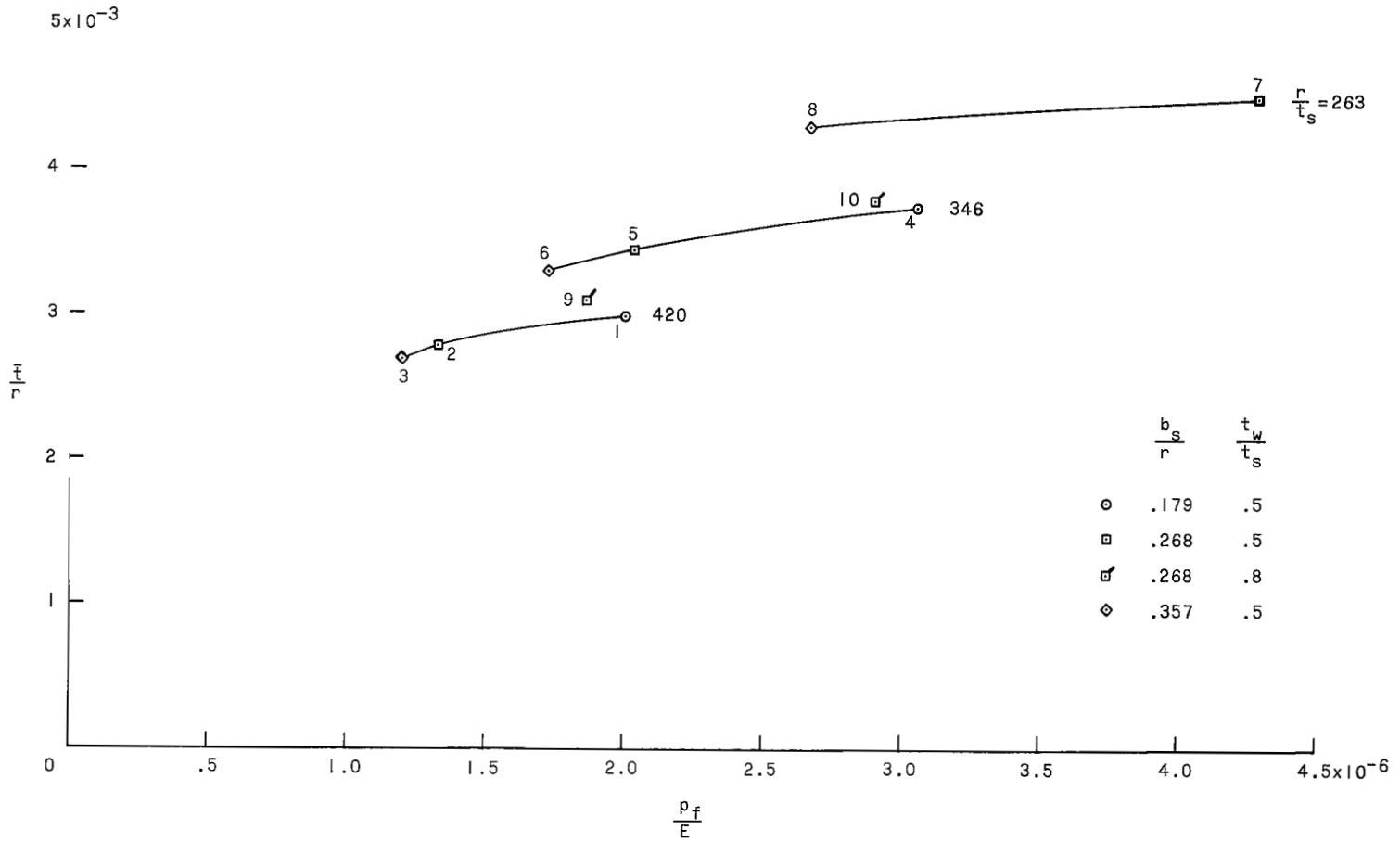
Figure 8.- Structural efficiency plot of collapse pressures of cylinders. L/r = 1.214 ; L = 17.0 in. (43.2 cm); numbers beside test points are cylinder numbers.
