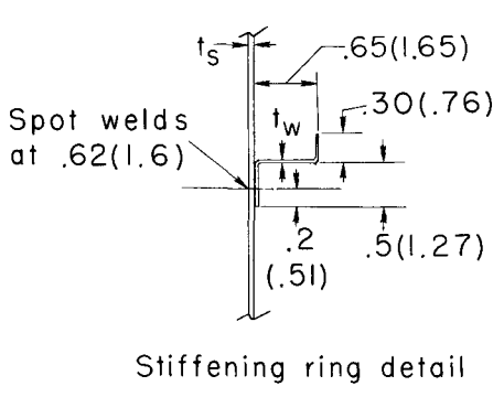
Figure 1.- Dimensions of cylinders. All dimensions are in inches (centimeters). (See table I.)
