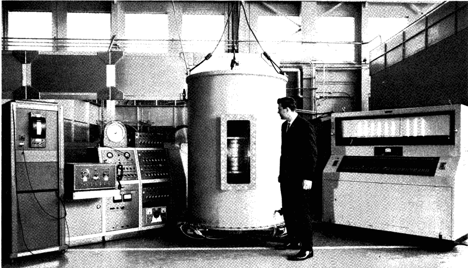
Figure 2.- General view of test setup showing a cylinder in the pressurizing tank.
