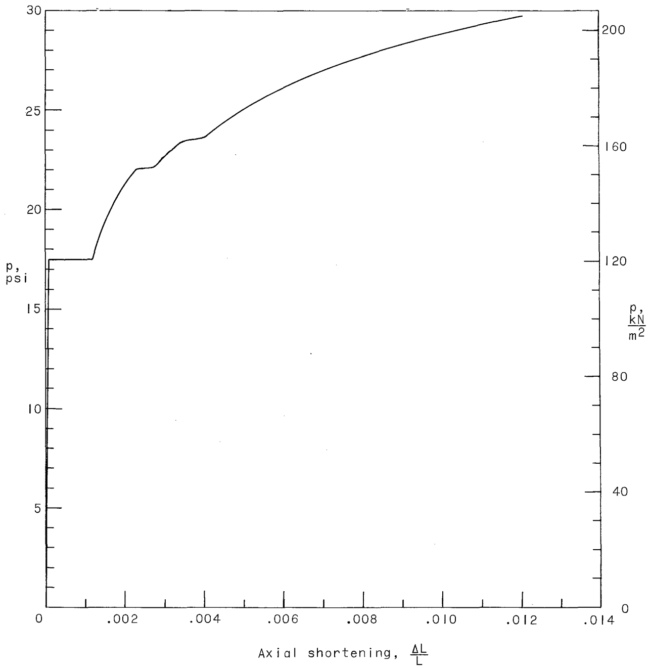
Figure 7.- Curve showing axial shortening with pressure for one of the axial shortening devices on cylinder 10.
