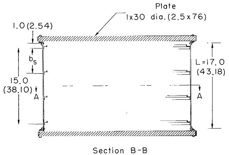
Figure 1.- Dimensions of cylinders. All dimensions are in inches (centimeters). (See table I.)
