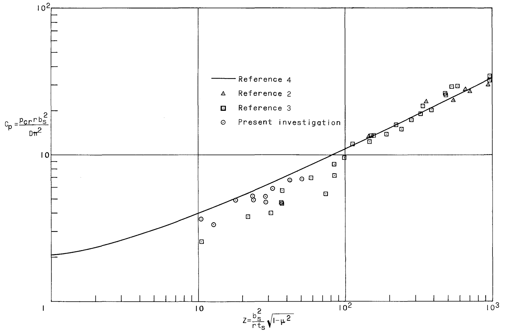
(a) 1 \leq Z \leq 10^3 ; test data from present investigation and references 2 and 3.
