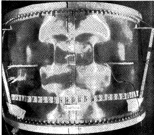
(e) Cylinder with very deep buckles. Pressure, 29.6 psi ( 204 \text{ kN/m}^2 ).
