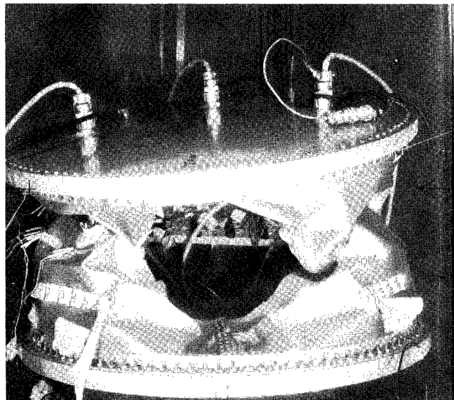
(f) Collapse. Pressure immediately before collapse, 29.8 psi ( 206 \text{ kN/m}^2 ).
