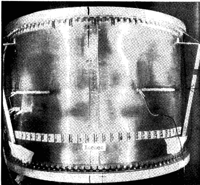
(b) Cylinder immediately after first buckling. (Note one line of light is curved.) Pressure, 17.6 psi (121 kN/m 2 ).
