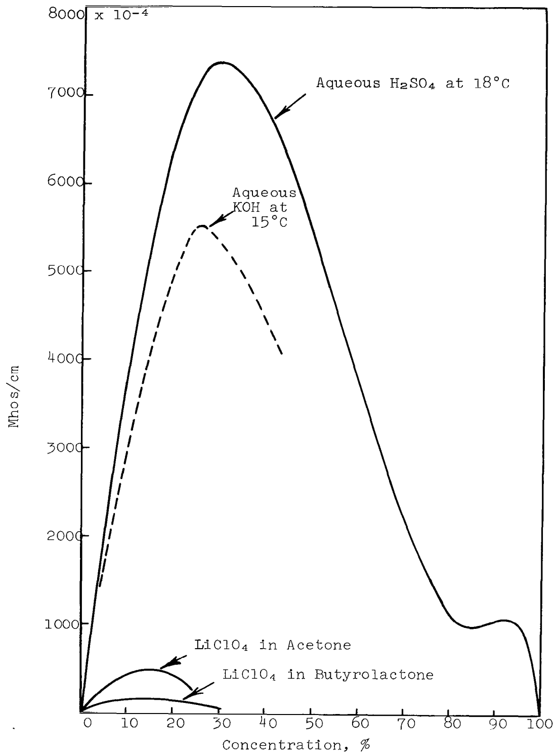
Figure 44. Specific Conductance of Aqueous and Nonaqueous Electrolytes
