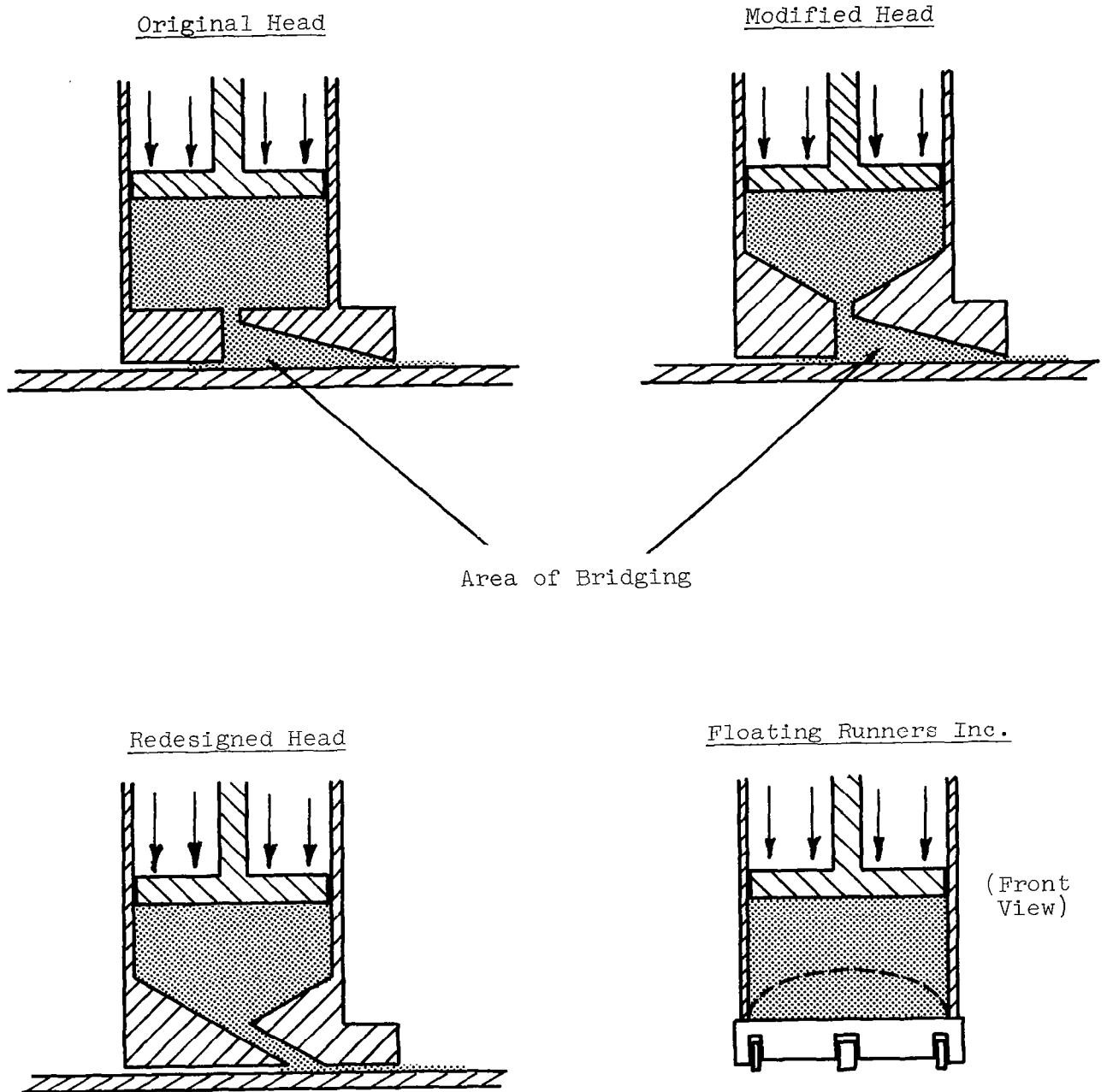
Figure 52. Schematic of Slurry Extrusion Dies
