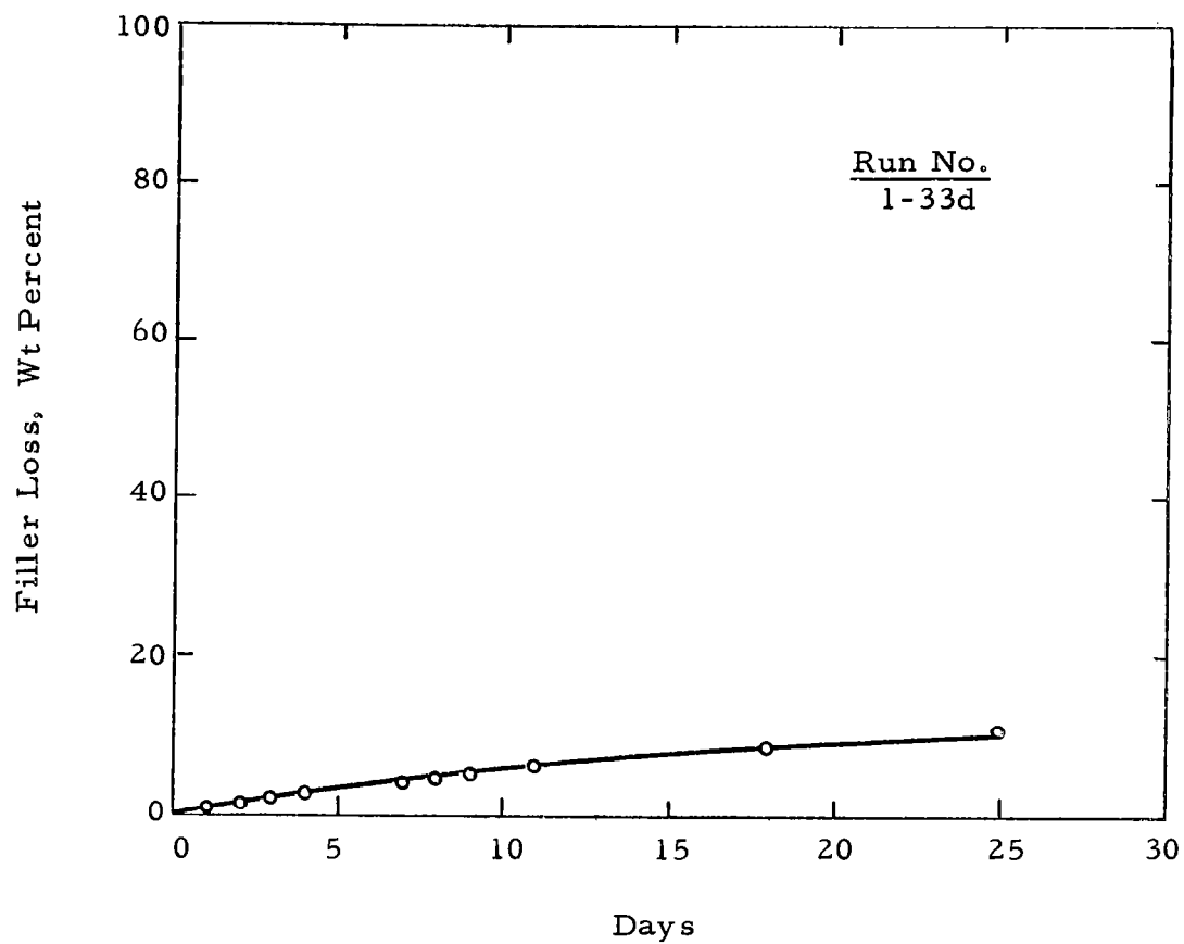
FIGURE 5 STORAGE TEST ON ENCAPSULATED AQUEOUS 2M LiCl-SURFACTANT MIXTURE USING HOT MELT
