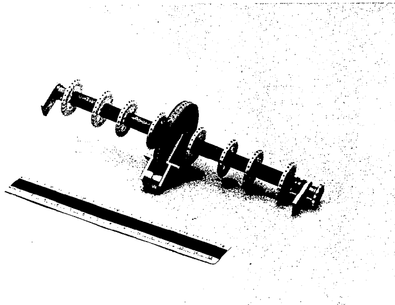
Figure 69. Capstan Drive Assembly
