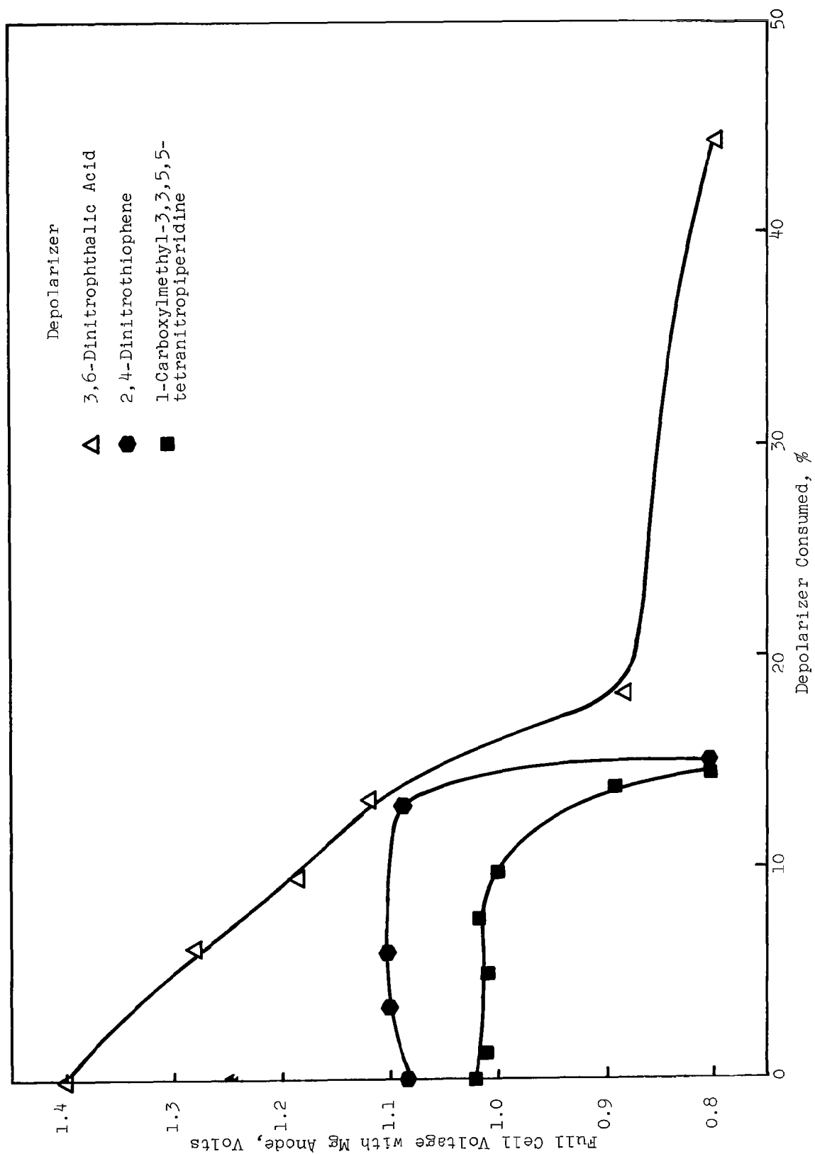
Figure 20. Static Discharge of Various Depolarizers in 2M \text{Mg}(\text{ClO}_4)_2 at 100 mA/in. 2
