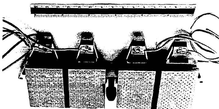
Figure 66. Anode Current Collector
