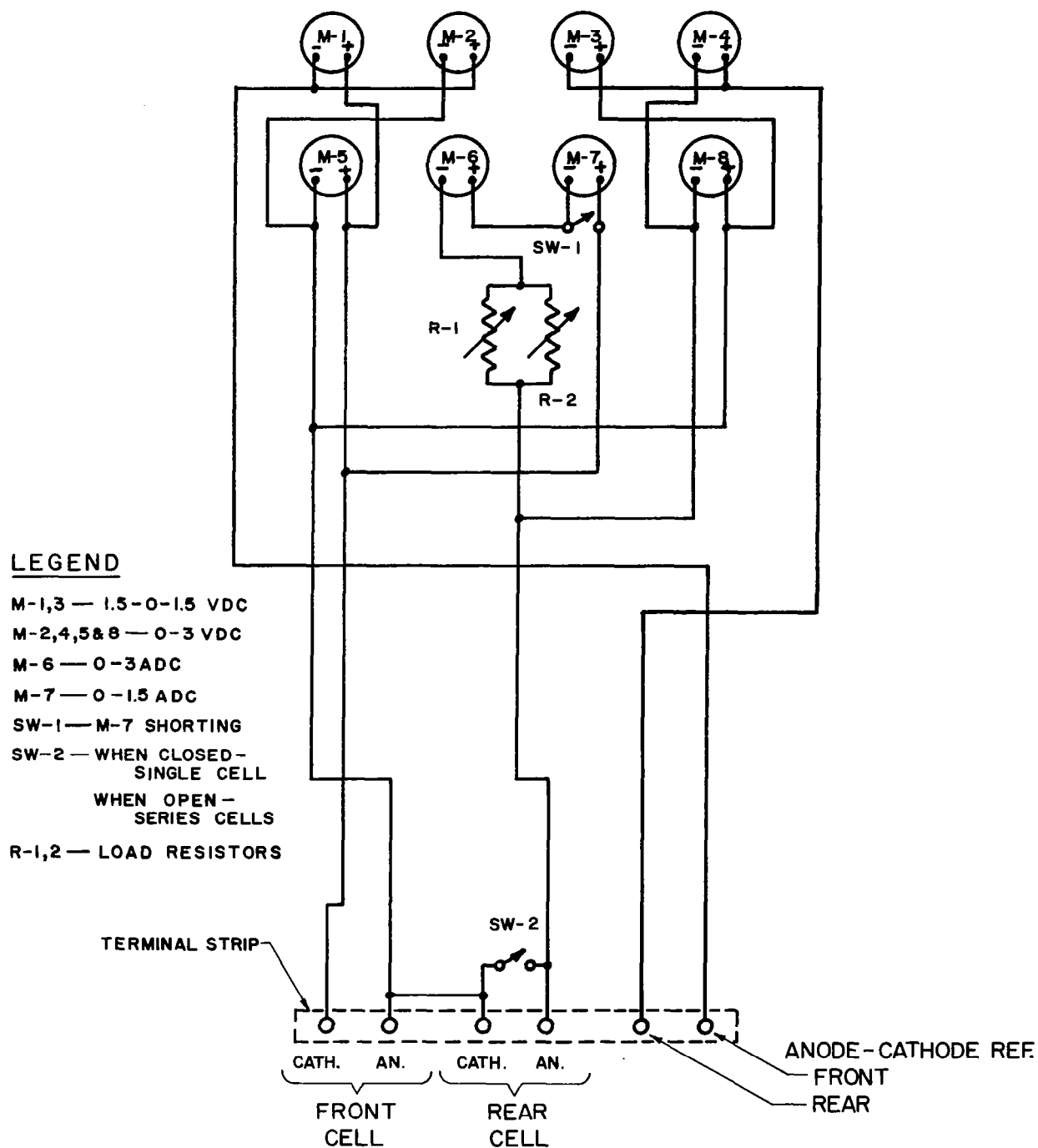
Figure 57. Dry Tape Discharge Circuit
