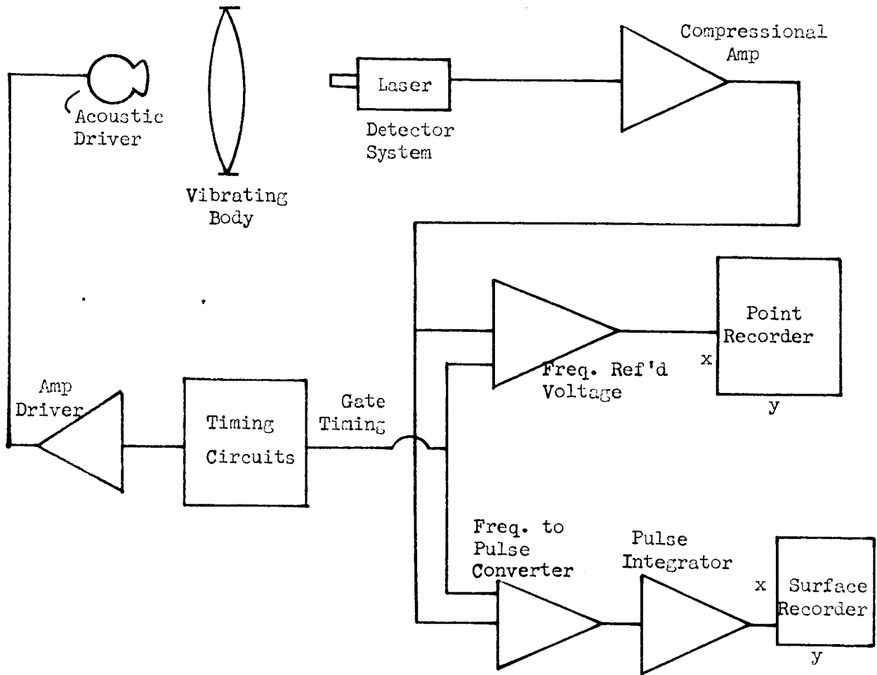
Figure 2 BASIC POINT BY POINT SYSTEM
