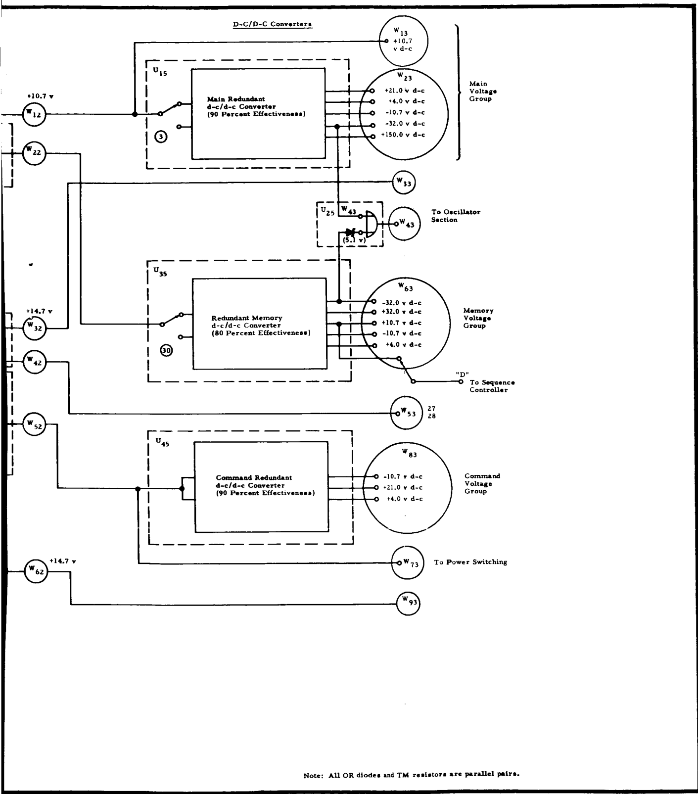
GEOS A POWER SUPPLY
