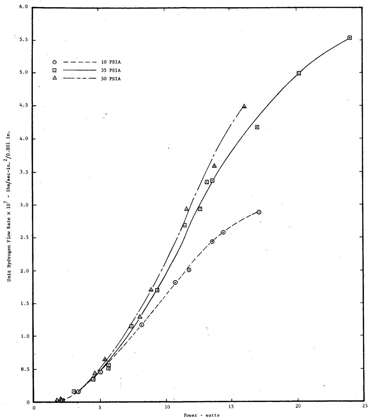
EFFECT OF DC POWER INPUT ON HYDROGEN FLOW RATE AT INDICATED PRESSURE DIFFERENTIALS ACROSS A 34-INCH DIFFUSION ELEMENT (13)
