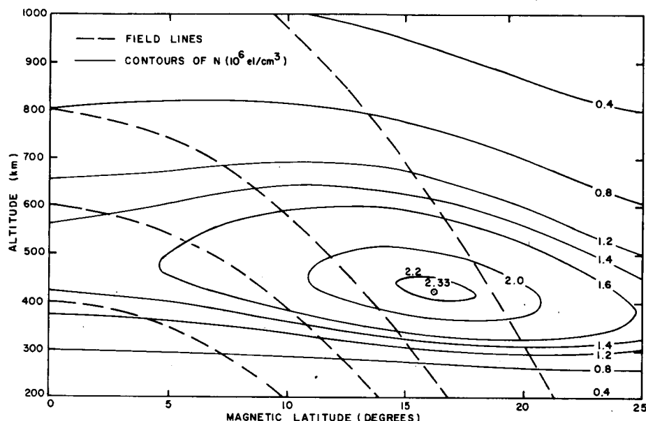
Figure 3 - Sunspot maximum conditions: T_i = T_e/2 = 1500^\circ\text{K} . At 400 km: P = 1.8 \times 10^2 \text{ cm}^{-3}\text{sec}^{-1} , \beta = 8.0 \times 10^{-5} \text{ sec}^{-1} , D_a = 1.3 \times 10^{11} \text{ cm}^2\text{sec}^{-1} , n(0) = 2 \times 10^8 \text{ cm}^{-3} , v_o = 10 \text{ m/sec} independent of altitude.
