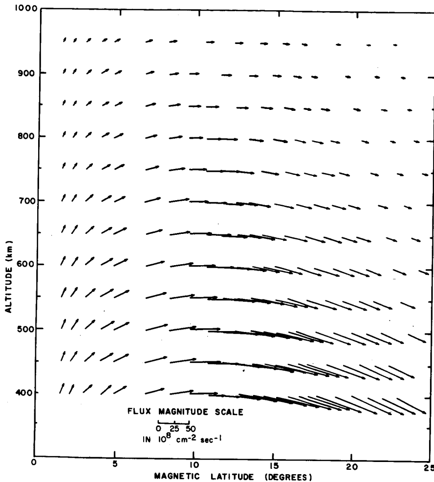
Fig. 4 - Sunspot maximum conditions:
