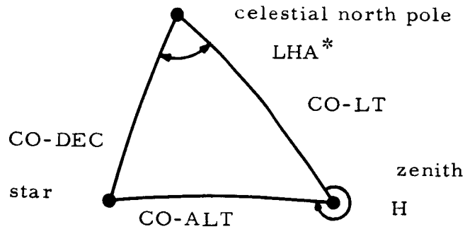
Figure 6 Astronomical Triangle
